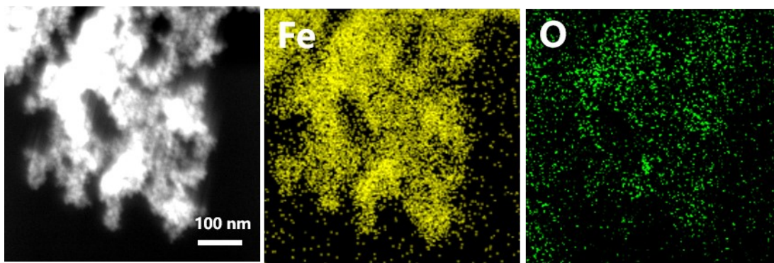
Figure S1. High-angle annular dark field image of CMNP and elemental mappings of Fe and O elements.
