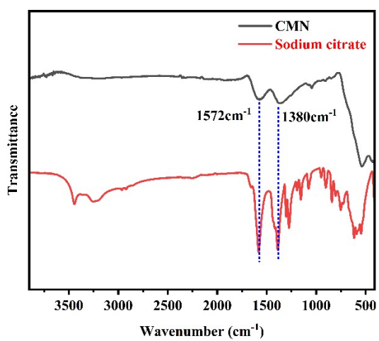
Figure S3. Fourier transform infrared spectroscopy of CMNP and sodium citrate.
