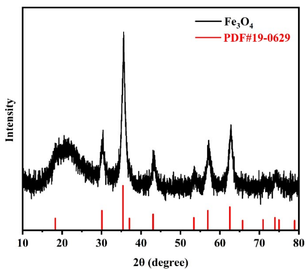
Figure S2. XRD patterns of CMNP and Fe 3 O 4 (JCPDS card no. 19-0629).
