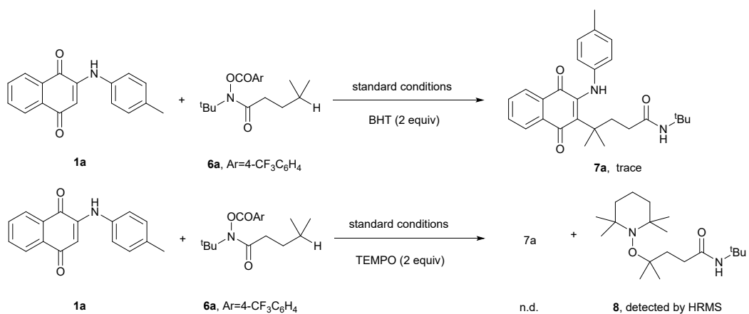
Scheme S2 Control Experiments
