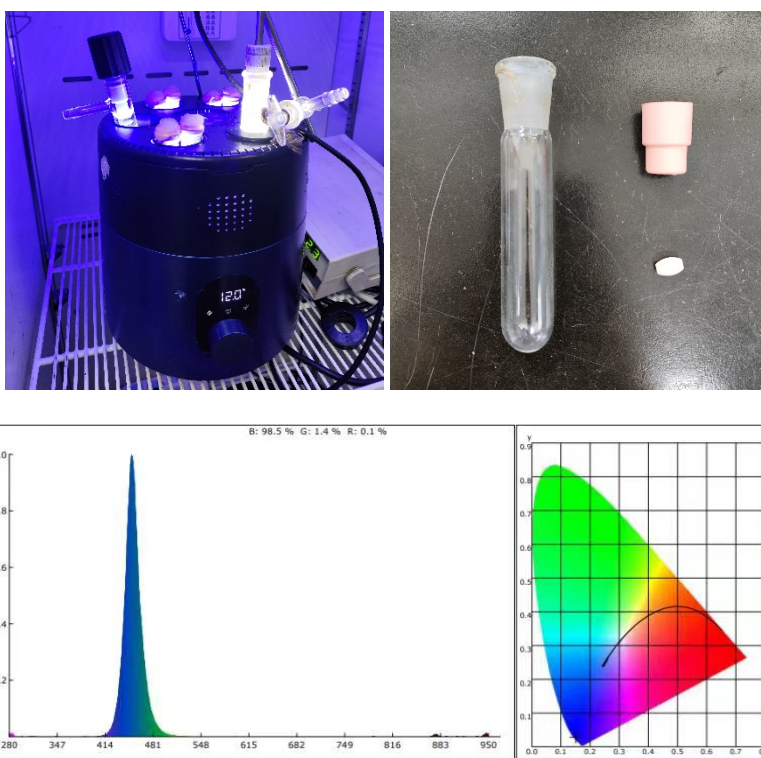
Figure S1. Photo-reactor and the spectrum of our lamp (blue LED)
