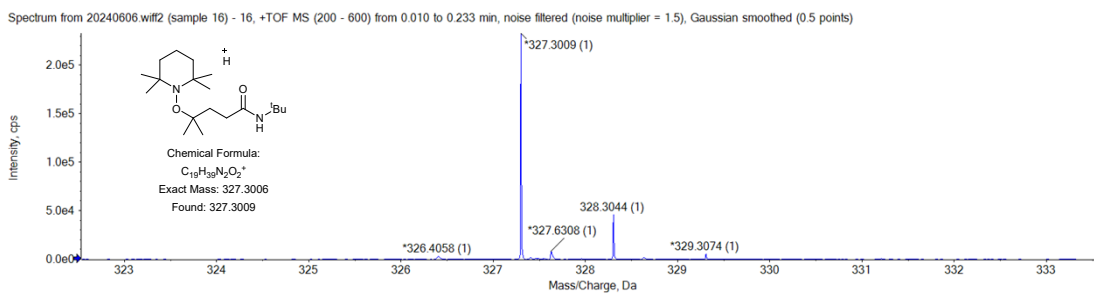
Figure S3. The HRMS spectrum of 8
