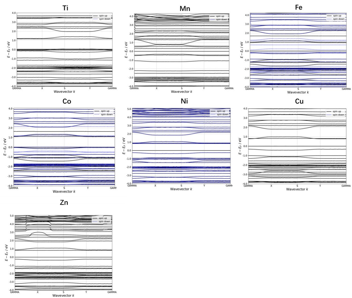
Figure S1. Electronic band structures of MPc COFs (M = Ti, Mn, Fe, Co, Ni, Cu and Zn).
