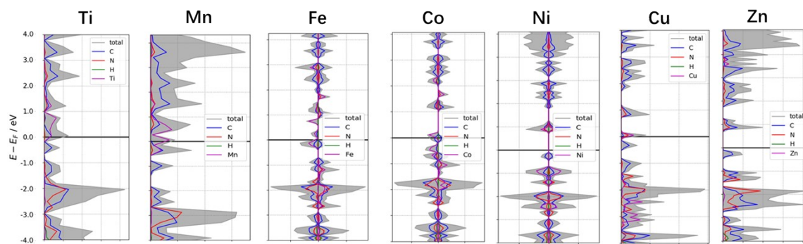
Figure S2. pDOS of MPc COFs (M = Ti, Mn, Fe, Co, Ni, Cu and Zn).
