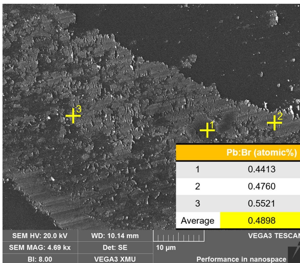
Figure S9. SEM image of degraded n = 2 flakes and EDS analysis at selected points.
