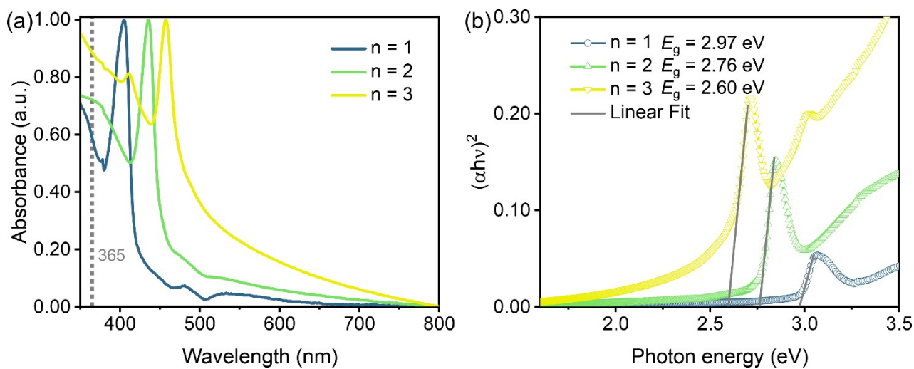
Figure S2. UV-vis spectra of 2D perovskite (\text{BA})_2(\text{MA})_{n-1}\text{Pb}_n\text{Br}_{3n+1} with n = 1, 2, and 3.
