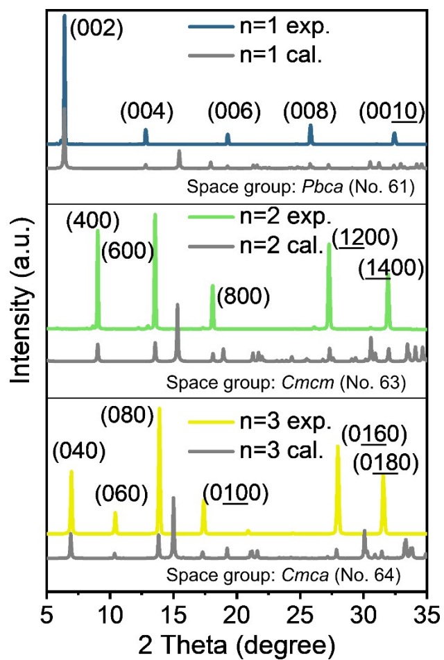
Figure S3. Experimental and calculated XRD patterns for 2D perovskite (\text{BA})_2(\text{MA})_{n-1}\text{Pb}_n\text{Br}_{3n+1} with n = 1^1, 2^2, \text{ and } 3^3 .
