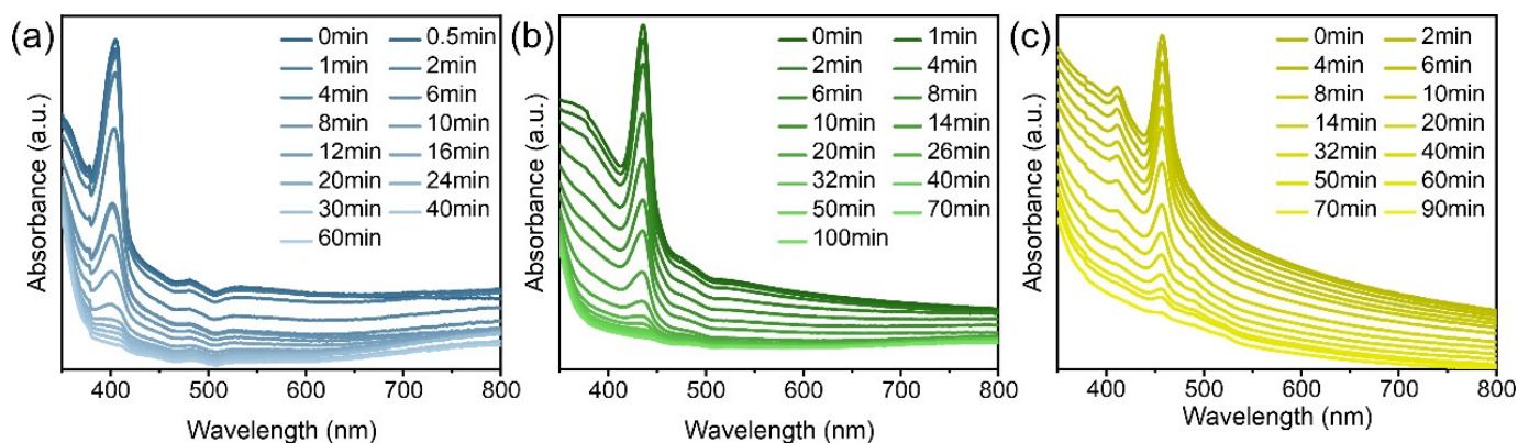
Figure S7. Evolution of UV-Vis absorption spectra of (a) n = 1, (b) n = 2, and (c) n = 3 flakes under UV illumination.
