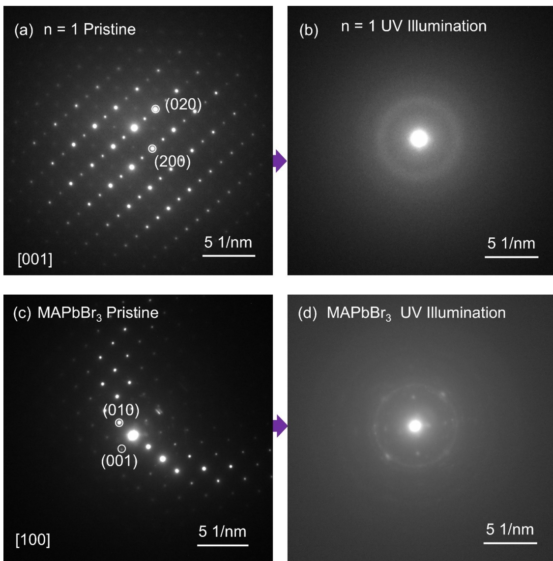
Figure S8. SAED patterns of (a, b) n = 1 and (c, d) \text{MAPbBr}_3 before and after 15 mins of UV exposure.
