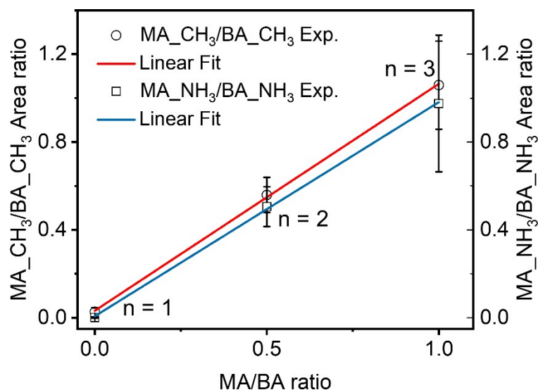
Figure S6. Calibration of Fourier-transform infrared spectroscopy (FTIR) signal by quantifying the MA/BA ratio of n = 1, 2, and 3 flakes based on the area ratios of peaks corresponding to methyl group (circle, -\text{CH}_3 , 1480 \text{ cm}^{-1} ) and amine group (square, -\text{NH}_3 , 1580 \text{ cm}^{-1} ). The linear relationship is obtained for both groups ( -\text{CH}_3 : y = (1.03 \pm 0.02) x + (0.03 \pm 0.01) , R^2 = 0.9997 ; -\text{NH}_3 : y = (0.97 \pm 0.02) x + (0.01 \pm 0.01) , R^2 = 0.9996 ) with the slope \sim 1 . The measured peak area ratios for both methyl and amine groups are approximately the same as the nominal MA/BA ratios in all three compounds, which provides a calibration and validates that the peak area ratio can be used to measure the MA/BA ratio in degraded 2D perovskites.
