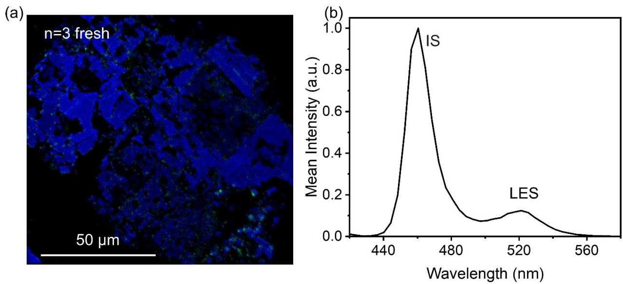
Figure 12. (a) PL image and (b) spectrum of fresh n = 3 flakes.
