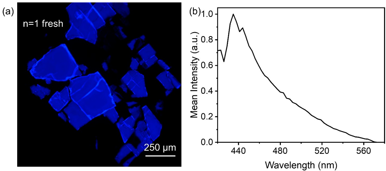
Figure 13. (a) PL image and (b) spectrum of fresh n = 1 flakes. Notably, no low-energy edge peaks, typically associated with green light, are observed for the fresh sample, suggesting that the LES peaks are related to 3D perovskites.
