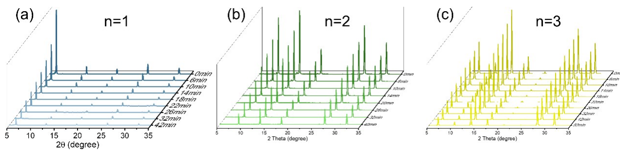
Figure S10. Evolution of XRD patterns from exfoliated n = 1, 2, and 3 flakes under UV illumination.
