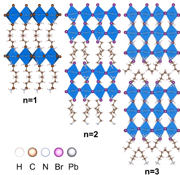
Figure S1. Structural model of 2D perovskite (\text{BA})_2(\text{MA})_{n-1}\text{Pb}_n\text{Br}_{3n+1} with n = 1, 2, and 3.
