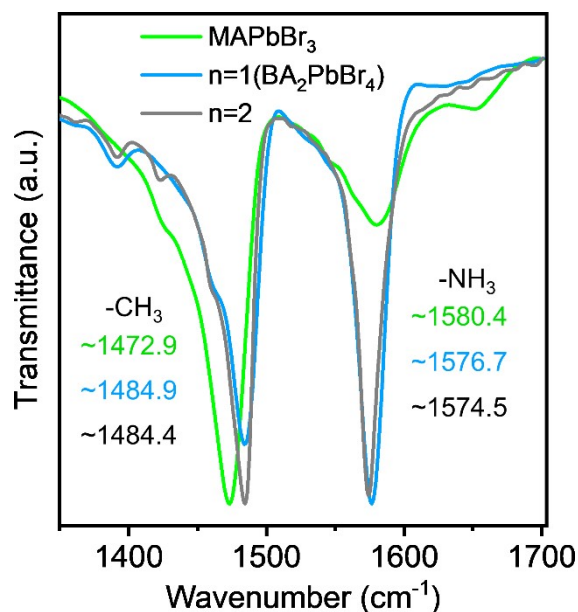
Figure S5. FT-IR spectra of n = 1 (BA 2 PbBr 4 ), n = 2 , and n = \infty (MAPbBr 3 ) flakes with a wavenumber range of 1350 to 1700 cm -1 .
