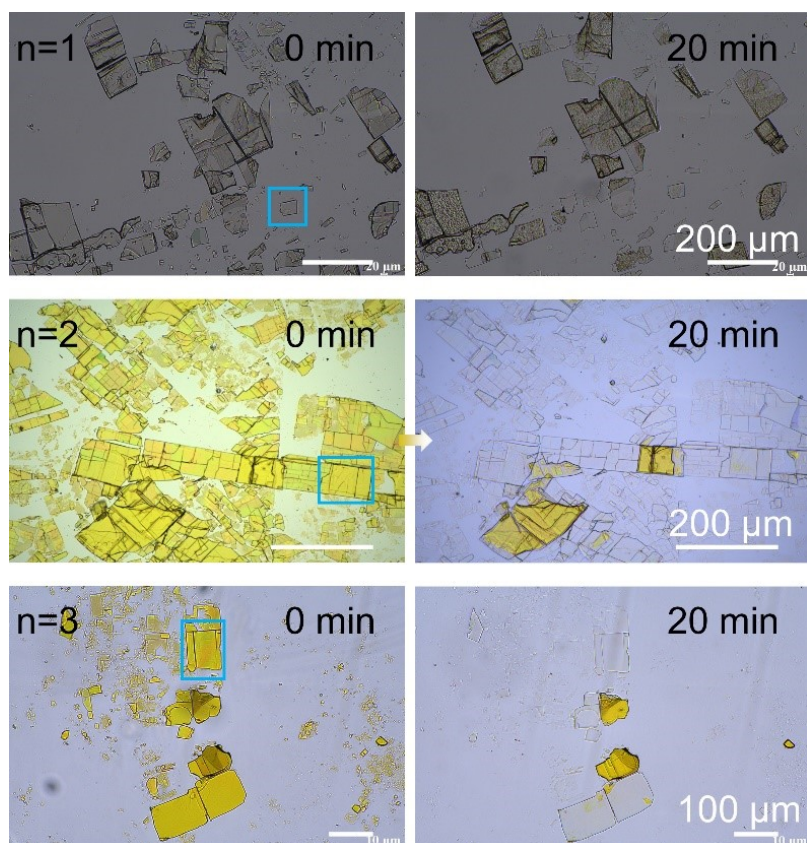
Figure S4. Photographs of n = 1, 2, and 3 flakes which gradually lose their original colors and turn to transparent after 20 mins of UV illumination. The blue boxes indicate the selected regions that are enlarged in Figure 1b. The differences in brightness and contrast observed in the image of initial flakes can be attributed to optical interference caused by variations in the thickness of the exfoliated samples. 4
