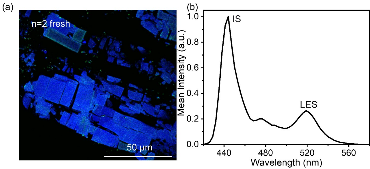
Figure 11. (a) PL image and (b) spectrum of fresh n = 2 flakes.
