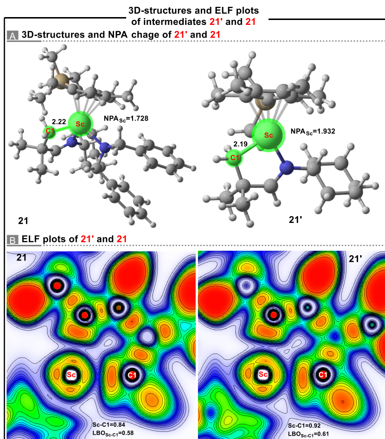
Fig. S8 (A) 3D-structures and (B) ELF analysis of the key intermediates 21 and 21' .
