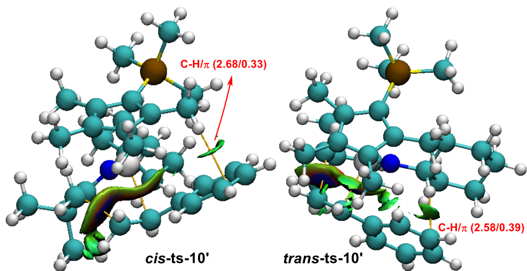
Fig. S10 NCI and AIM analyses for transition states cis -ts-10' and trans -ts-10'
