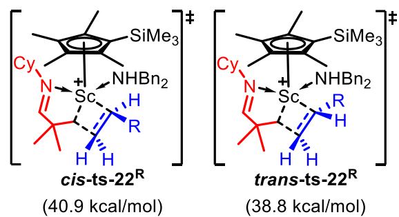
Fig. S7 Structures and Gibbs free energy barriers of 2,1-insertion for octene
