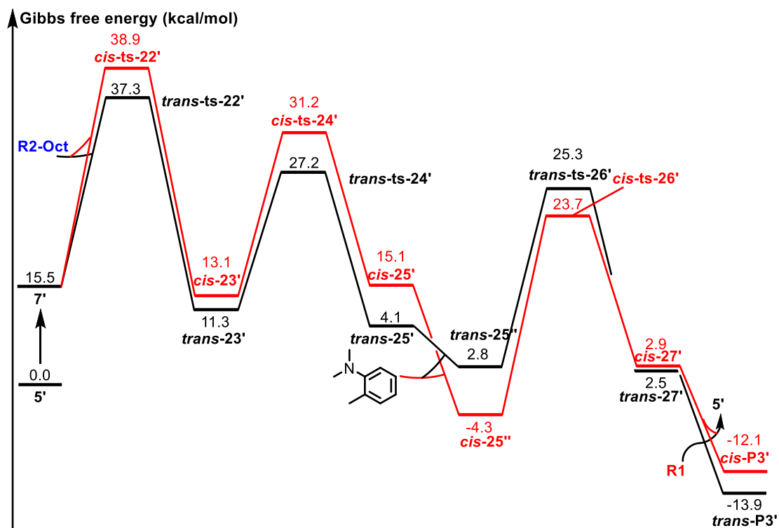
Fig. S6 Energy profile for the reaction between metallacycle intermediate 7' and R2-Oct in the absence of Bn 2 NH
