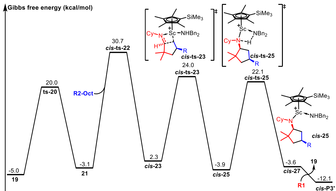
Fig. S5 Energy profiles for the formation of product cis -P3'
