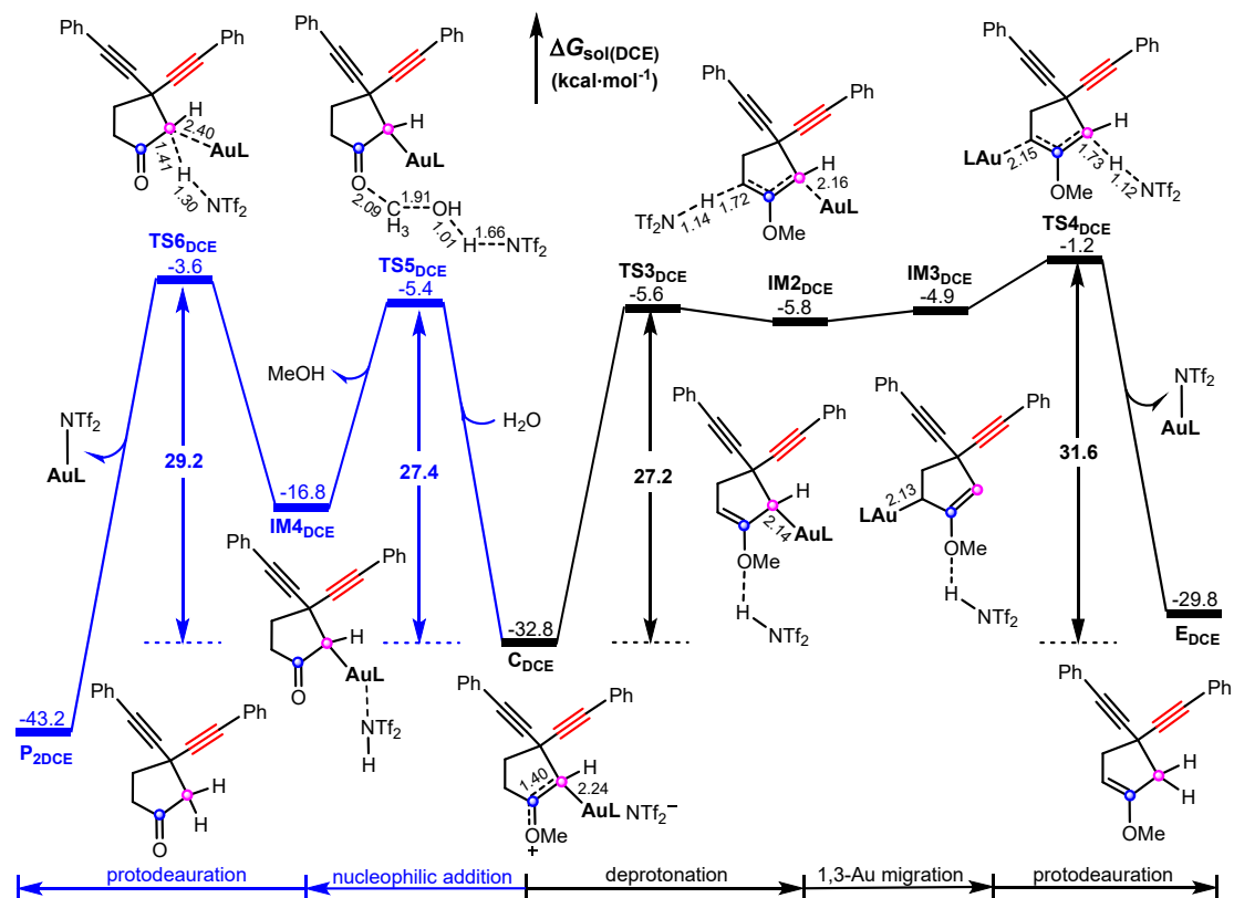
Fig. S5 Calculated free energy profiles for the formation of cyclopentene E DCE (the right profile) and cyclopentanone P 2 DCE (the left profile) in DCE solvent. Bond distances (black values) are in Å.
