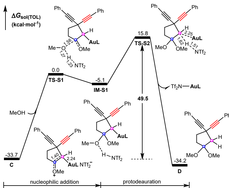
Fig. S2 Calculated free energy profile for the formation of cyclopentane D. Bond distances (black values) are in Å.
