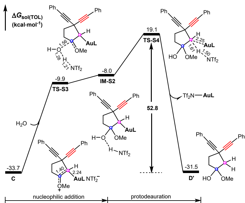
Fig. S3 Calculated free energy profile for the formation of another cyclopentane D' . Bond distances (black values) are in Å.
