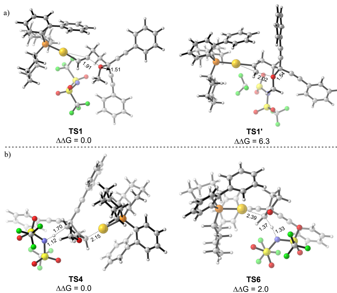
Fig. S6 Optimized geometries and calculated the relative Gibbs free energies for (a) the regioselectivity-determining transition states (TS1 and TS1') and (b) the chemoselectivity-determining transition states (TS4 and TS6). Bond distances are in Å. Gibbs energies are in kcal mol -1 .
