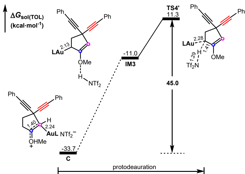
Fig. S4 Calculated free energy profile for the protodeauration process at the C 5 position in IM3 . Bond distances (black values) are in Å.
