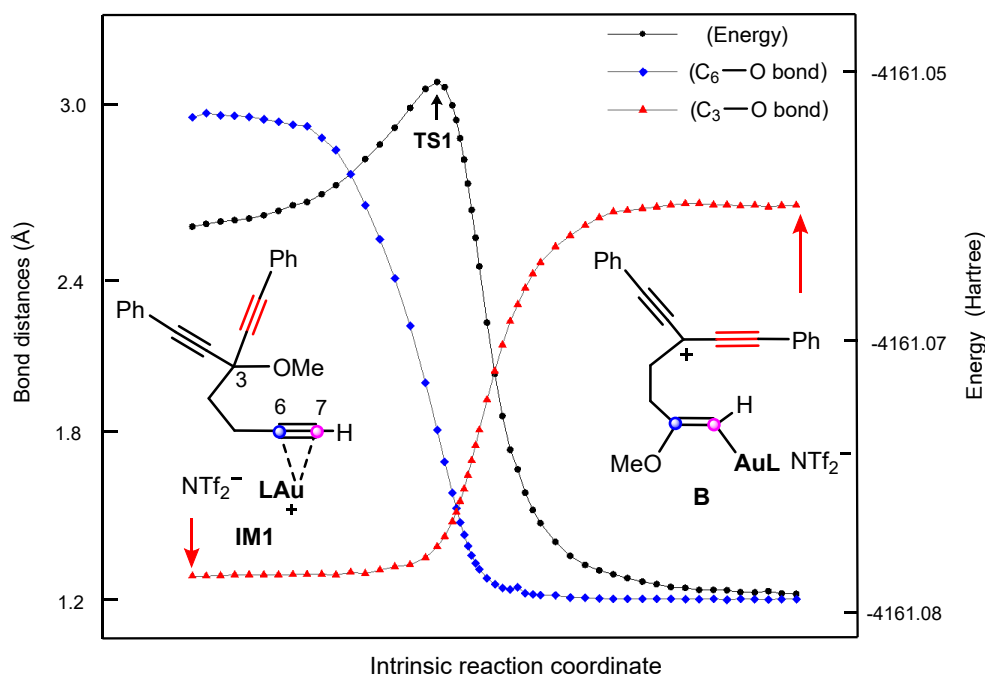
Fig. S1 IRC calculation results for transition state TS1.
