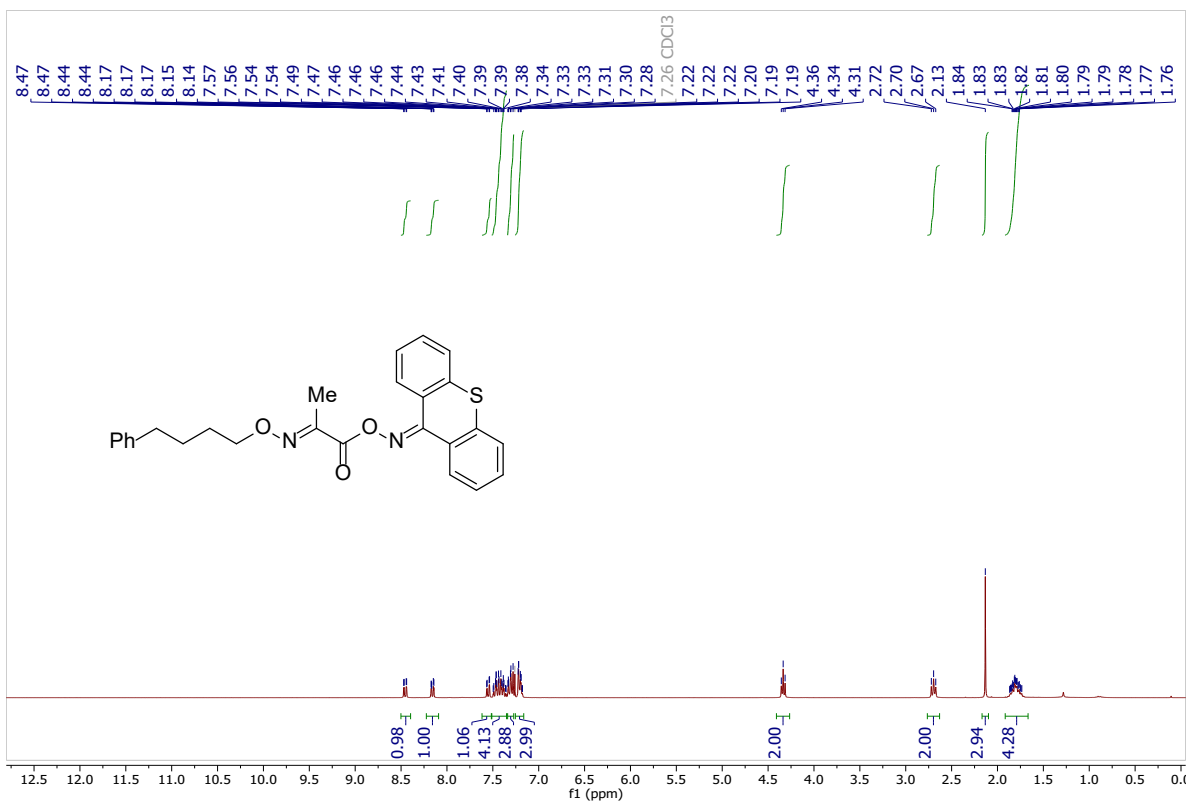
1 H NMR (300 MHz, CDCl 3 ) of compound 1b .
