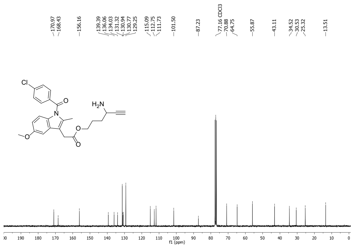
13 C NMR (75 MHz, CDCl 3 ) of compound 6.
