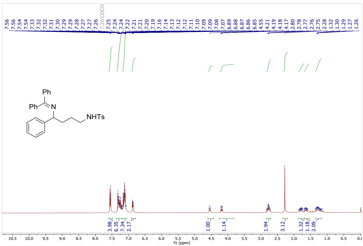
1 H NMR (300 MHz, CDCl 3 ) of compound 2u .
