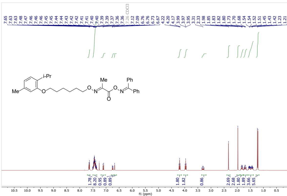
1 H NMR (300 MHz, CDCl 3 ) of compound 1m .
