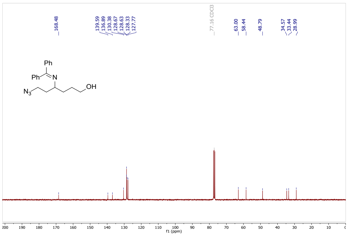
13 C NMR (75 MHz, CDCl 3 ) of compound 21.
