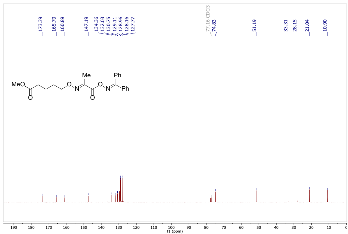
13 C NMR (75 MHz, CDCl 3 ) of compound 1i .
