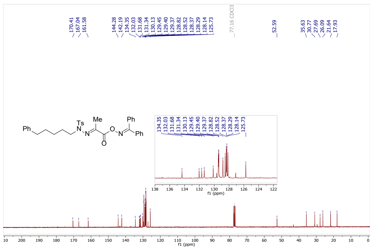
13 C NMR (75 MHz, CDCl 3 ) of compound 1w .
