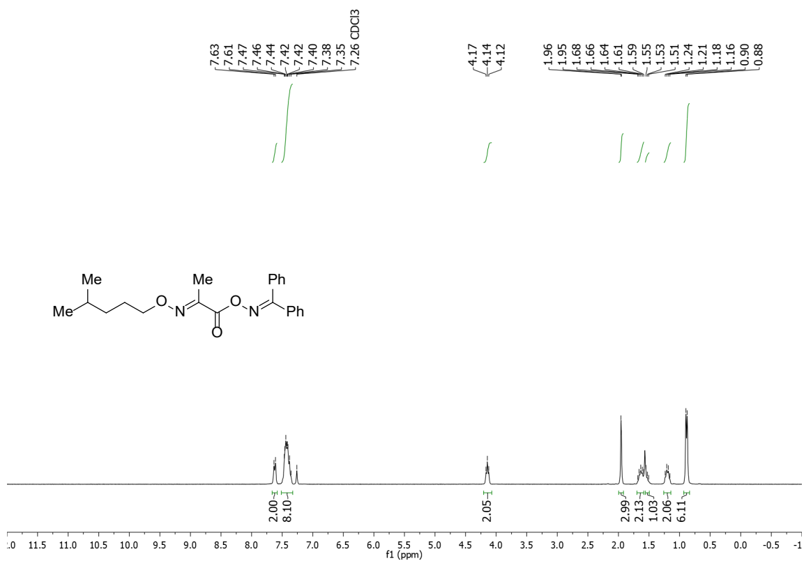
1 H NMR (300 MHz, CDCl 3 ) of compound 1g .
