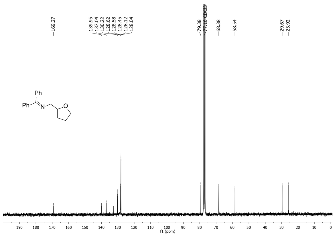
13 C NMR (75 MHz, CDCl 3 ) of compound 2t .
