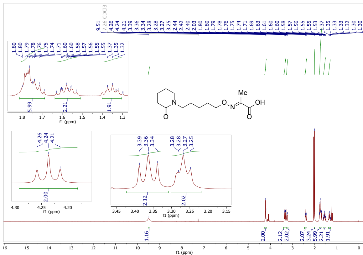
1 H NMR (300 MHz, CDCl 3 ) of compound S2n.
