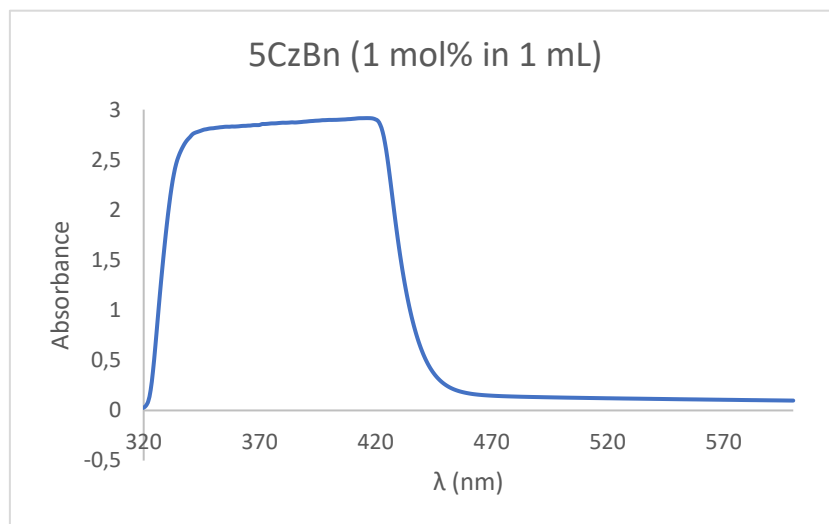
Figure S4. Absorption spectrum of 5CzBn in acetone.
