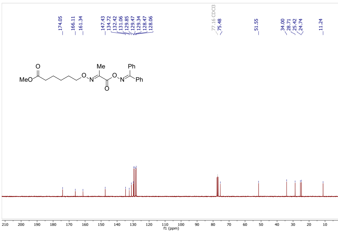
13 C NMR (75 MHz, CDCl 3 ) of compound 1j .
