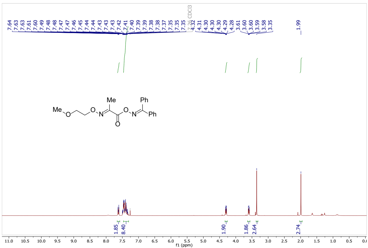
1 H NMR (300 MHz, CDCl 3 ) of compound 1aa .
