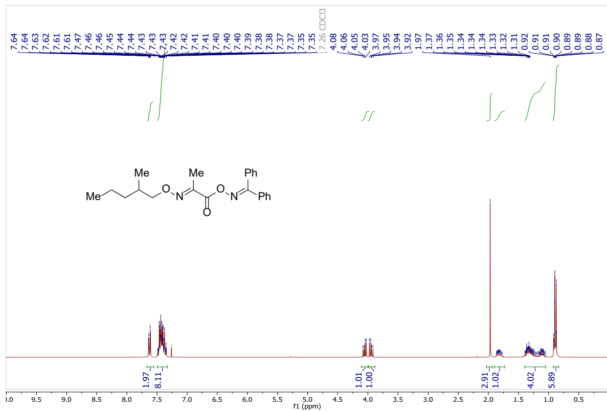
1 H NMR (300 MHz, CDCl 3 ) of compound 1s .
