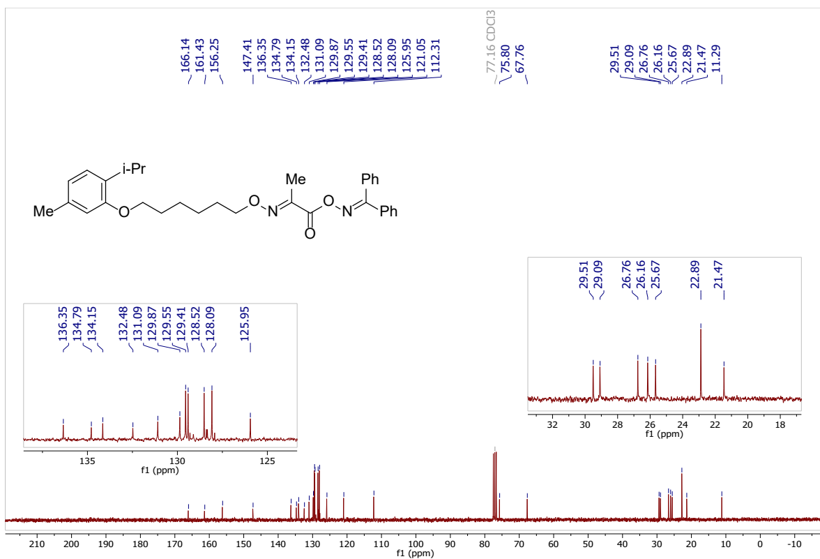
13 C NMR (75 MHz, CDCl 3 ) of compound 1m .
