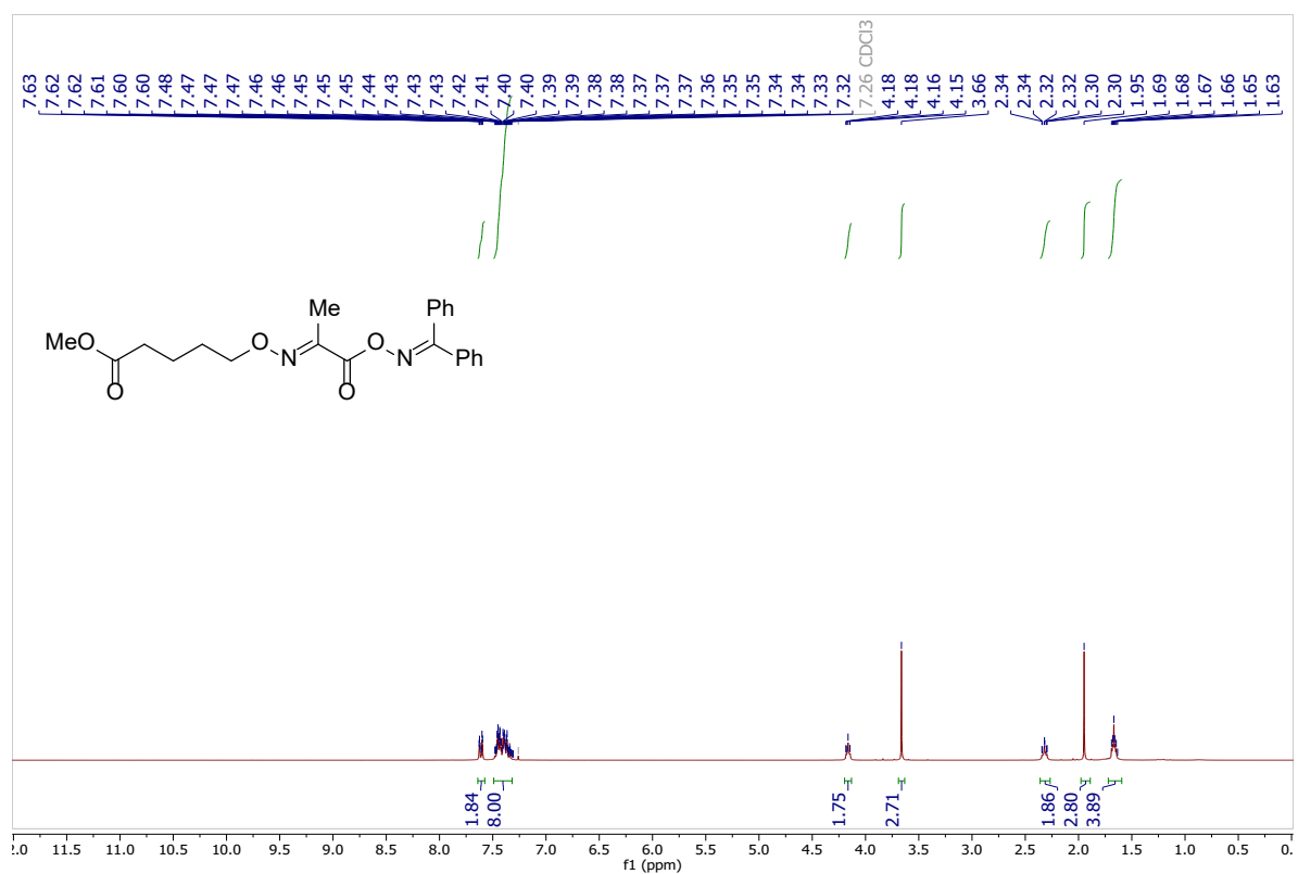
1 H NMR (300 MHz, CDCl 3 ) of compound 1i .
