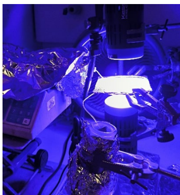
Figure S2. Gram scale synthesis reaction setup of 2a .
