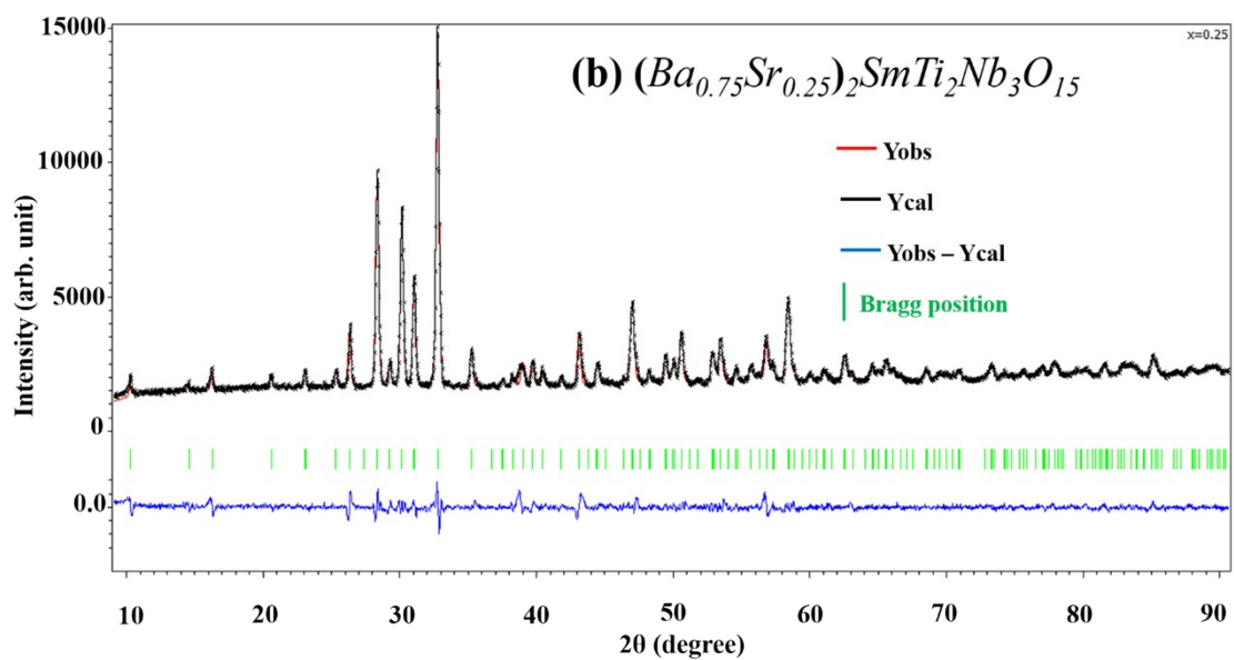
Figure S1: X-ray diffraction refinement for BS_xSTN powder x=0.25 .
