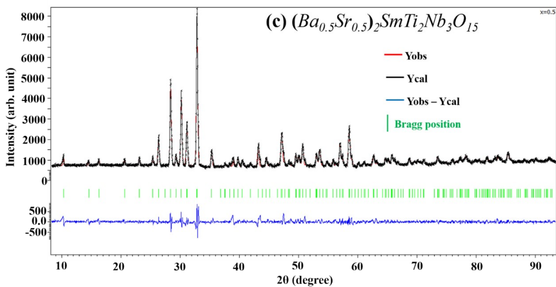
Figure S2: X-ray diffraction refinement for BS_xSTN powder x=0.5 .
