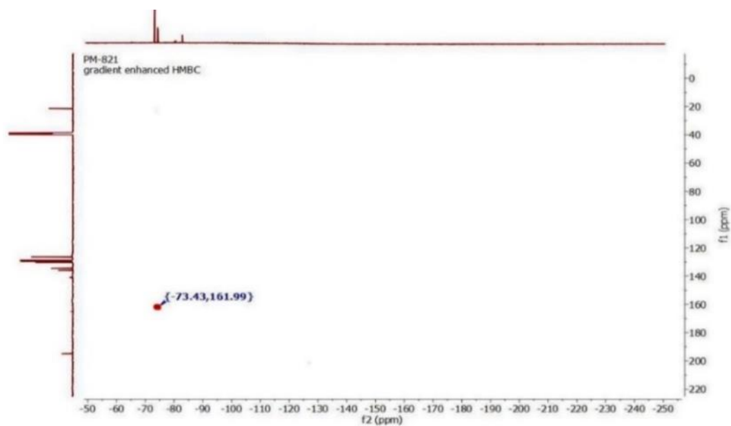
(^{19}\text{F}-^{13}\text{C}) HMBC spectrum of compound 14a
