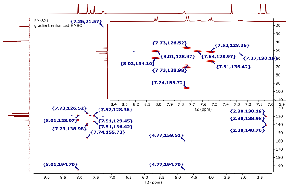
(^{19}\text{F}-^{13}\text{C}) HMBC spectrum of compound 14a
