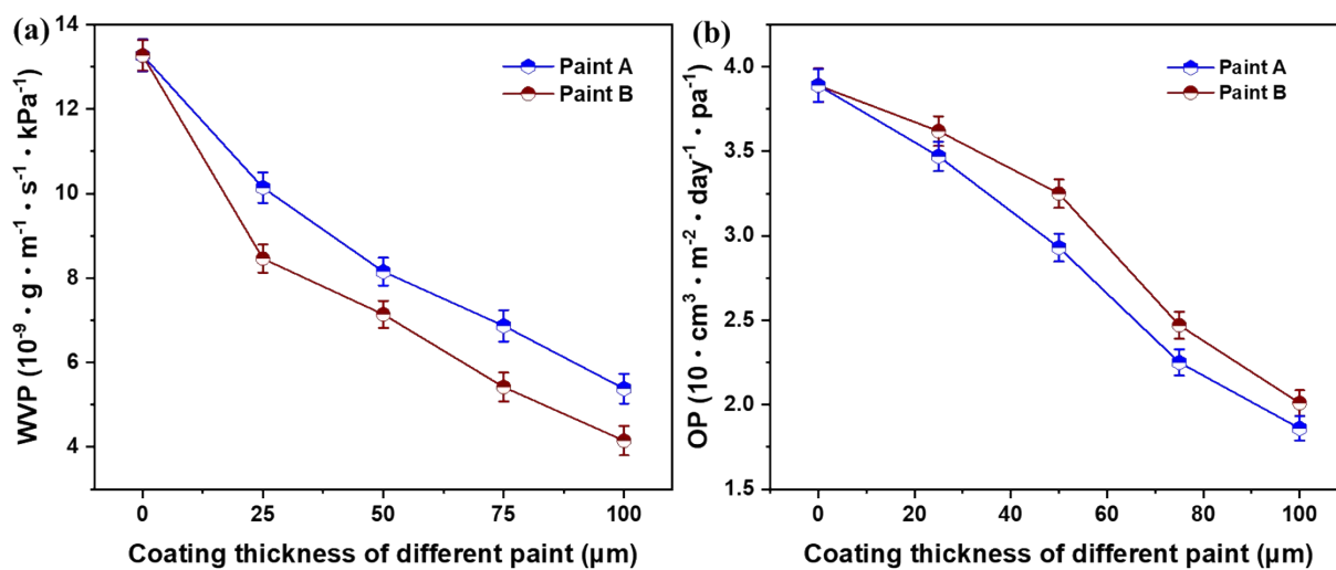
Figure S1. (a) Water vapor permeability of WC respectively coated by paint A or paint B with different coating thicknesses; (b) Gas permeability coefficient of WC respectively coated by paint A or paint B with different thickness.
