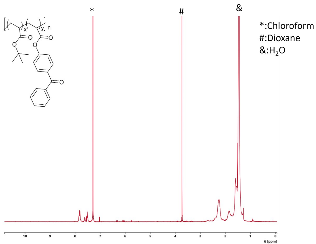
Fig S1. 1 H NMR spectrum of compound poly(BA 95 -BPA 5 ) (CDCl 3 , 400 MHz).
