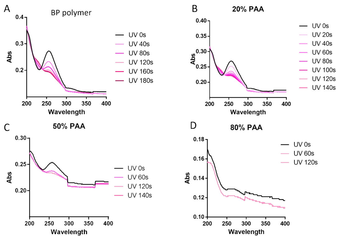
Fig S2. UV vis spectrum of BP-PAA coating with different UV exposure time. (A) Pure BP polymer; (B) 20% PAA + 80% BP; (C) 50% PAA + 50% PAA; (D) 80% PAA + 20% BP
