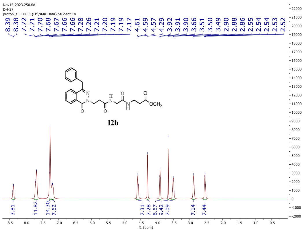
Figure S78: The ^1\text{H} -NMR spectrum of compound 12b
