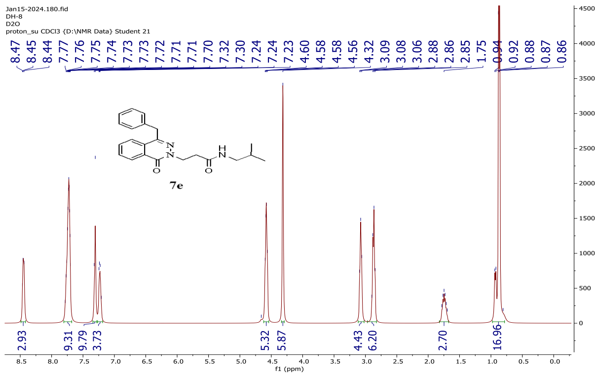
Figure S25 The D2O spectrum of compound 7e
