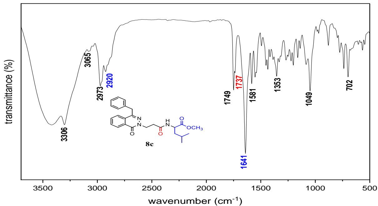
Figure S45 The IR spectrum of compound 8c
