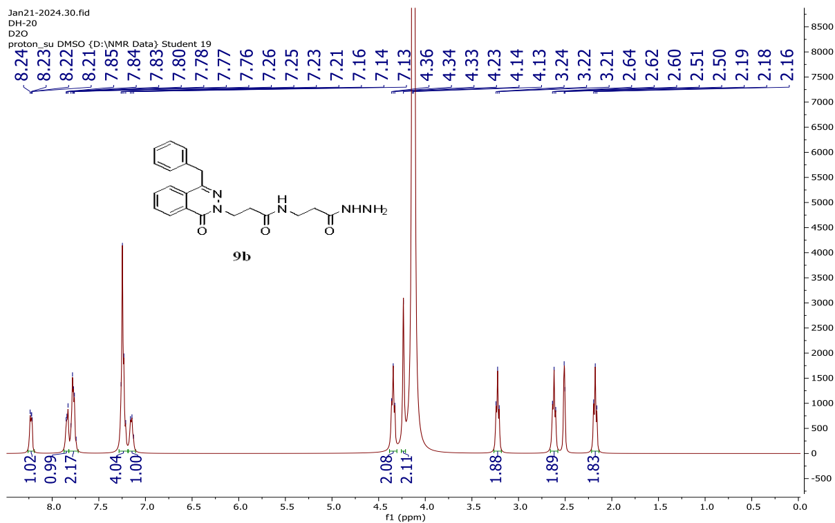
Figure S52 The D 2 O spectrum of compound 9b
