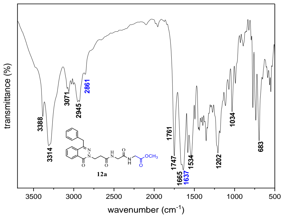
Figure S77: The IR spectrum of compound 12a
