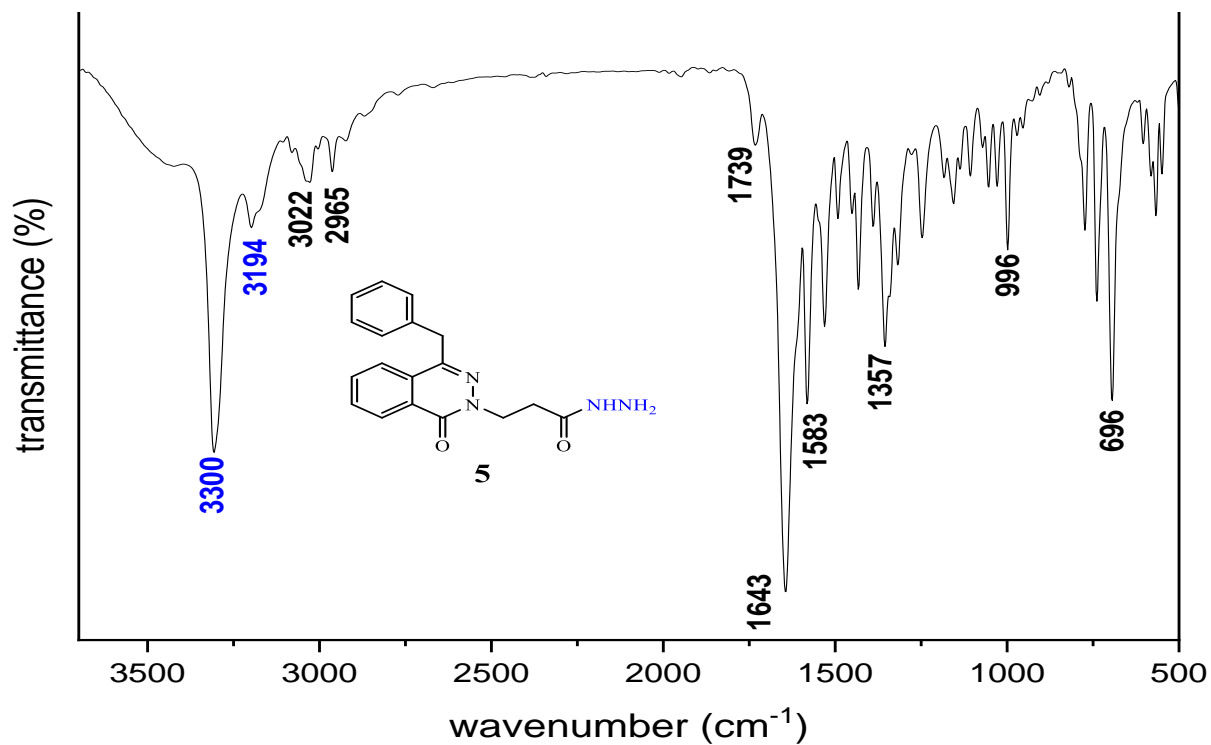
Figure S8 The IR spectrum of compound 5
