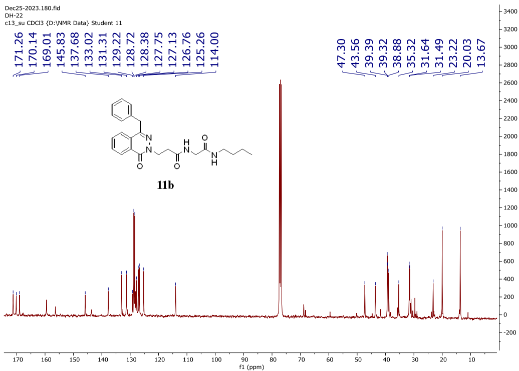
Figure 63: The ^{13}\text{C} -NMR spectrum of compound 11b
