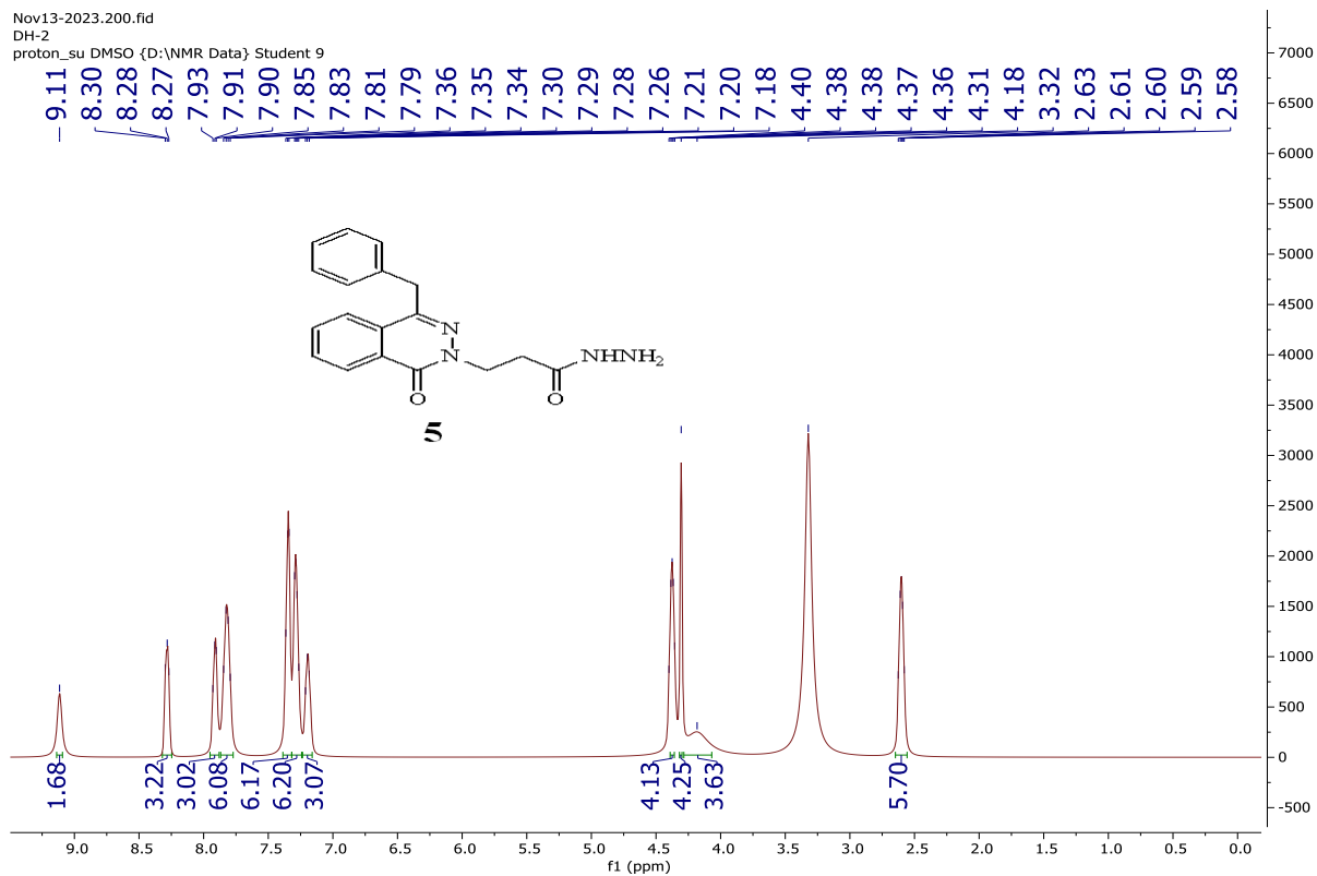
Figure S5 The ^1\text{H} -NMR spectrum of compound 5.
