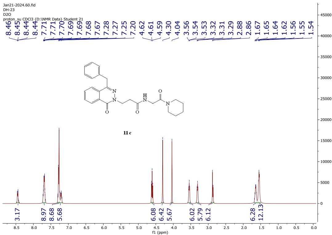
Figure S68: The D2O spectrum of compound 11c
