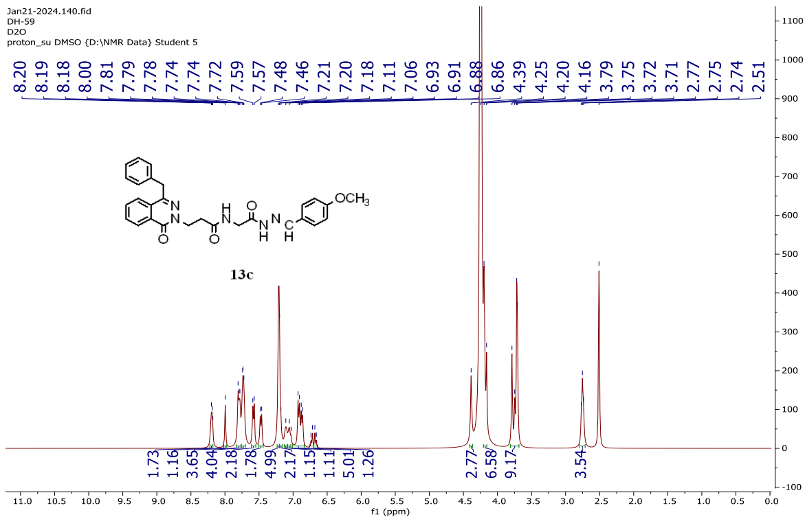
Figure S94: The D2O spectrum of compound 13c
