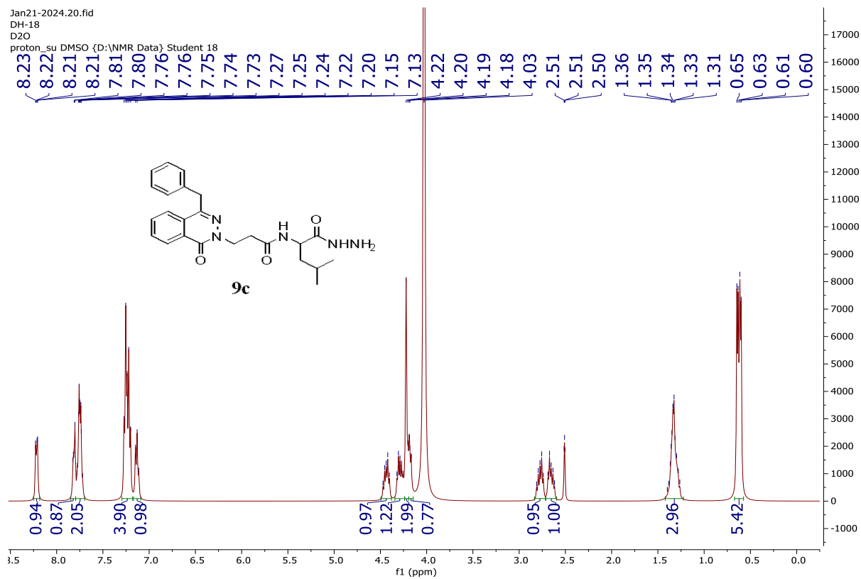
Figure S56 The D 2 O spectrum of compound 9c
