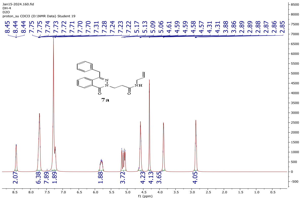
Figure S11 The D2O spectrum of compound 7a
