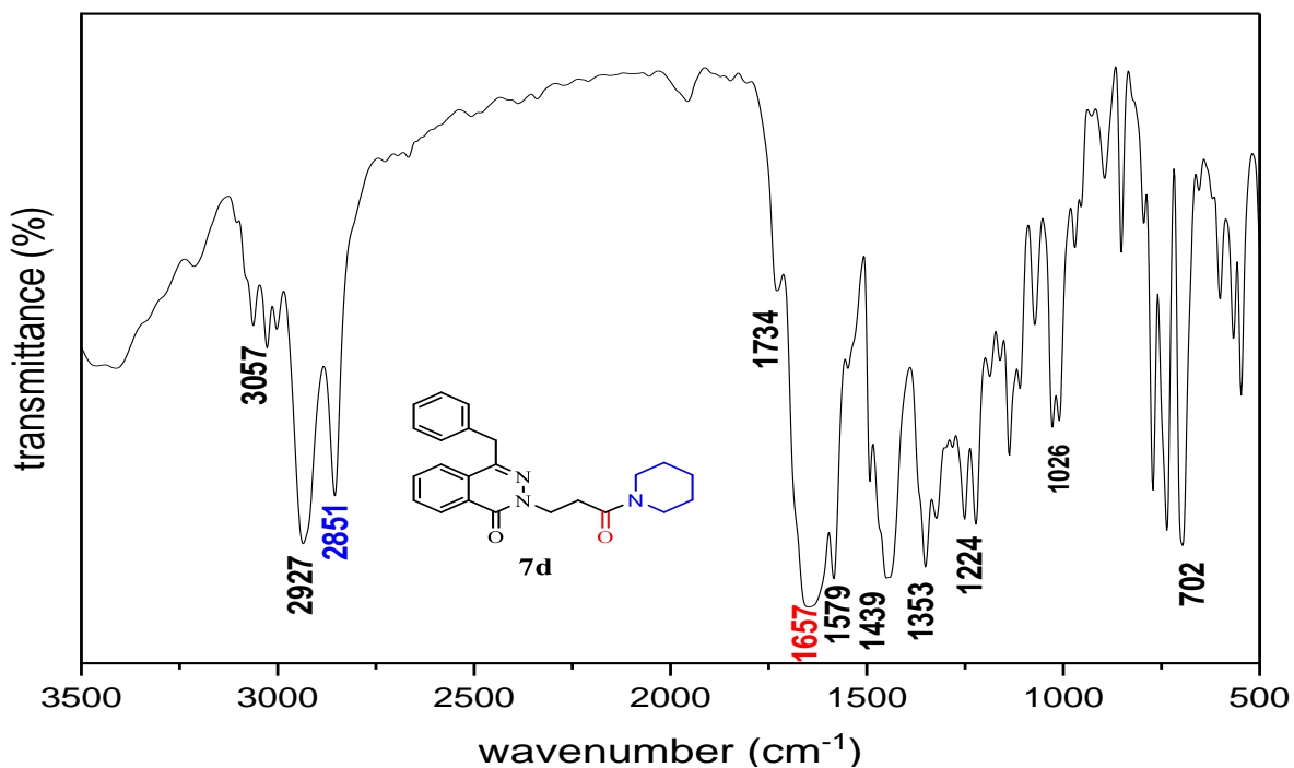
Figure S22 The IR spectrum of compound 7d
