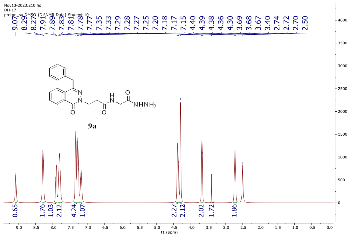
Figure S46 The 1 H-NMR spectrum of compound 9a
