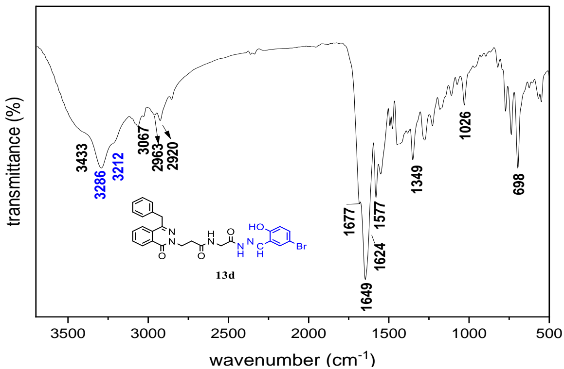
Figure S97: The IR spectrum of compound 13d
