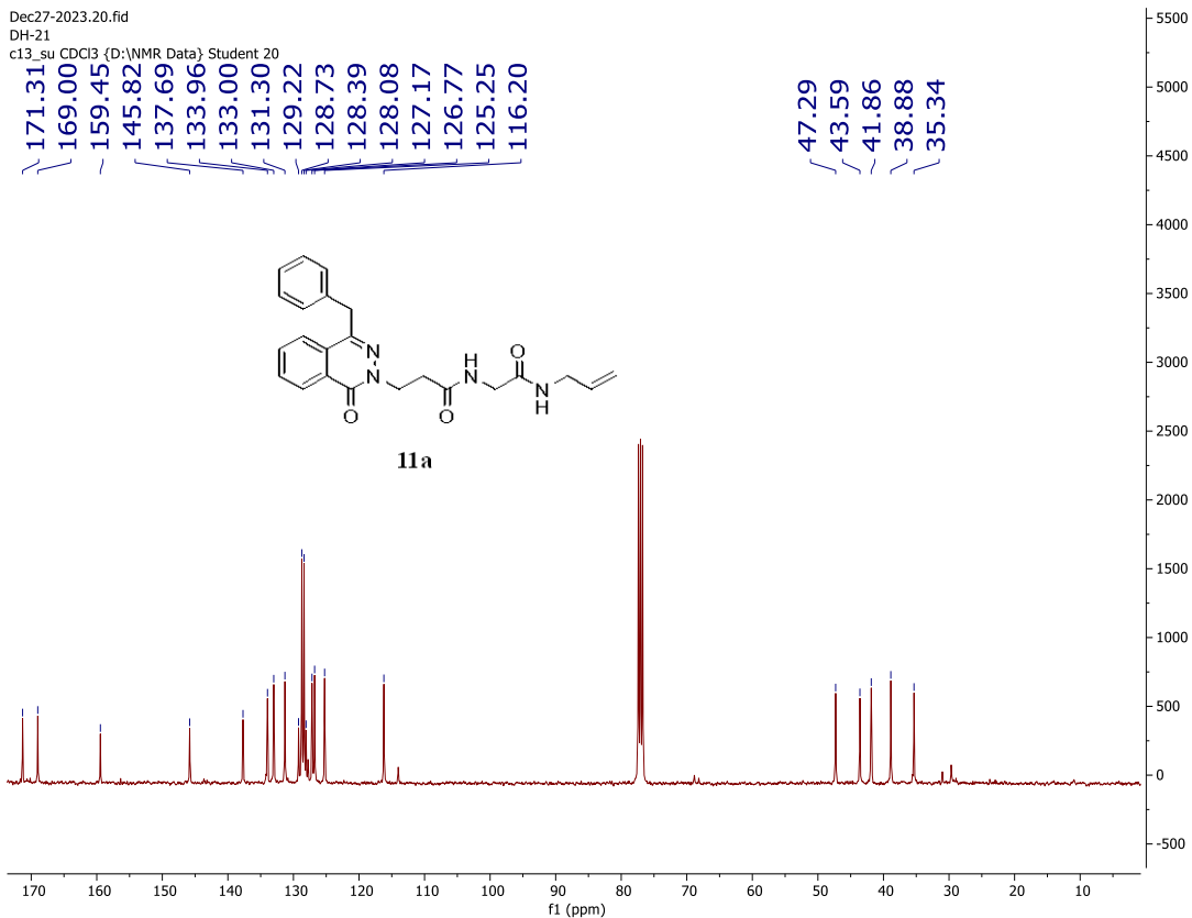
Figure S59: The ^{13}\text{C} -NMR spectrum of compound 11a
