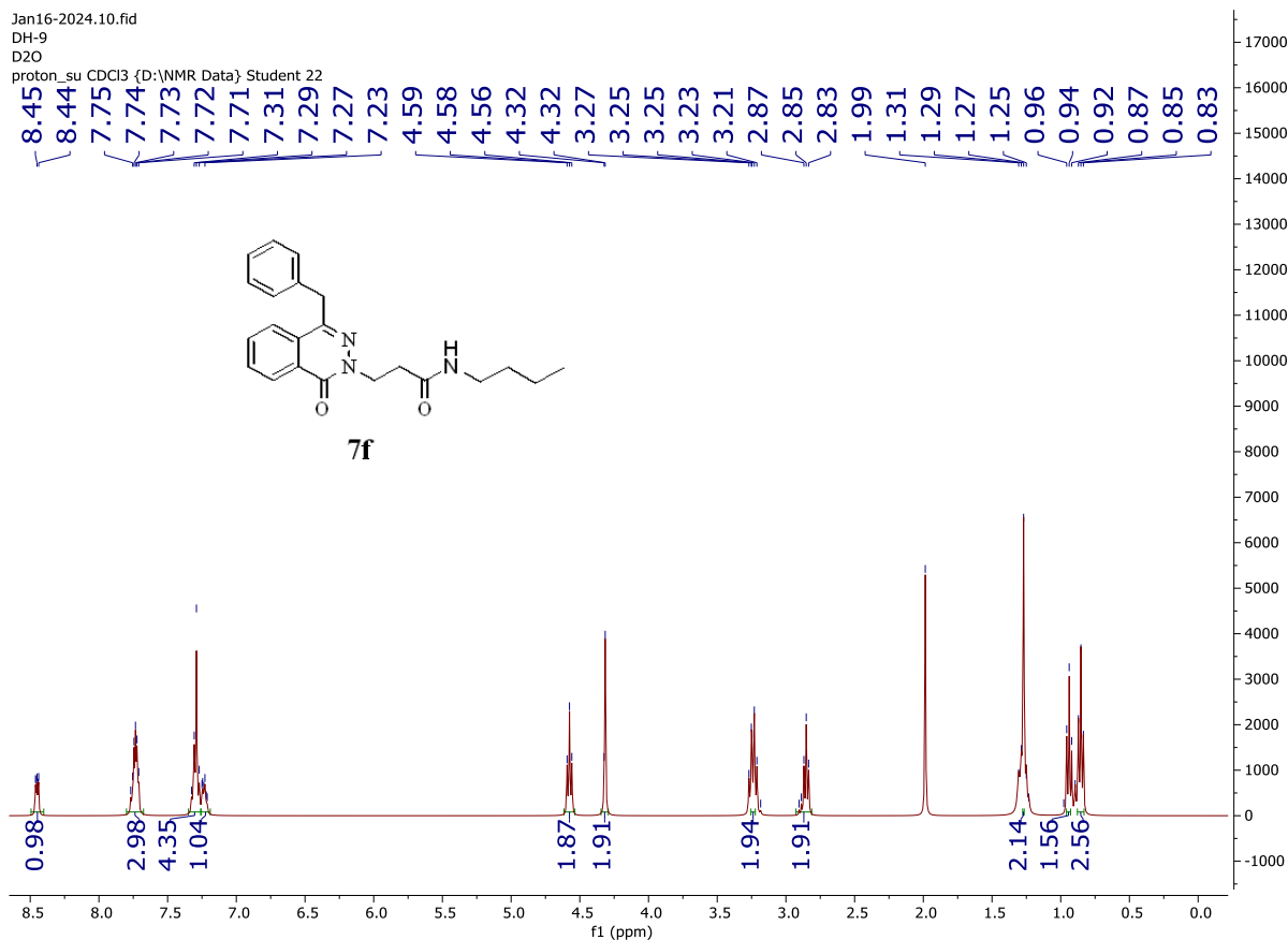
Figure S29 The D2O spectrum of compound 7f
