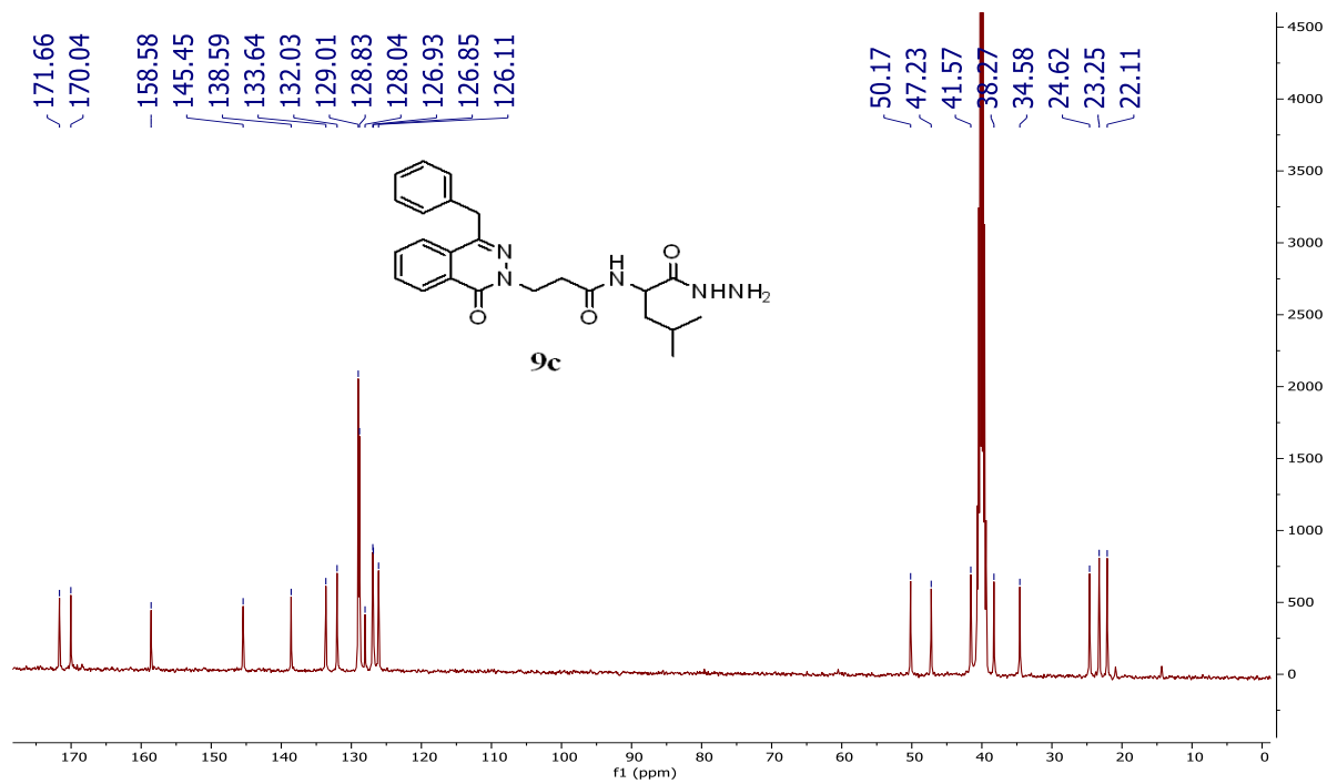
Figure S55 The 13 C-NMR spectrum of compound 9c
