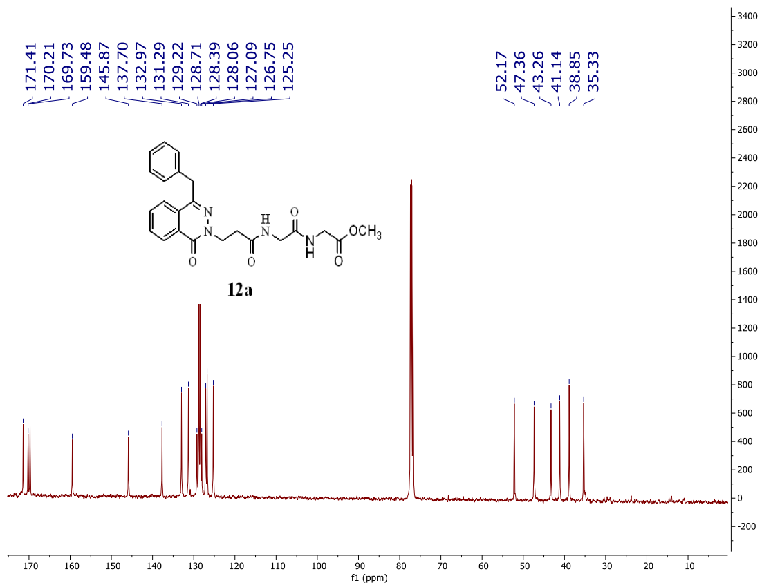
Figure S75: The ^{13}\text{C} -NMR spectrum of compound 12a
