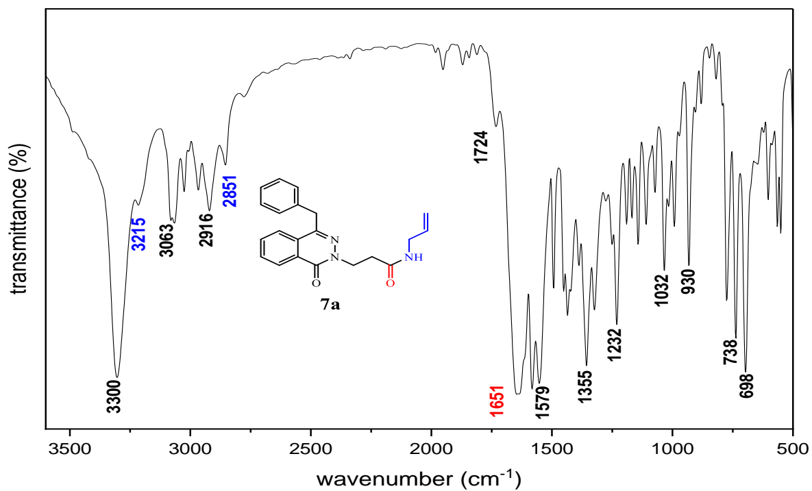
Figure S12 The IR spectrum of compound 7a
