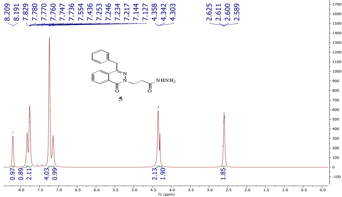
Figure S7 The D2O spectrum of compound 5.
