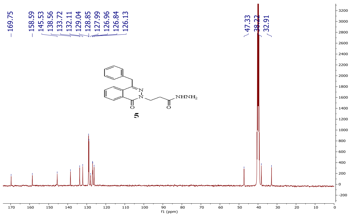
Figure S6 The ^{13}\text{C} -NMR spectrum of compound 5.
