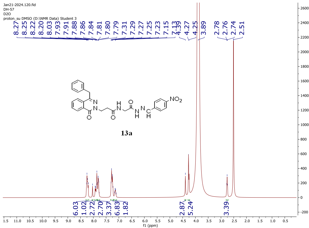
Figure S88: The D2O spectrum of compound 13a
