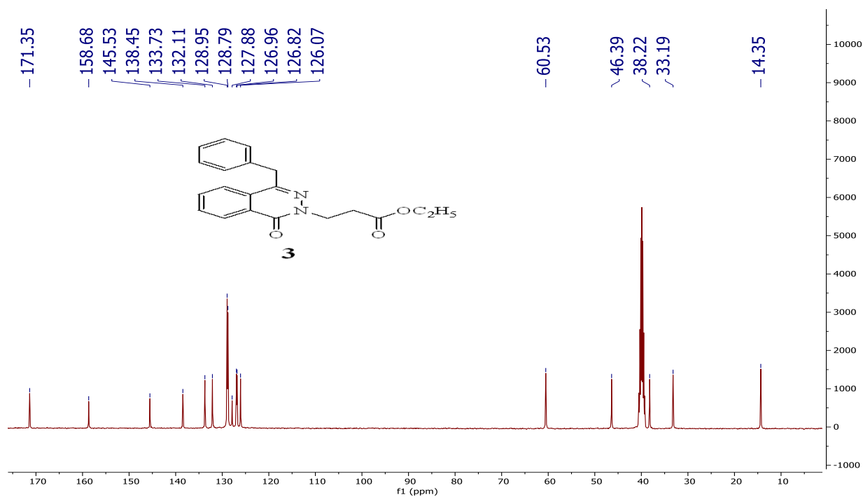
Figure S2 The ^{13}\text{C} -NMR spectrum of compound 3 .
