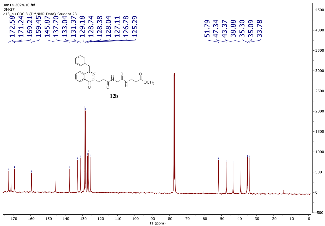
Figure S79: The ^{13}\text{C} -NMR spectrum of compound 12b
