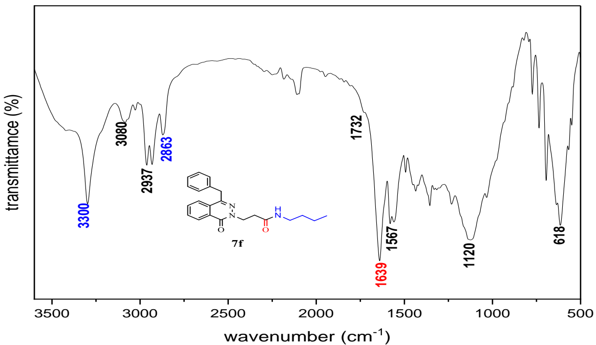
Figure S30 The IR spectrum of compound 7f
