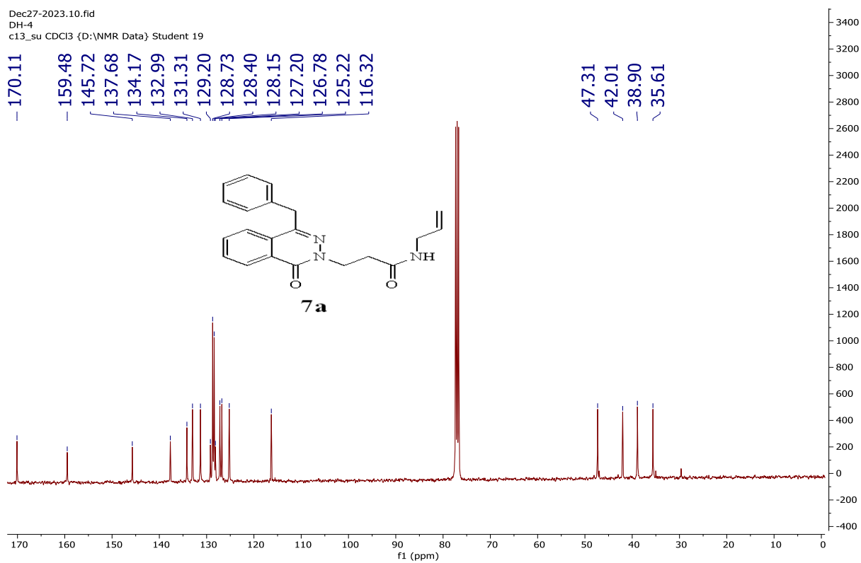
Figure S10 The ^{13}\text{C-NMR} spectrum of compound 7a
