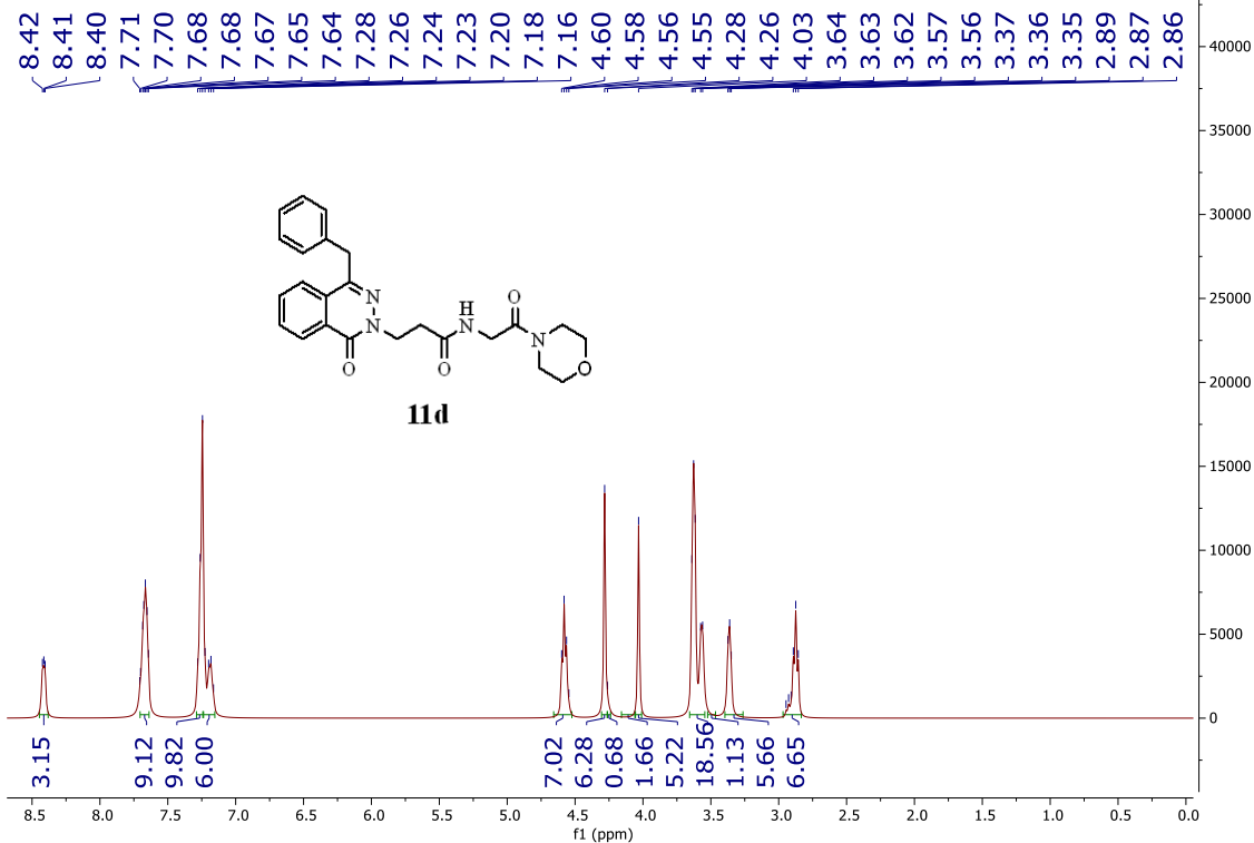
Figure S72: The D2O spectrum of compound 11d
