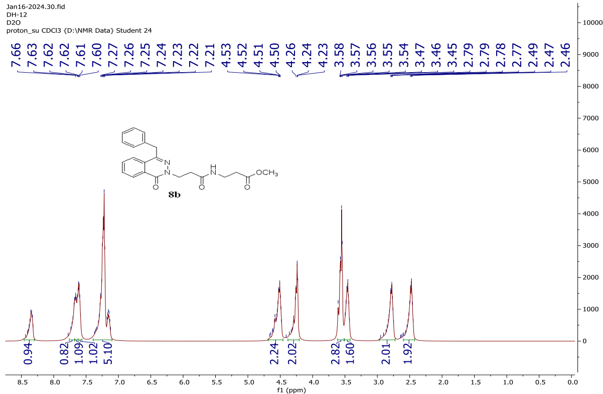
Figure S40 The D 2 O spectrum of compound 8b
