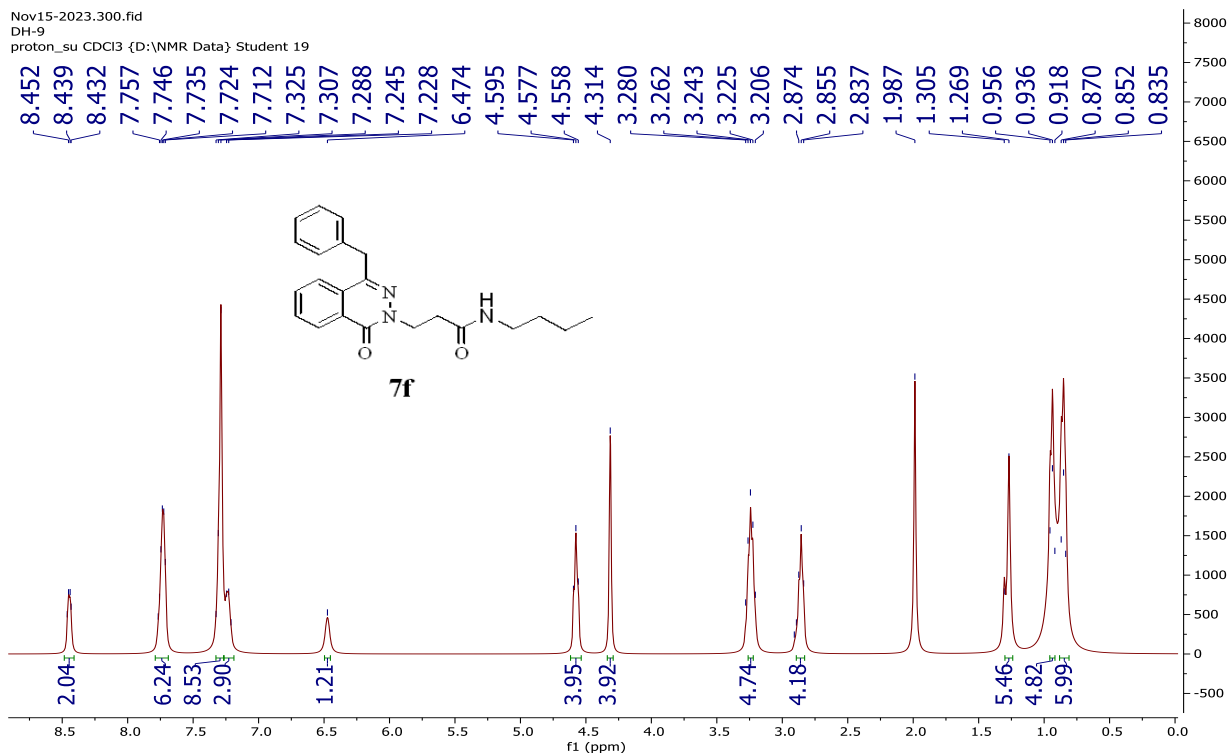
Figure S27 The ^1\text{H} -NMR spectrum of compound 7f
