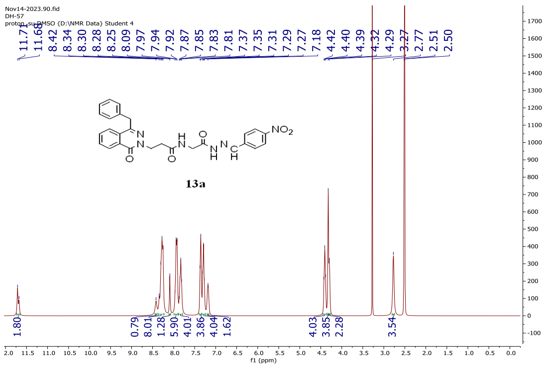
Figure S87: The 1 H-NMR spectrum of compound 13a
