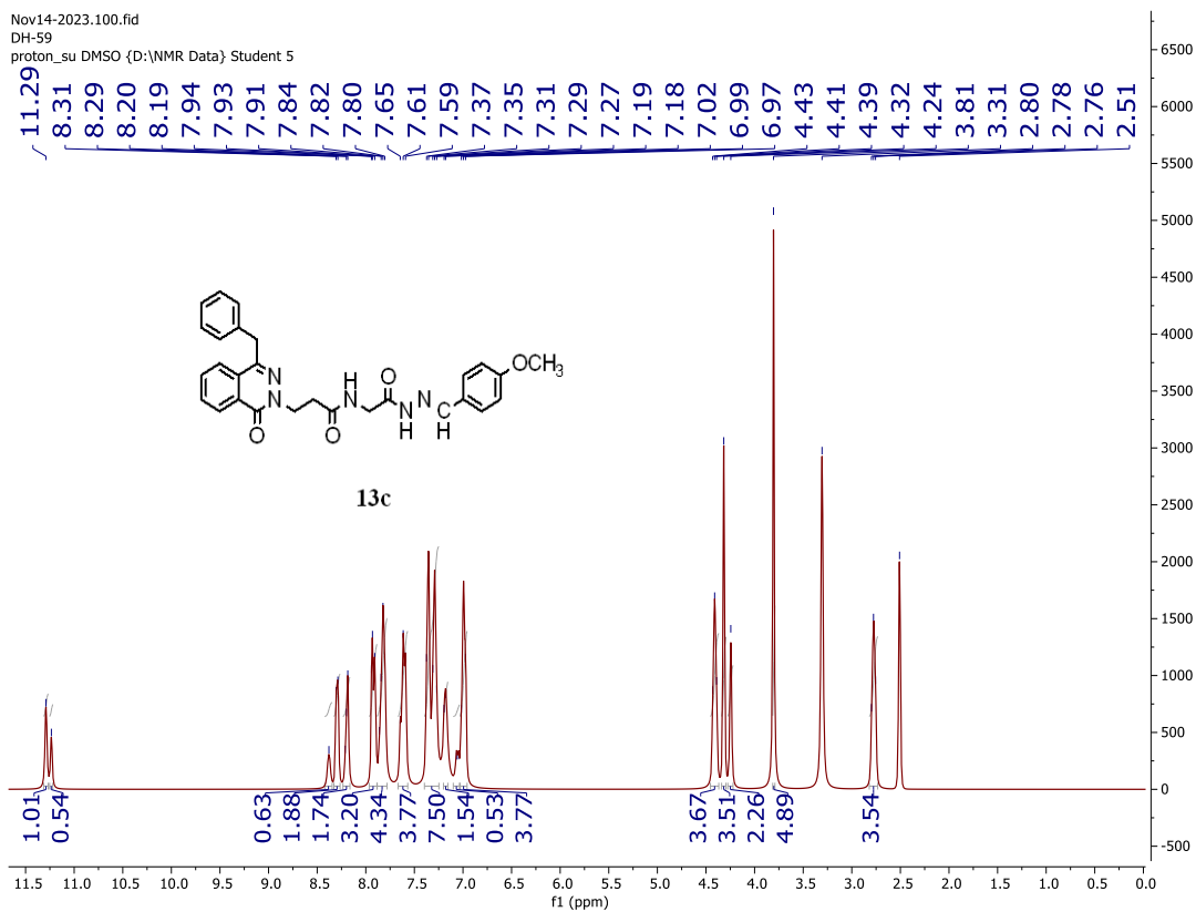
Figure S93: The 1 H-NMR spectrum of compound 13c
