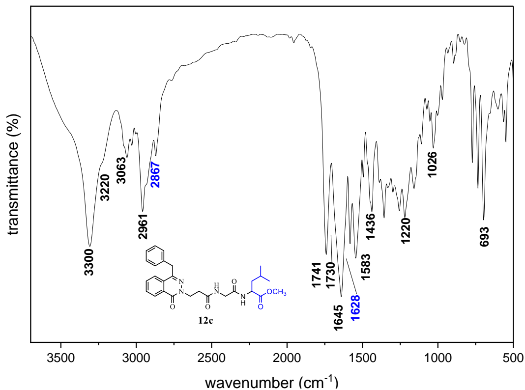
Figure S86: The IR spectrum of compound 12c
