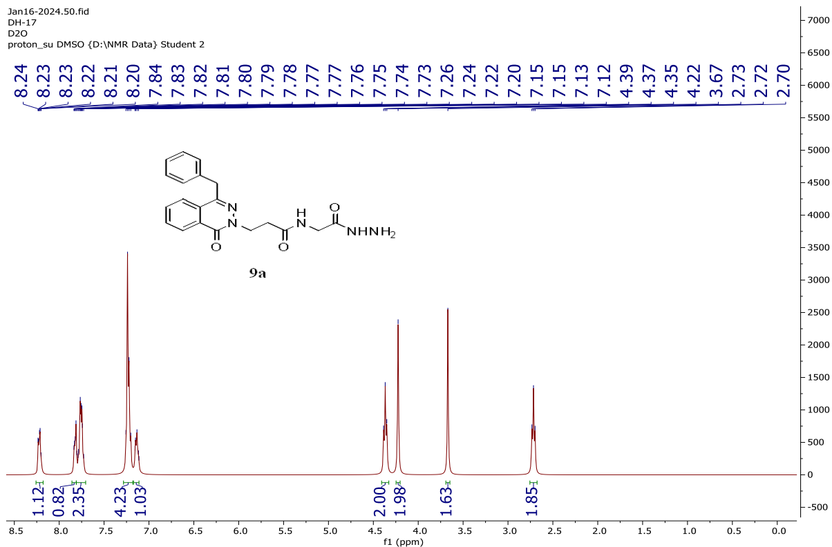
Figure S48 The D2O spectrum of compound 9a
