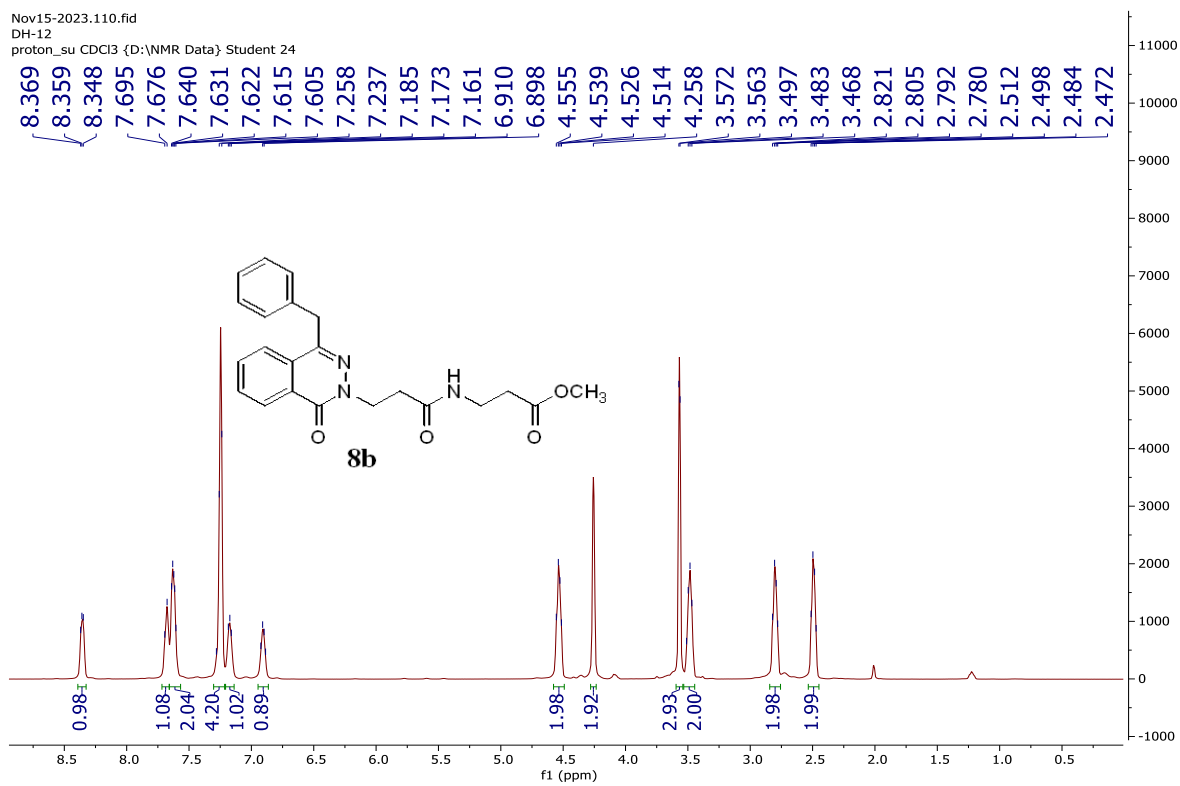
Figure S38 The 1 H-NMR spectrum of compound 8b
