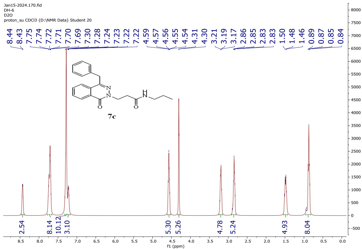
Figure S18 The D 2 O spectrum of compound 7c
