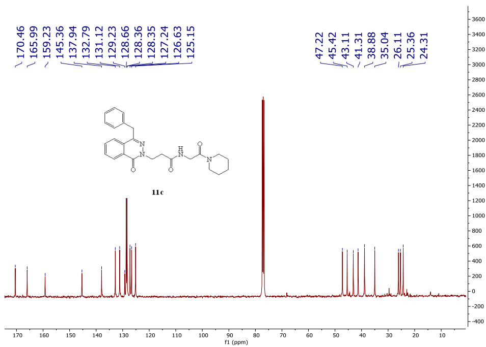
Figure S67: The ^{13}\text{C} -NMR spectrum of compound 11c
