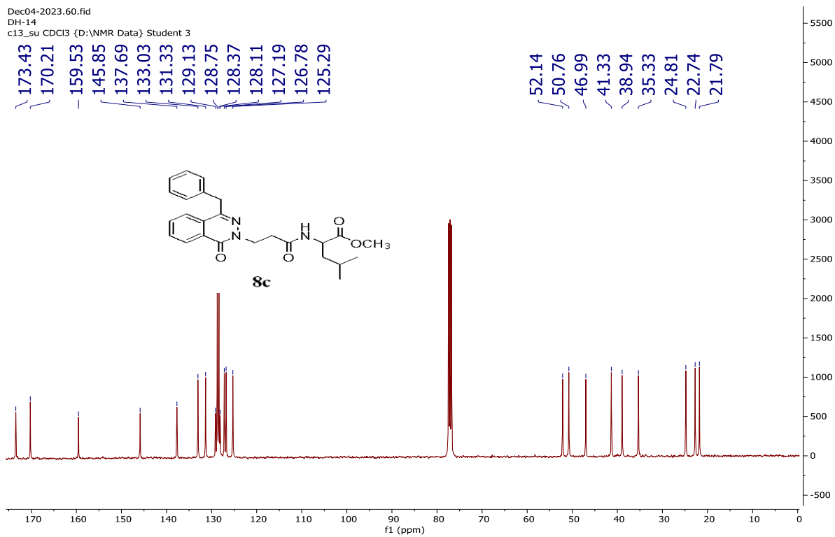
Figure S43 The 13 C-NMR spectrum of compound 8c
