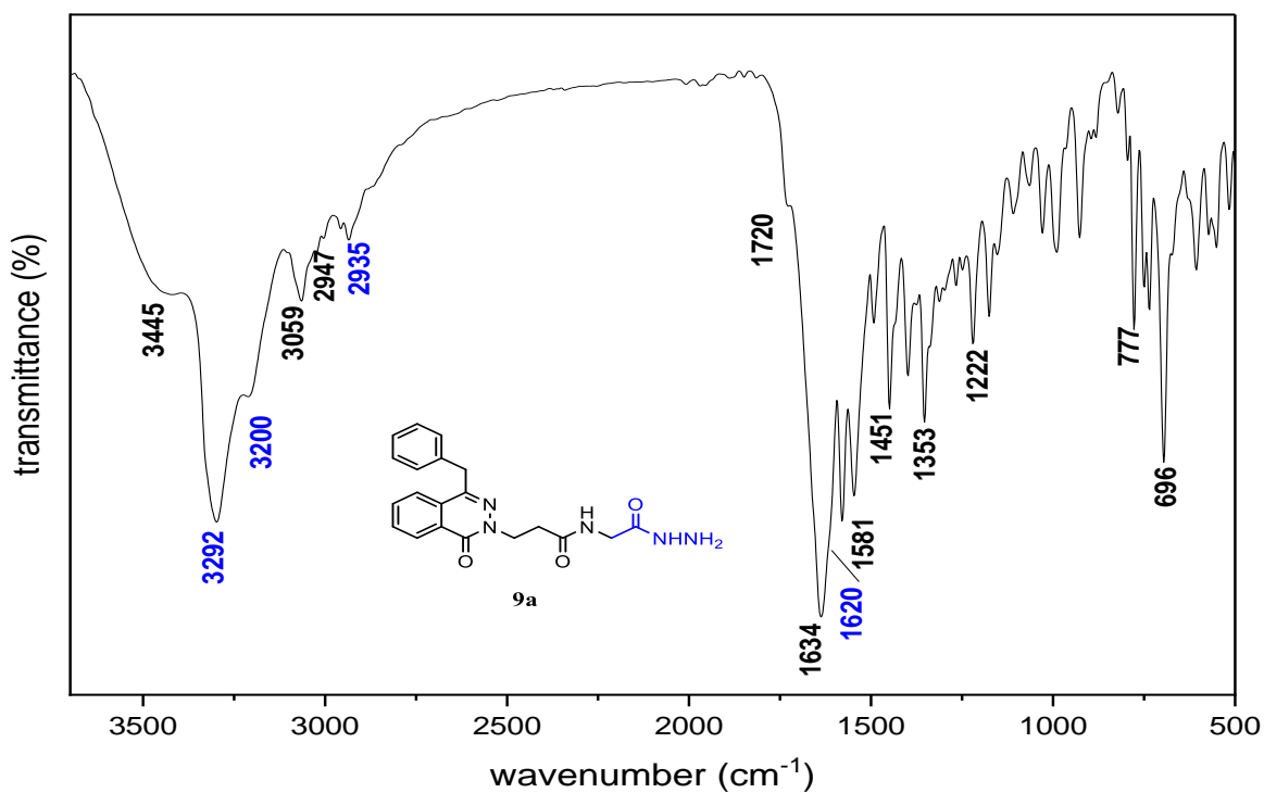
Figure S49 The IR spectrum of compound 9a
