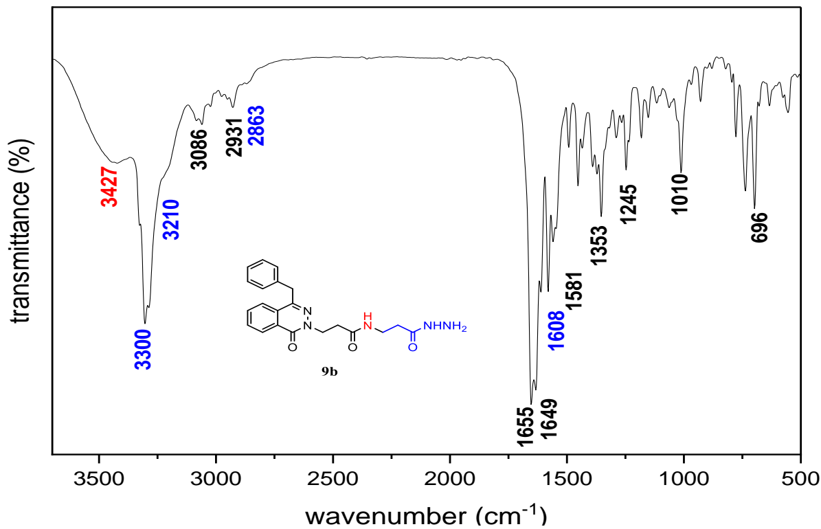
Figure S53 The IR spectrum of compound 9b
