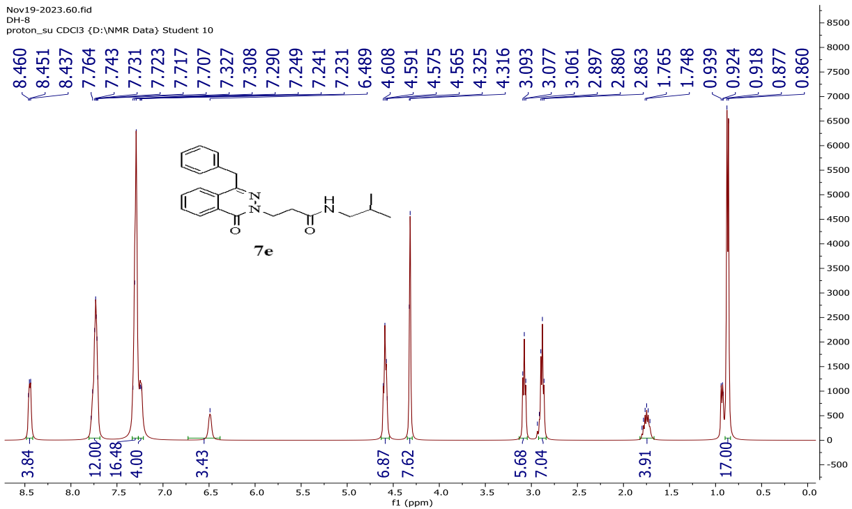
Figure S23 The ^1\text{H} -NMR spectrum of compound 7e
