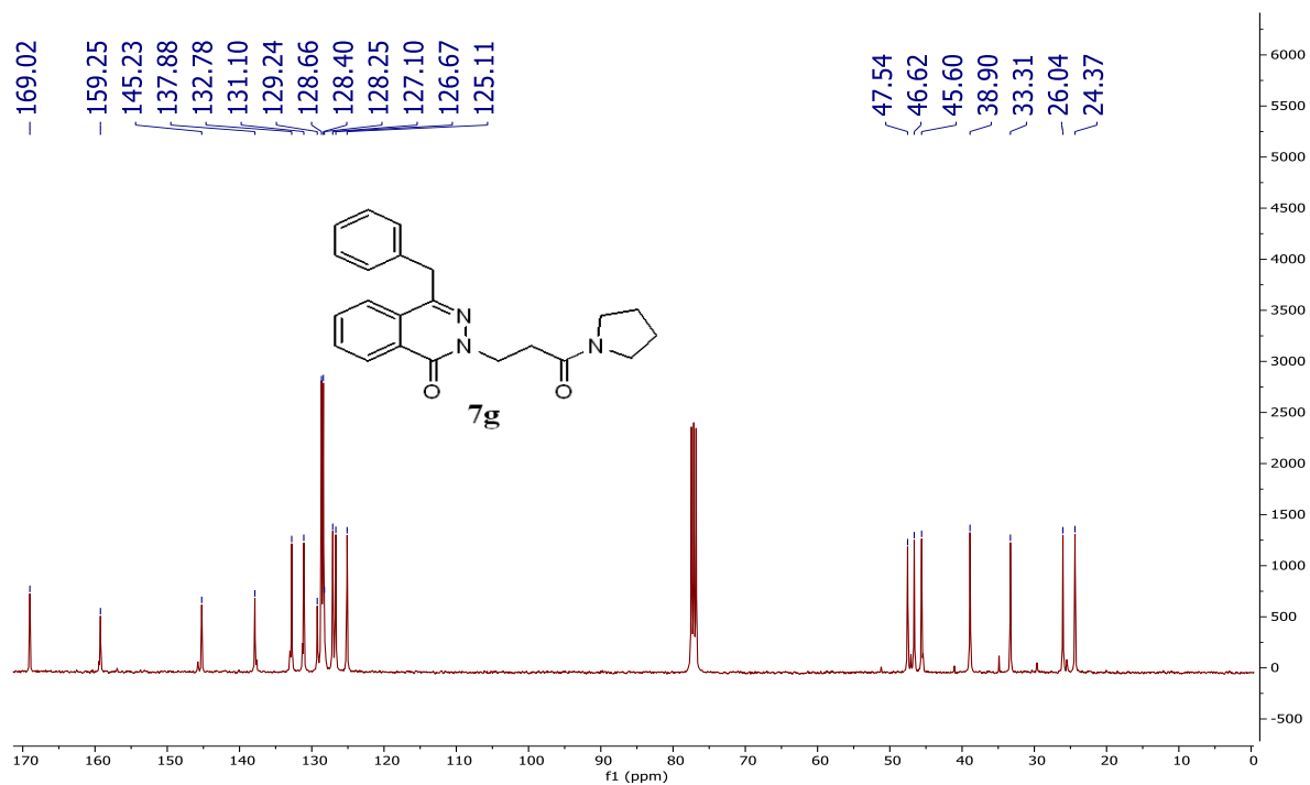
Figure S32 The ^{13}\text{C} -NMR spectrum of compound 7g
