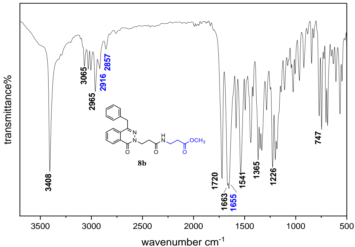
Figure S41 The IR spectrum of compound 8b
