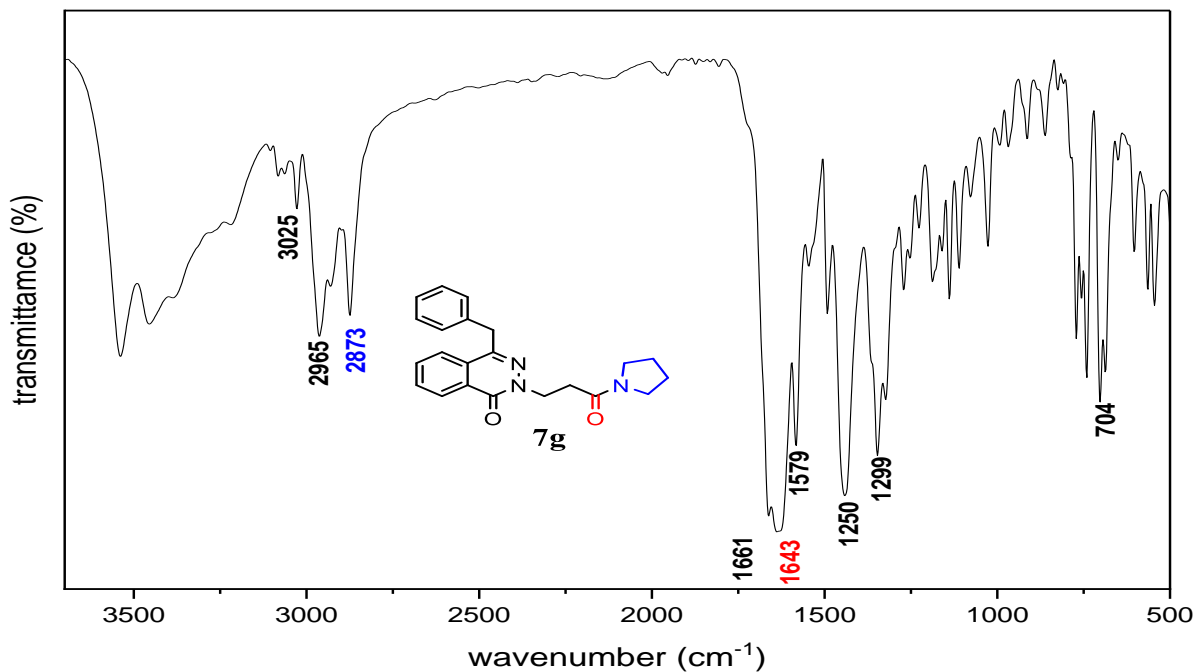
Figure S33 The IR spectrum of compound 7g
