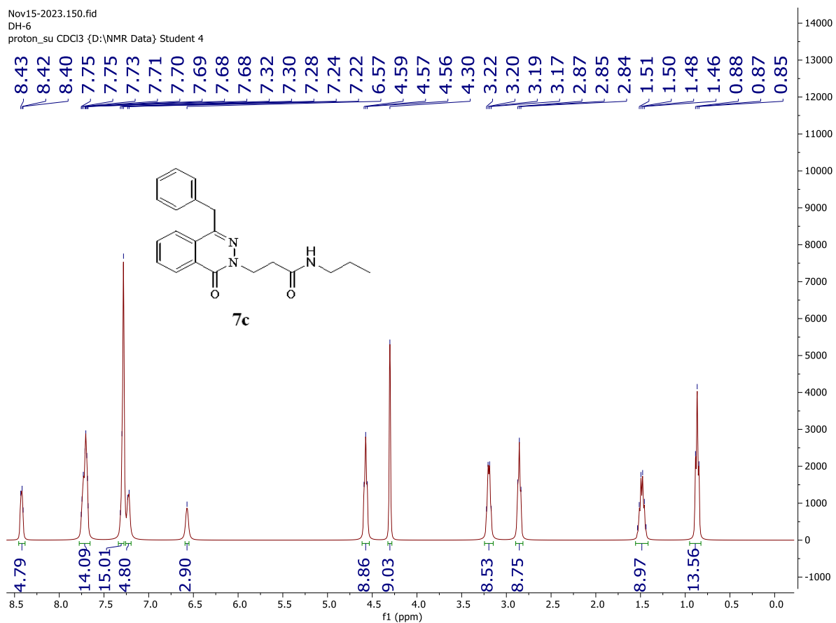
Figure S16 The 1 H-NMR spectrum of compound 7c
