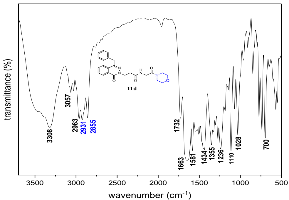
Figure S73: The IR spectrum of compound 11d
