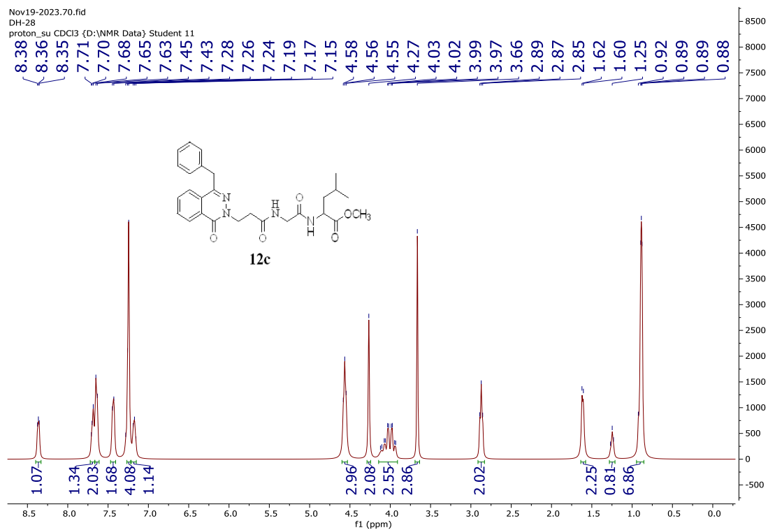
Figure S83: The ^1\text{H} -NMR spectrum of compound 12c
