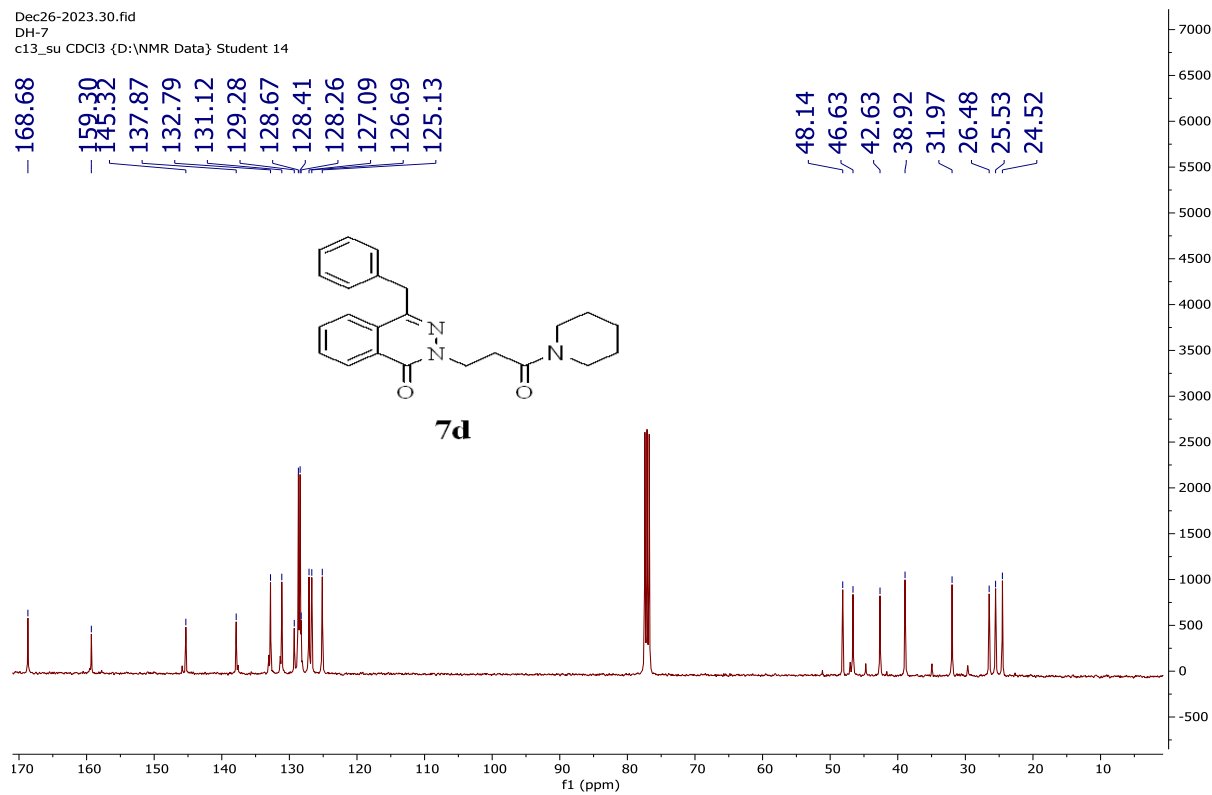
Figure S21 The 13 C-NMR spectrum of compound 7d
