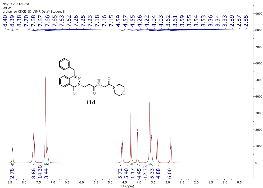
Figure S70 : The ^1\text{H} -NMR spectrum of compound 11d
