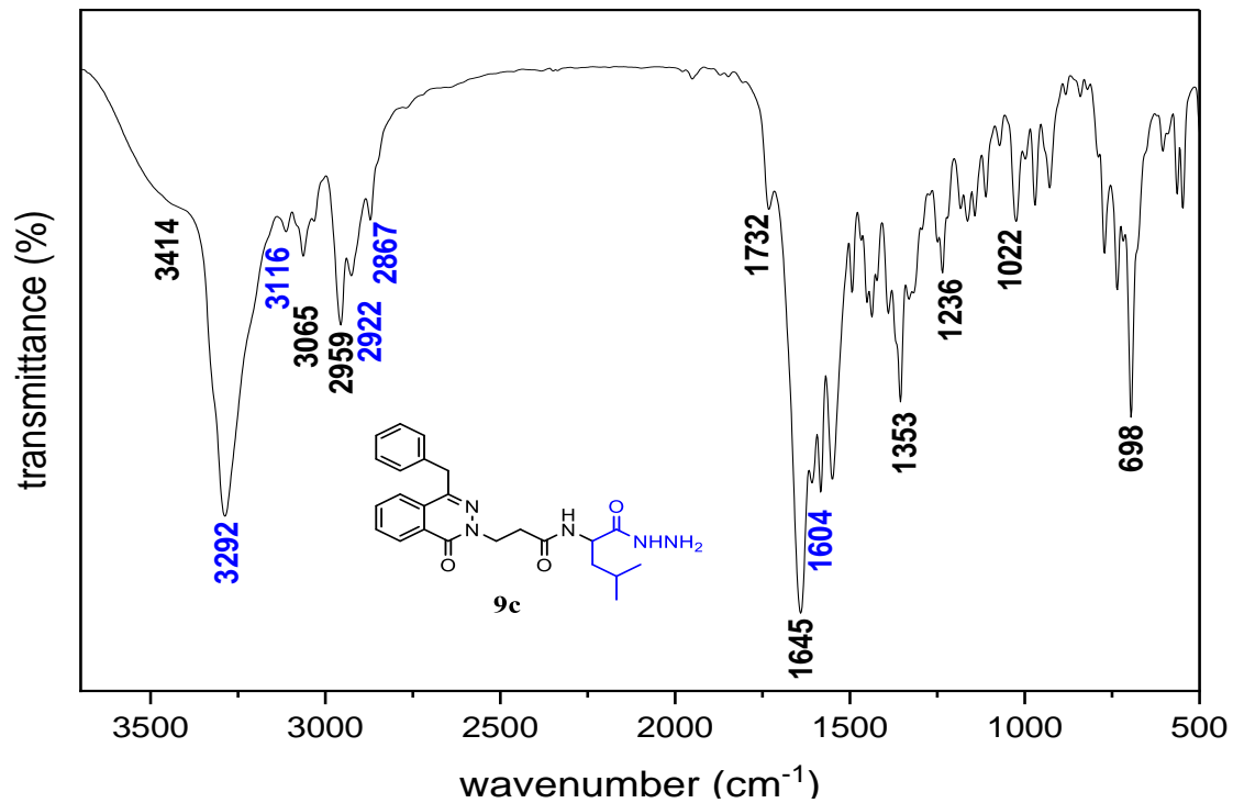
Figure S57: The IR spectrum of compound 9c
