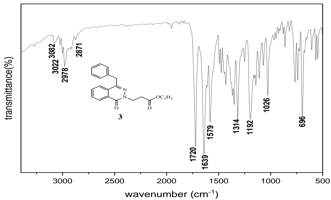
Figure S3 The IR spectrum of compound 3.
