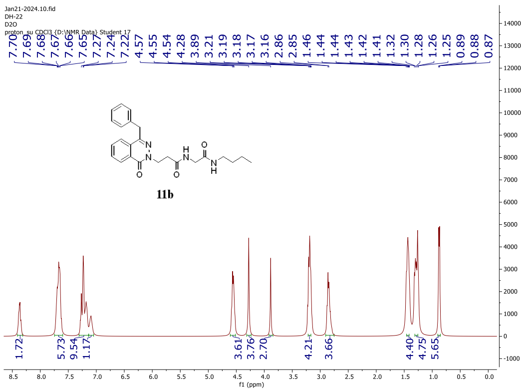
Figure S64: The D 2 O spectrum of compound 11b
