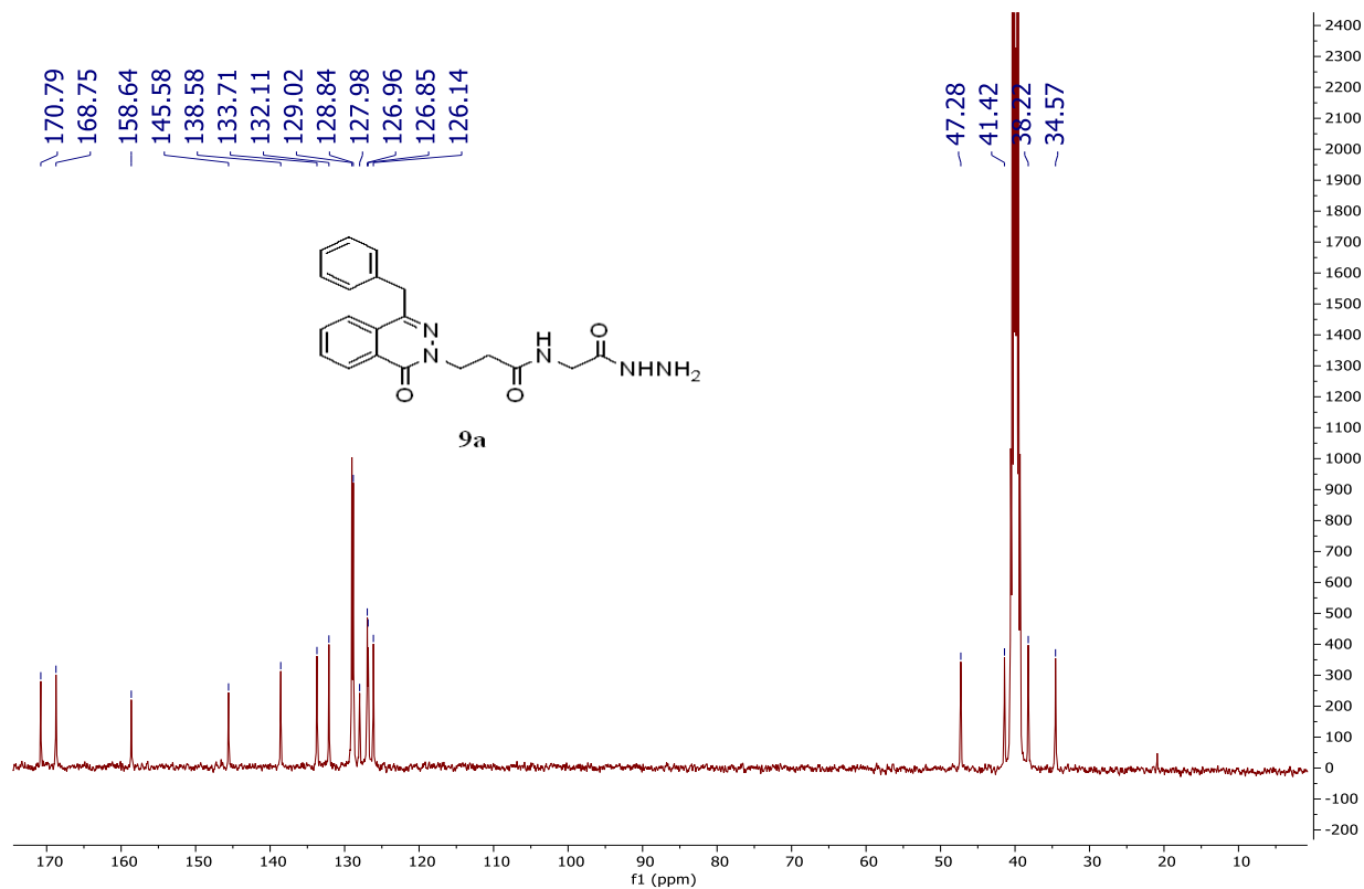
Figure S47 The ^{13}\text{C-NMR} spectrum of compound 9a
