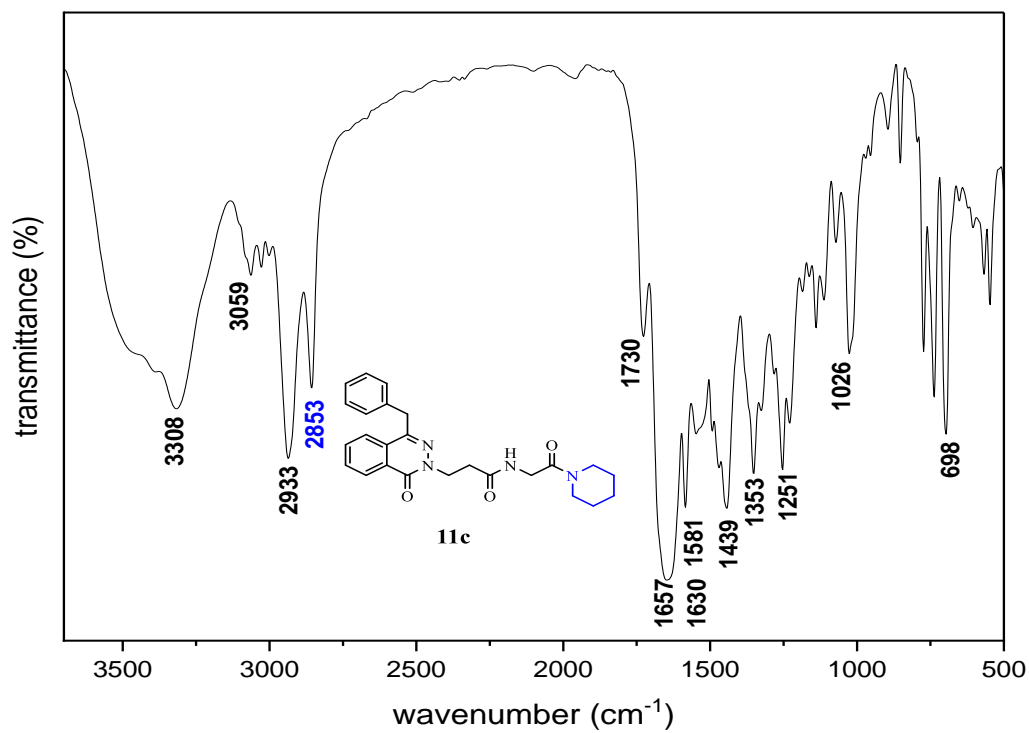
Figure S69: The IR spectrum of compound 11c
