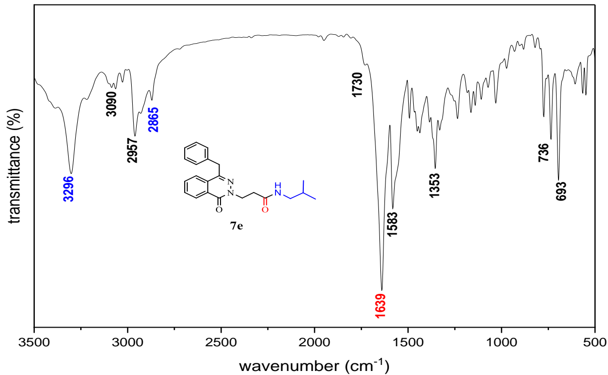
Figure S26 The IR spectrum of compound 7e
