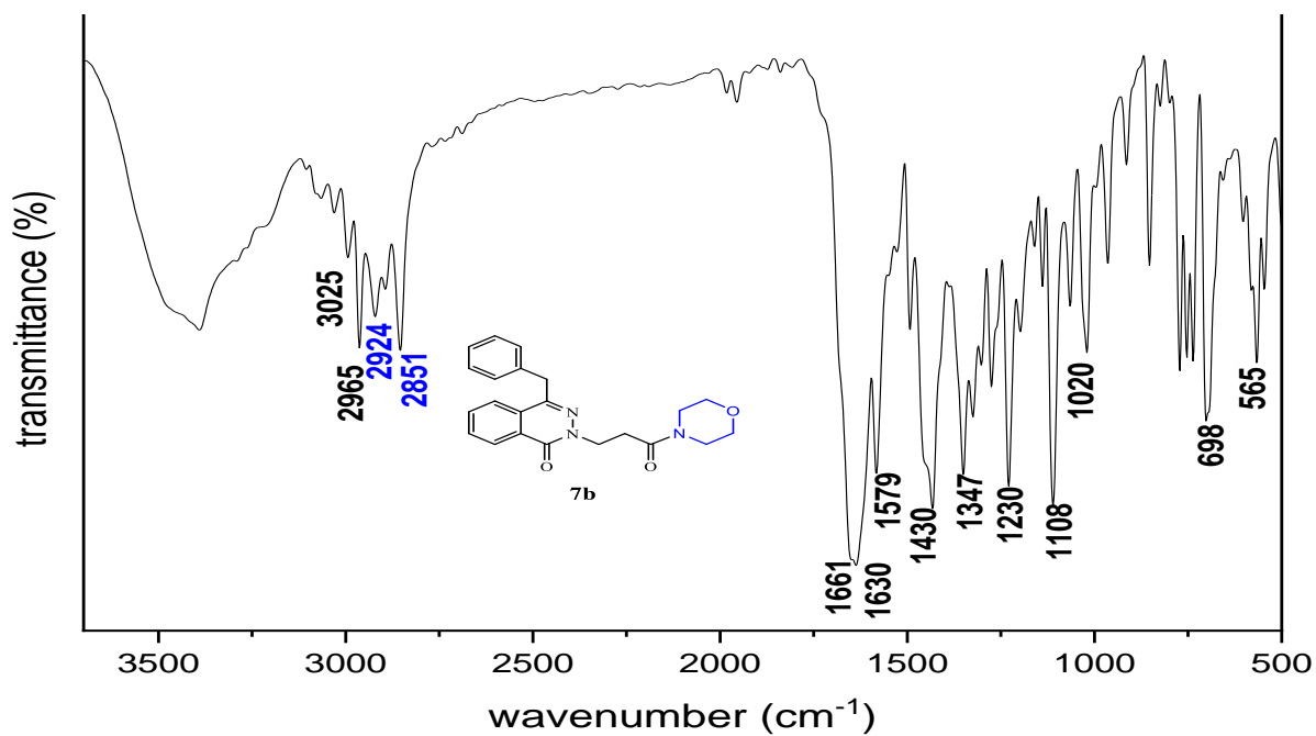
Figure S15 The IR spectrum of compound 7b
