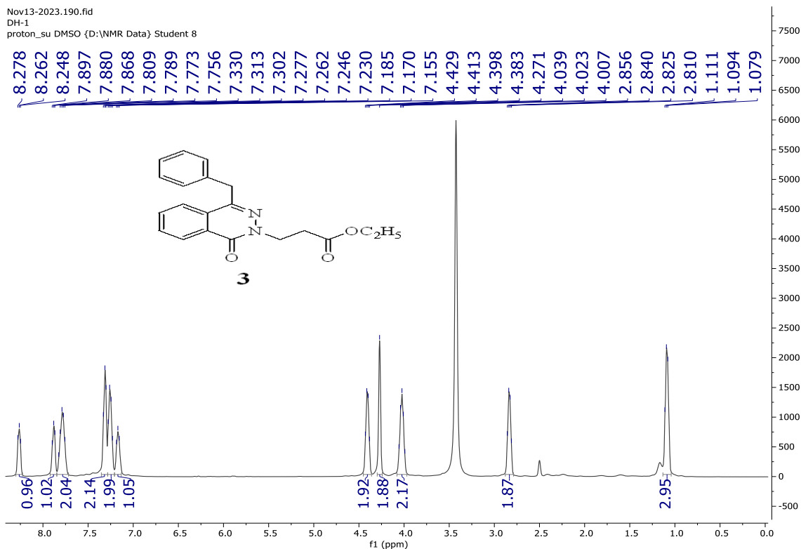
Figure S1 The ^1\text{H} -NMR spectrum of compound 3 .
