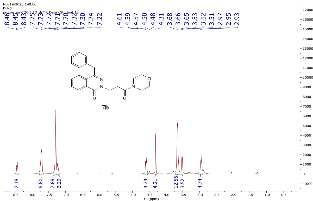
Figure S13 The ^1\text{H} -NMR spectrum of compound 7b
