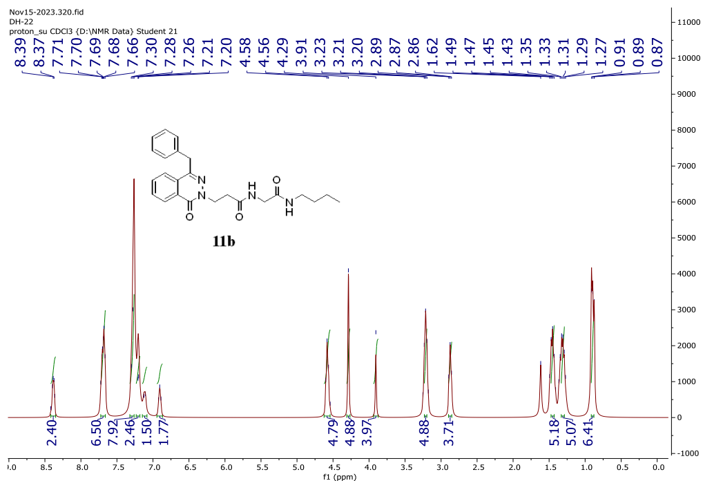
Figure 62: The 1 H-NMR spectrum of compound 11b
