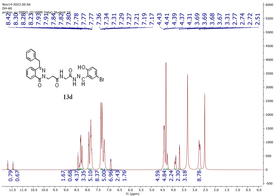
Figure S95: The 1 H-NMR spectrum of compound 13d
