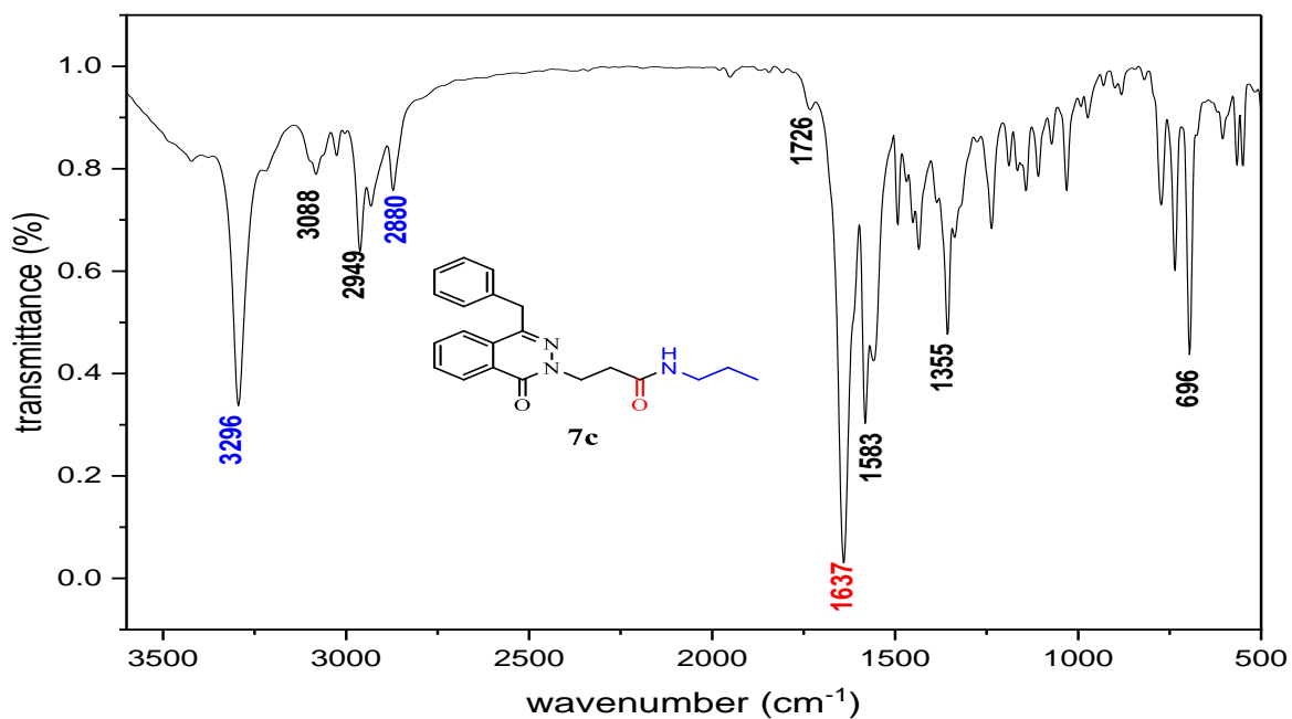
Figure S19 The IR spectrum of compound 7c
