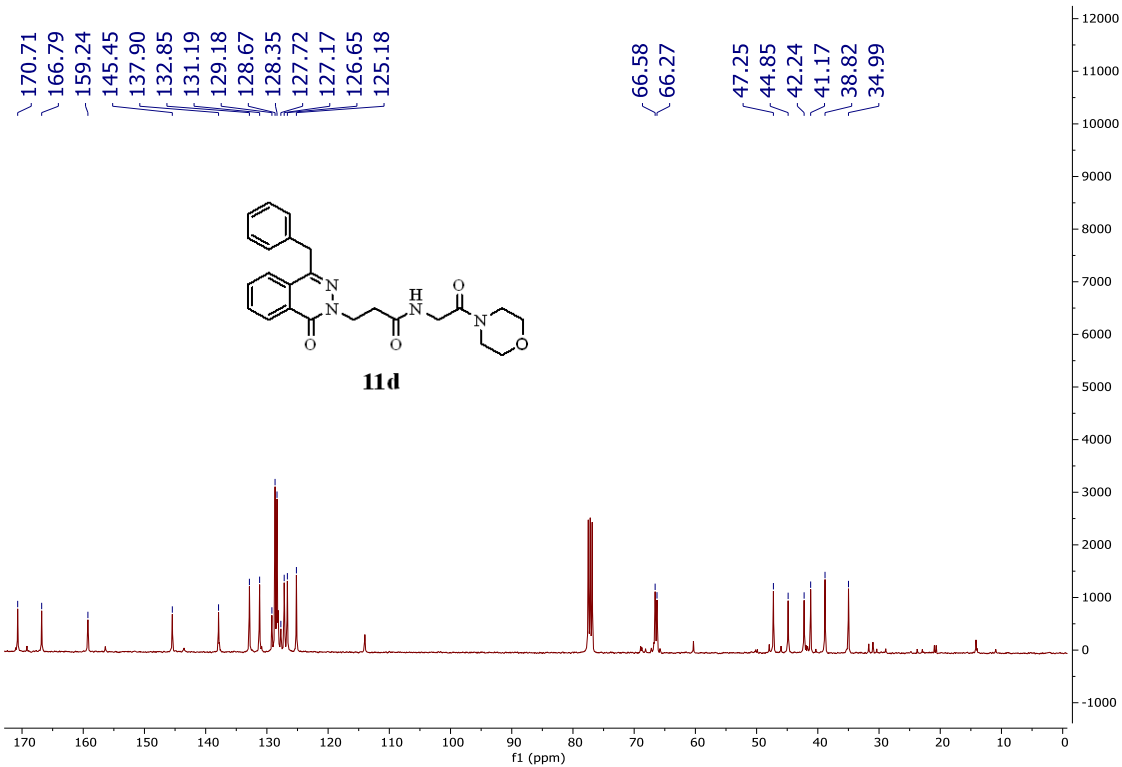
Figure S71: The ^{13}\text{C} -NMR spectrum of compound 11d
