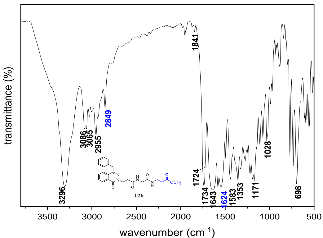
Figure S81: The IR spectrum of compound 12b
