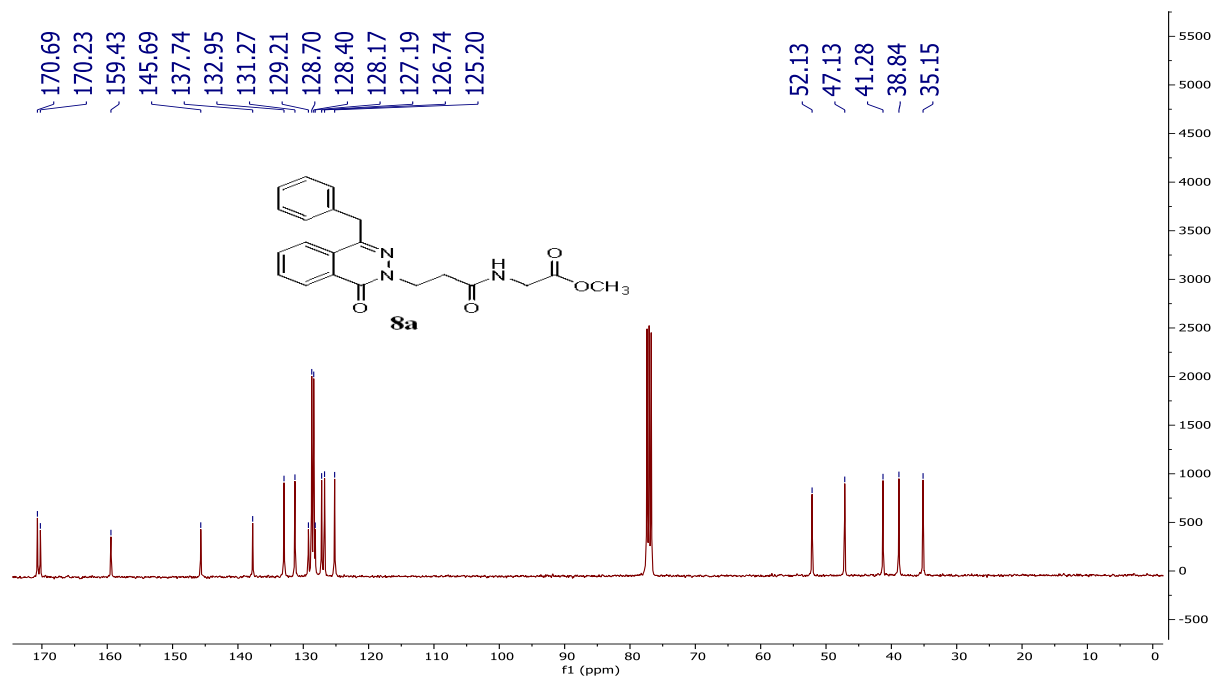
Figure S35 The 13 C-NMR spectrum of compound 8a
