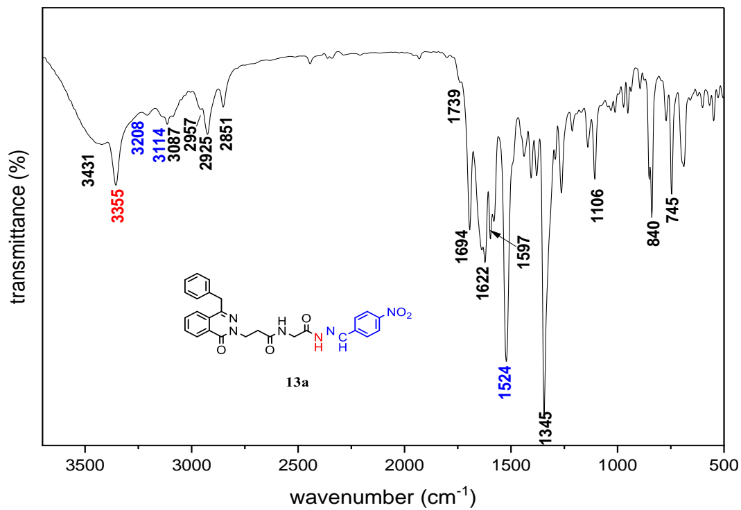
Figure S89: The IR spectrum of compound 13a
