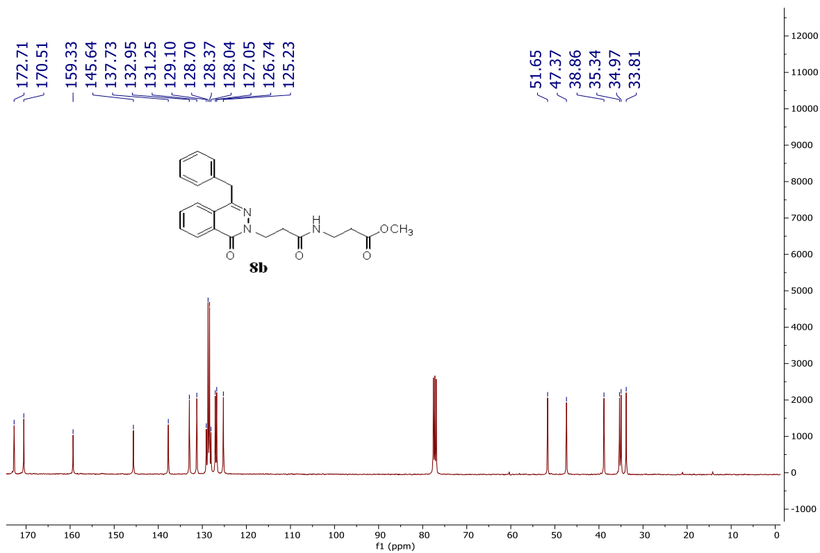
Figure S39 The 13 C-NMR spectrum of compound 8b
