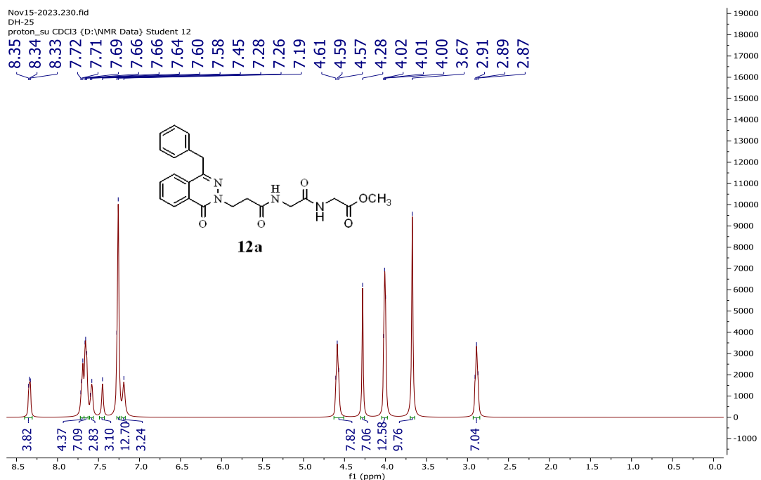
Figure S74: The ^1\text{H} -NMR spectrum of compound 12a
