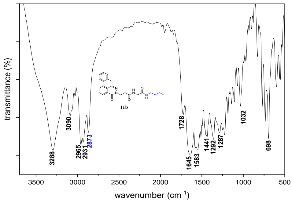
Figure S65: The IR spectrum of compound 11b
