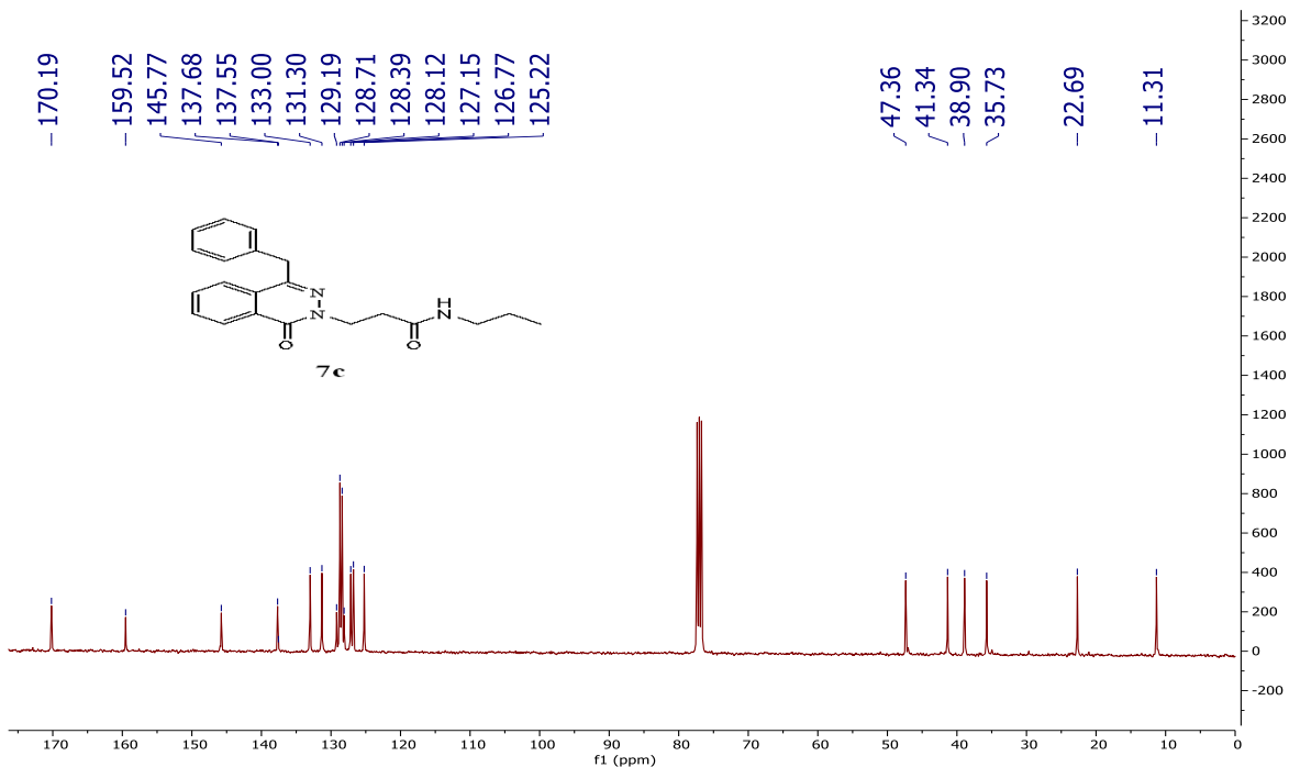
Figure S17 The 13 C-NMR spectrum of compound 7c
