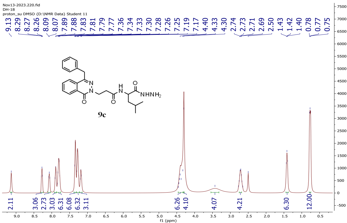
Figure S54 The ^1\text{H-NMR} spectrum of compound 9c
