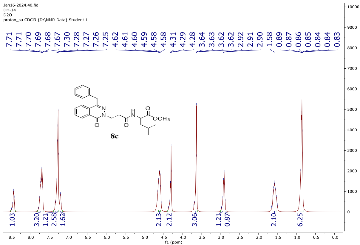
Figure S44 The D 2 O spectrum of compound 8c
