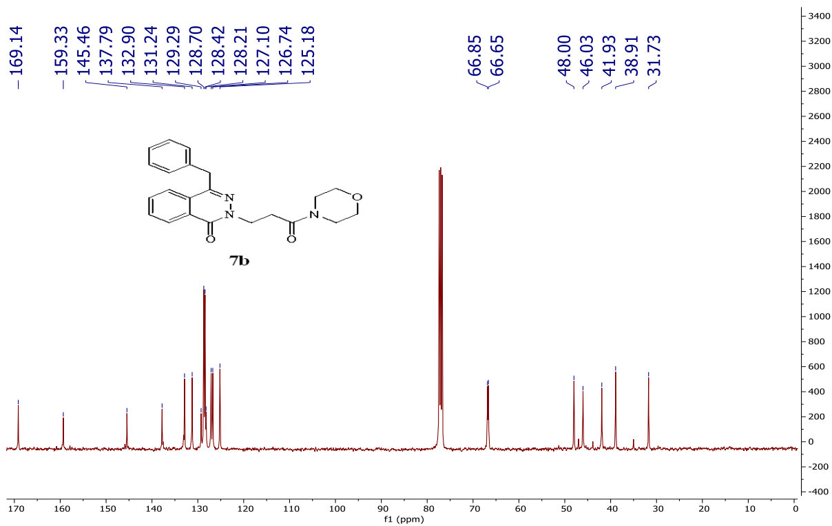
Figure S14 The ^{13}\text{C} -NMR spectrum of compound 7b
