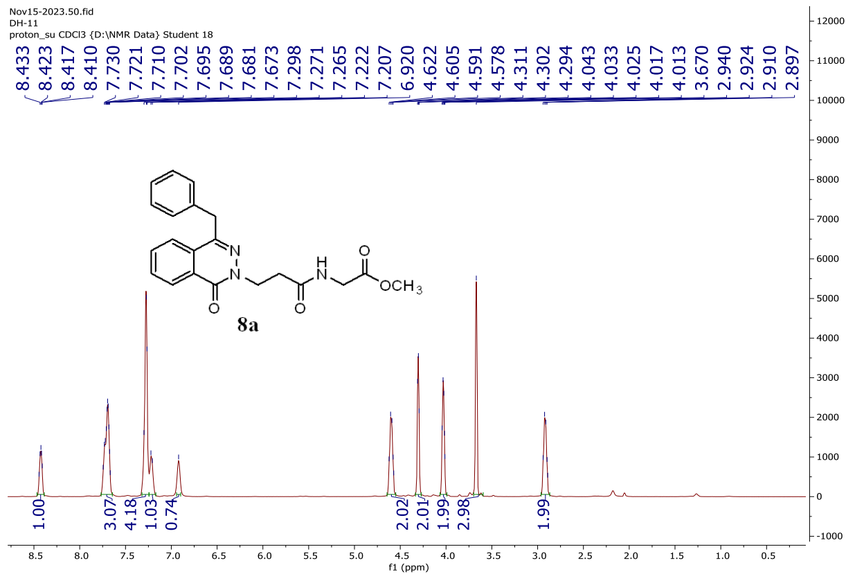
Figure S34 The 1 H-NMR spectrum of compound 8a
