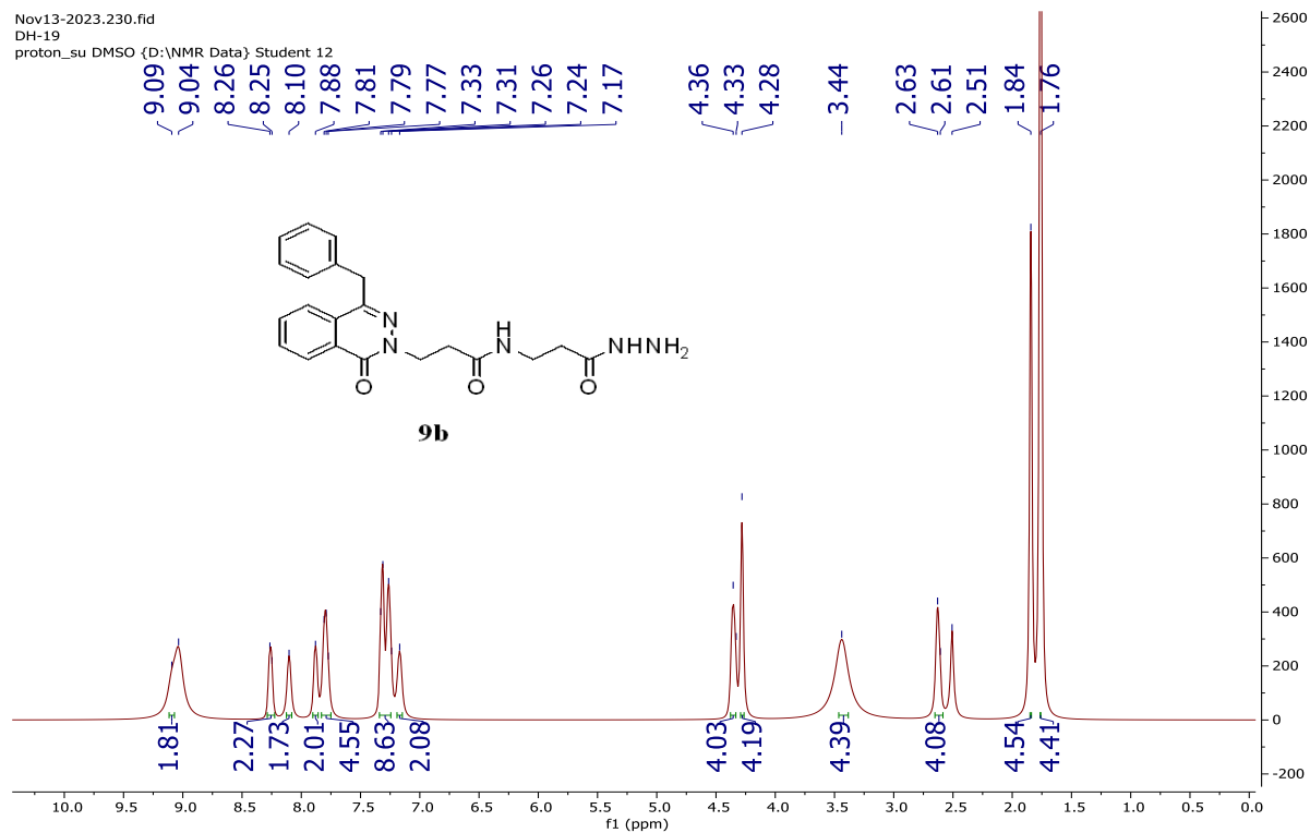
Figure S50 The 1 H-NMR spectrum of compound 9b
