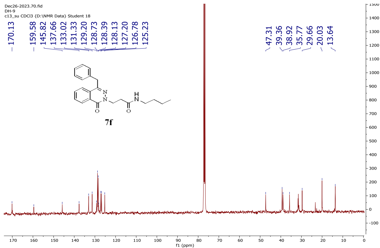
Figure S28 The ^{13}\text{C} -NMR spectrum of compound 7f
