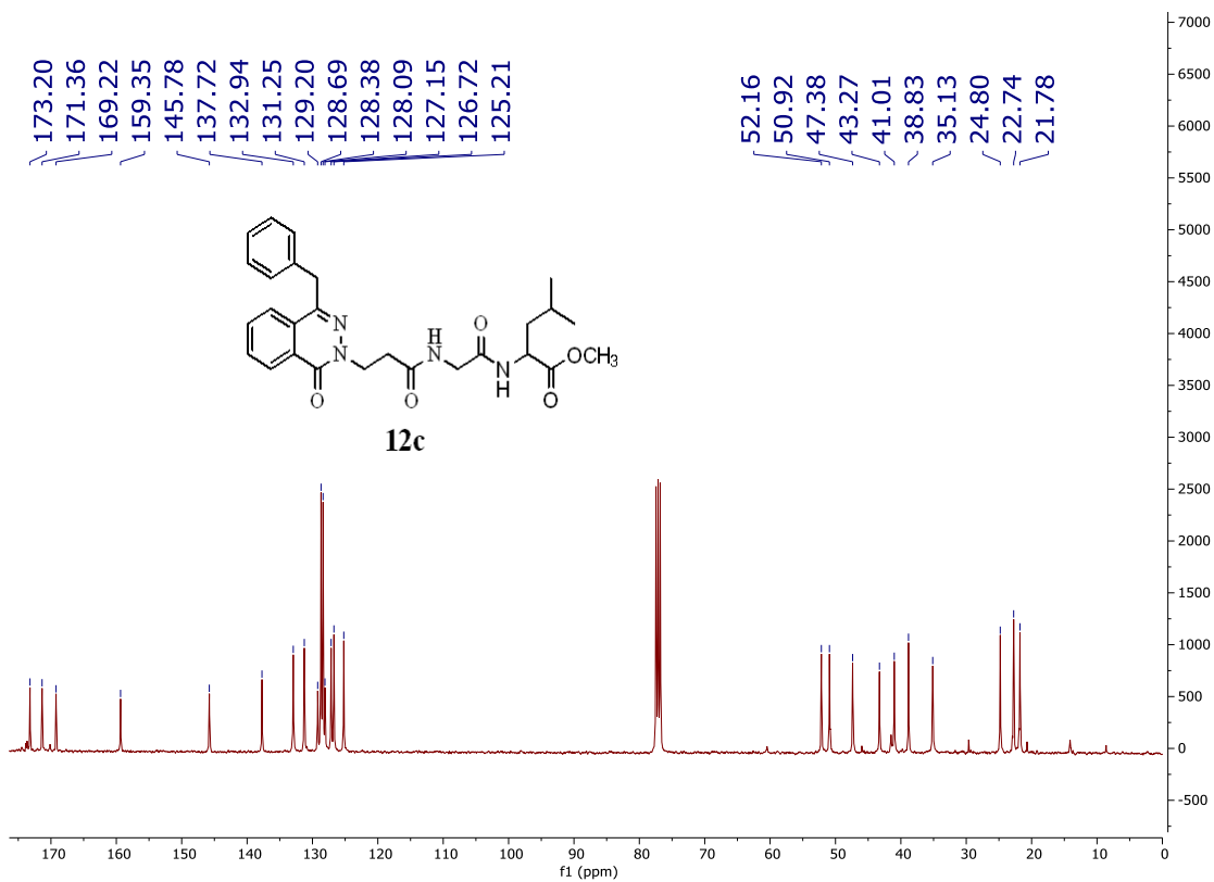
Figure S84: The ^{13}\text{C} -NMR spectrum of compound 12c
