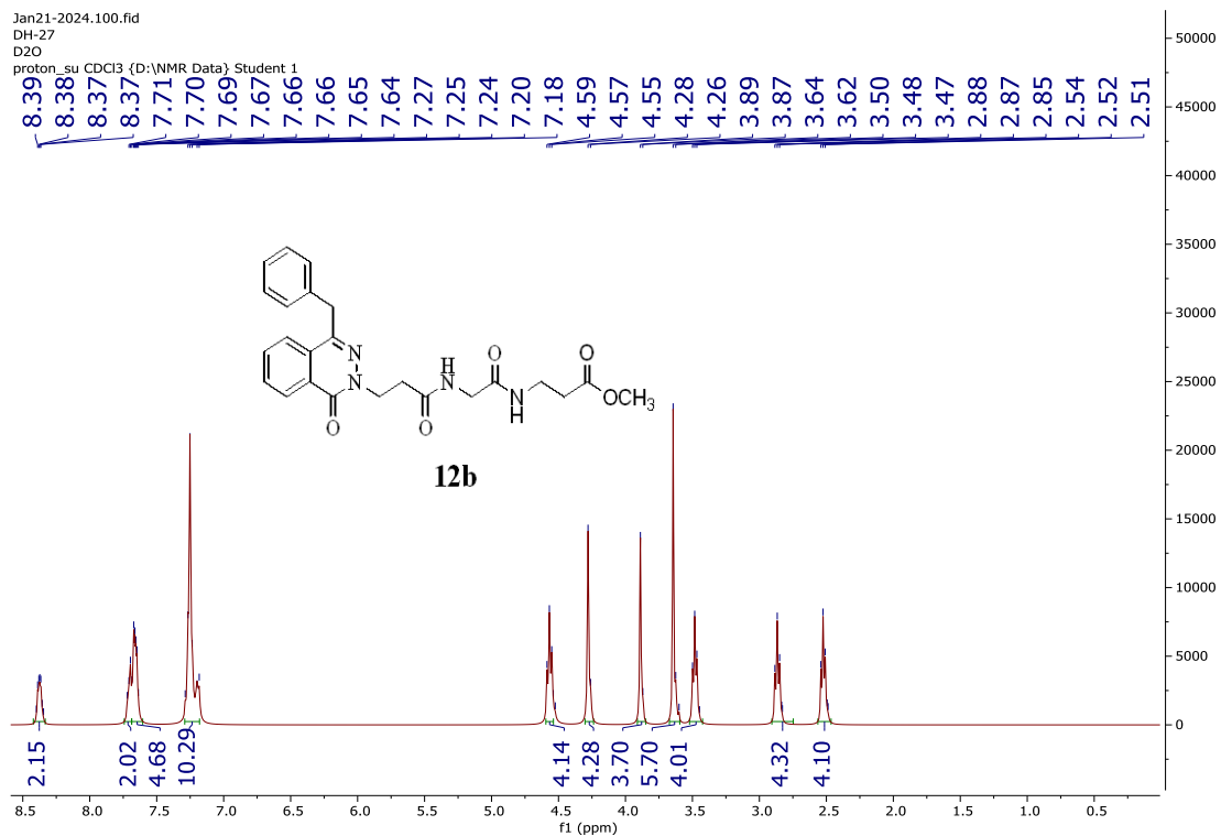
Figure S80: The D2O spectrum of compound 12b
