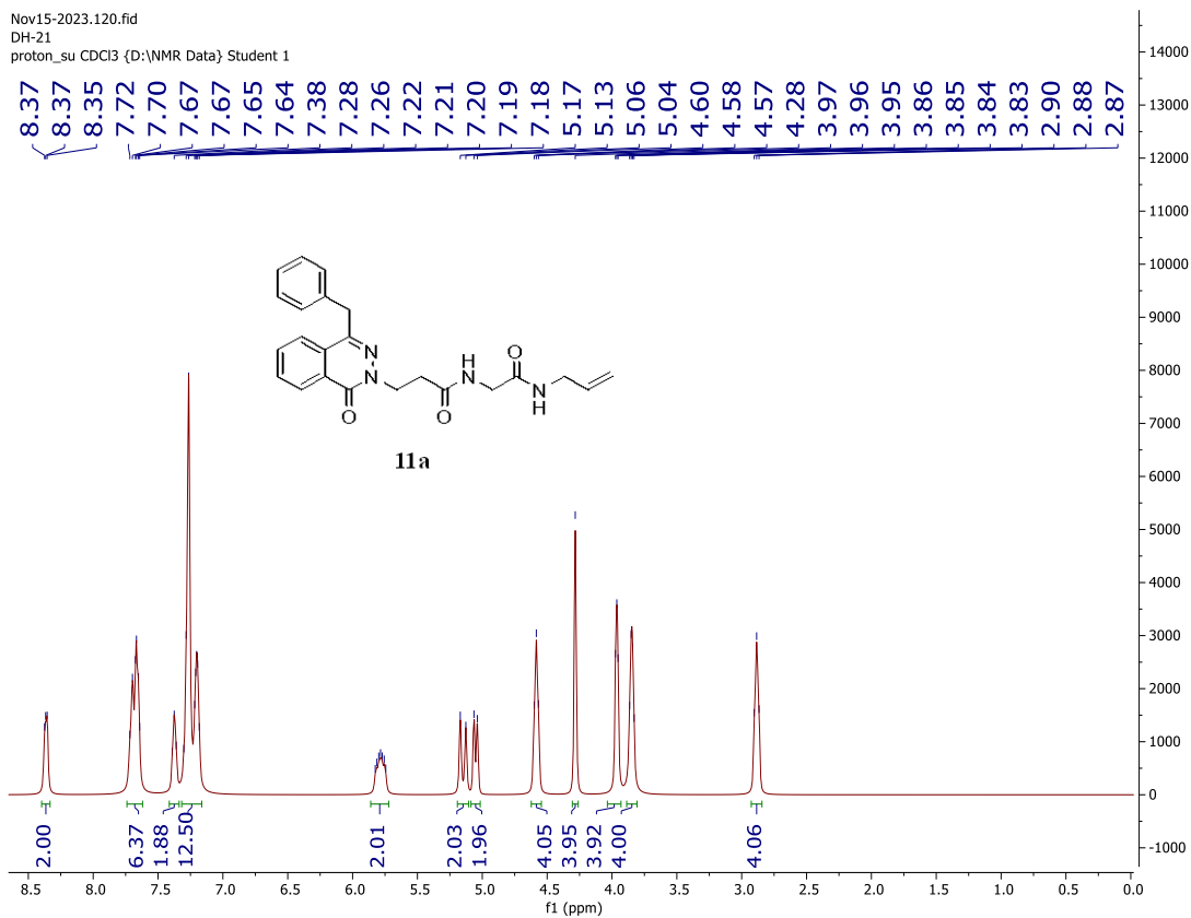
Figure S58: The 1 H-NMR spectrum of compound 11a
