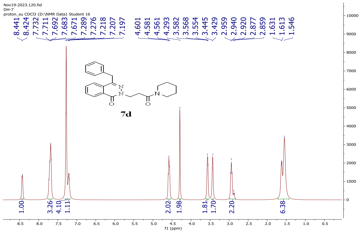
Figure S20 The 1 H-NMR spectrum of compound 7d
