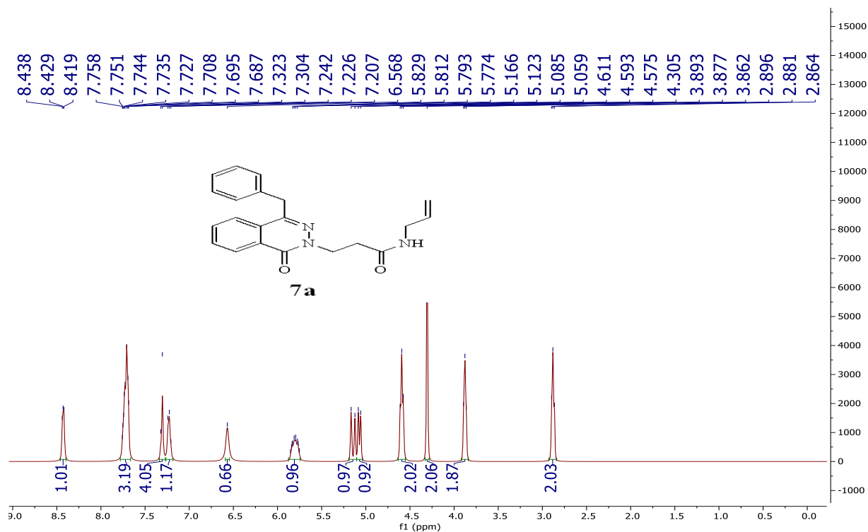
Figure S9 The ^1\text{H-NMR} spectrum of compound 7a
