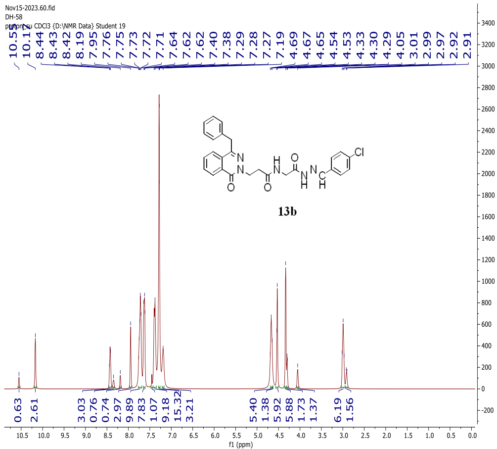
Figure S90: The ^1\text{H-NMR} spectrum of compound 13b
