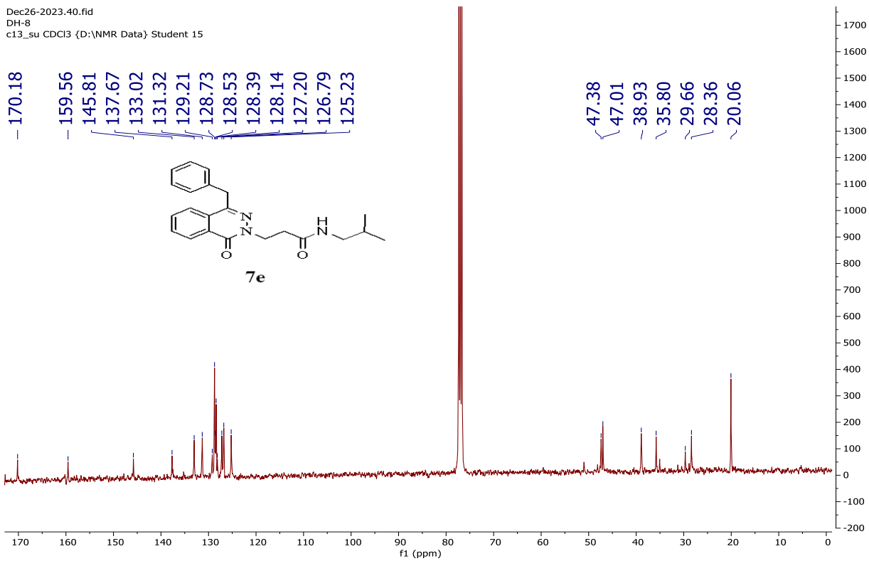
Figure S24 The ^{13}\text{C} -NMR spectrum of compound 7e
