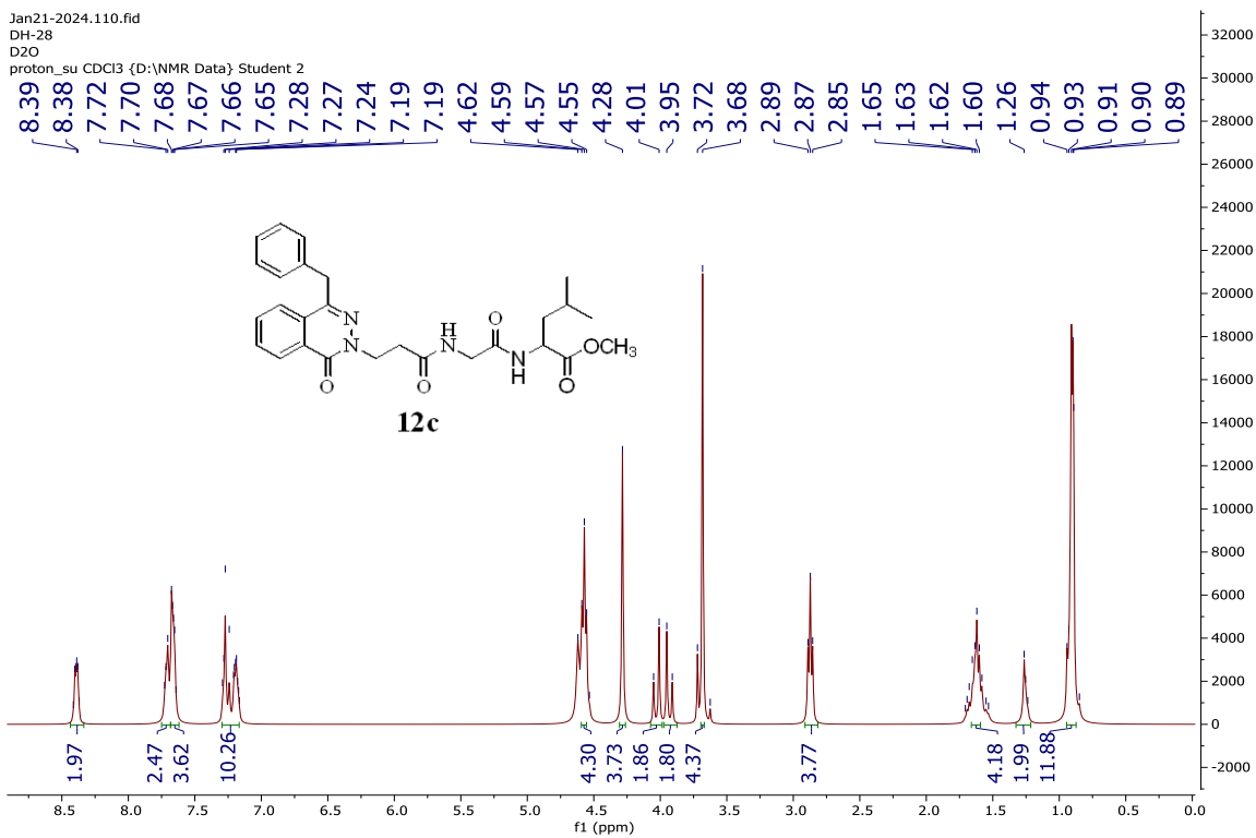
Figure S85: The D 2 O spectrum of compound 12c
