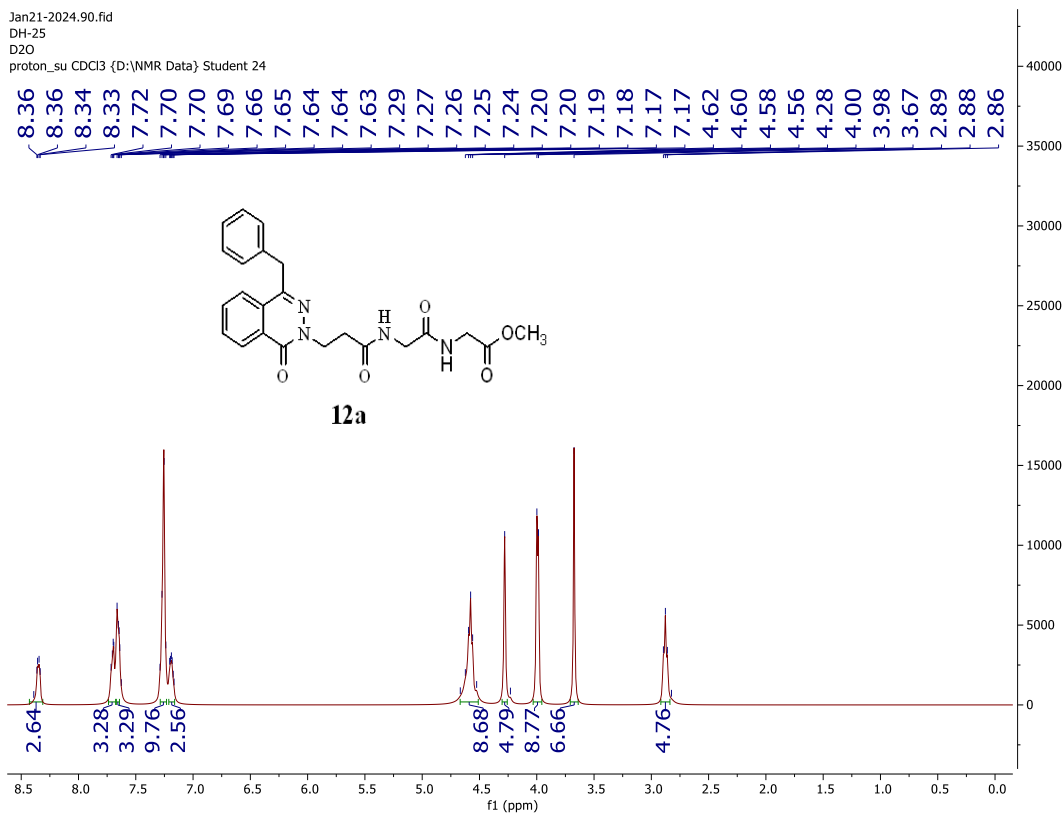
Figure S76: The D2O spectrum of compound 12a
