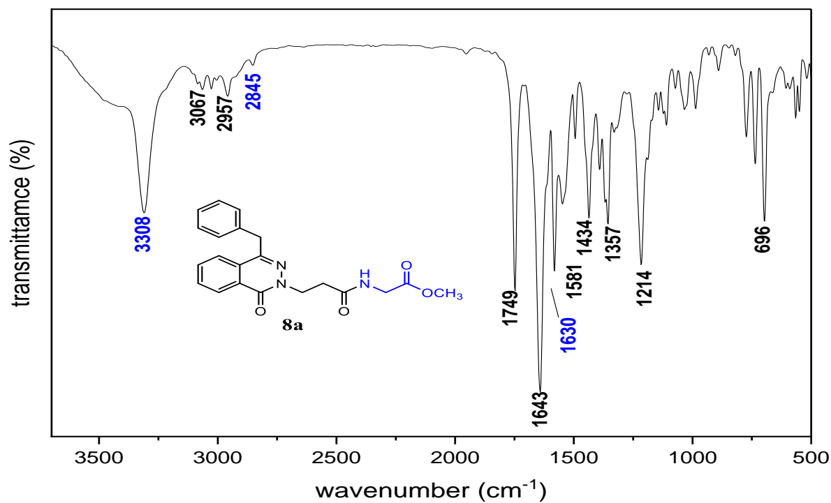
Figure S37 The IR spectrum of compound 8a
