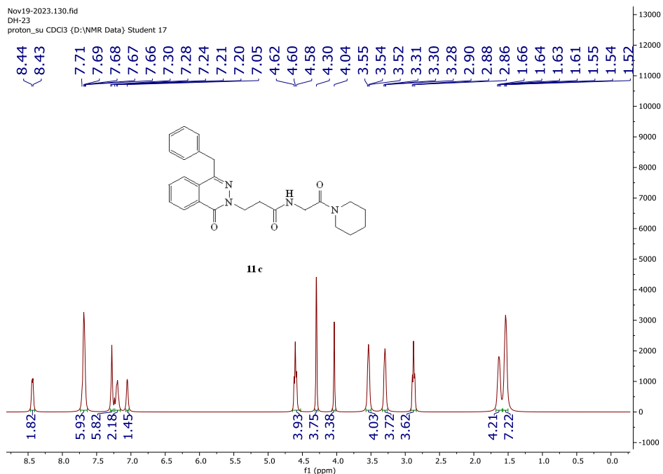
Figure S66: The ^1\text{H} -NMR spectrum of compound 11c
