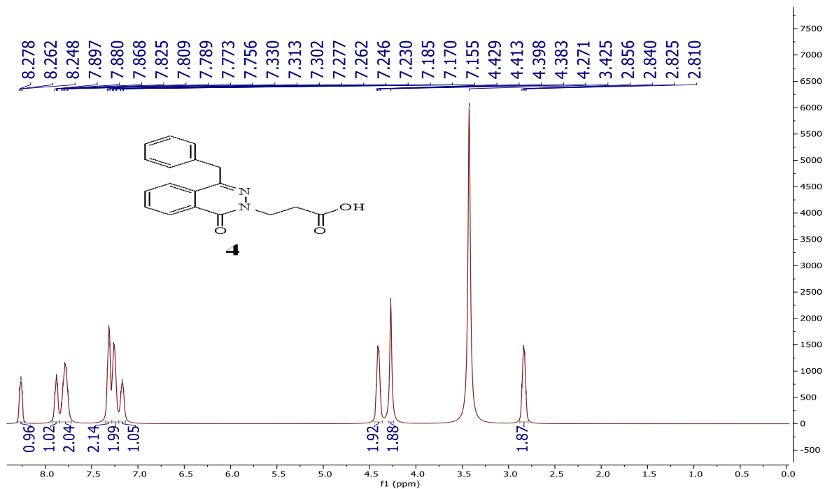
Figure S4 The 1 H-NMR spectrum of compound 4.
