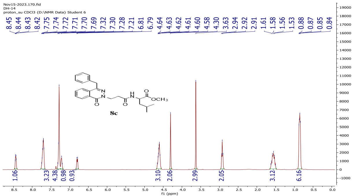
Figure S42 The ^1\text{H-NMR} spectrum of compound 8c
