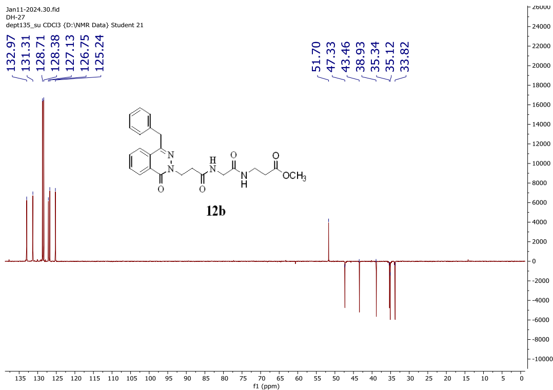
Figure S82: The dept135 spectrum of compound 12b
