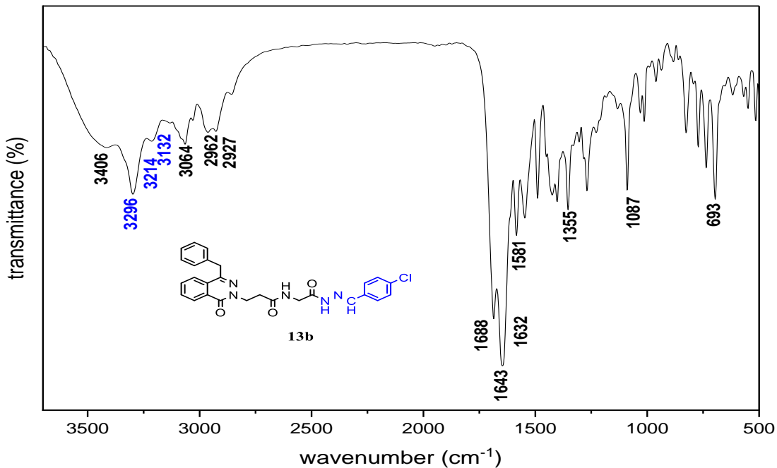
Figure S92: The IR spectrum of compound 13b
