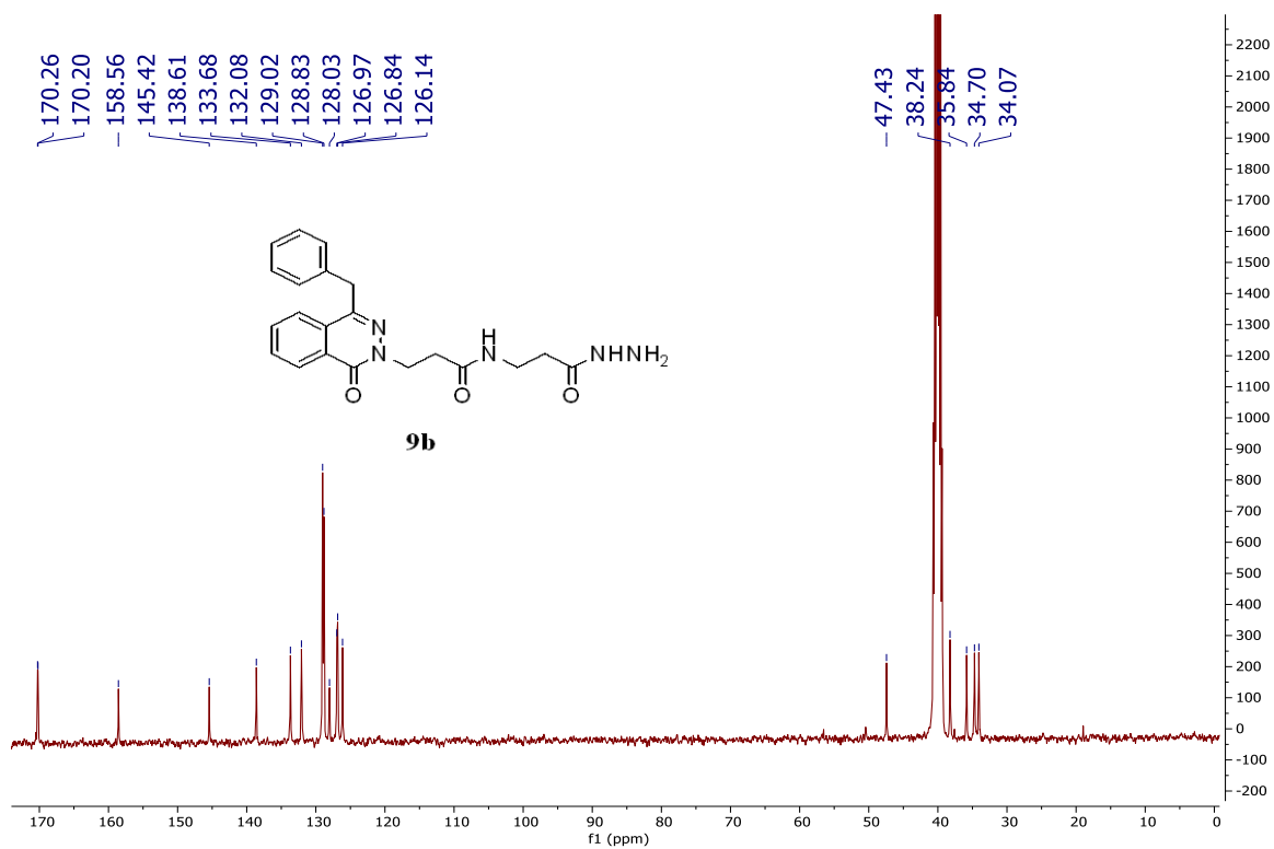
Figure S51 The 13 C-NMR spectrum of compound 9b
