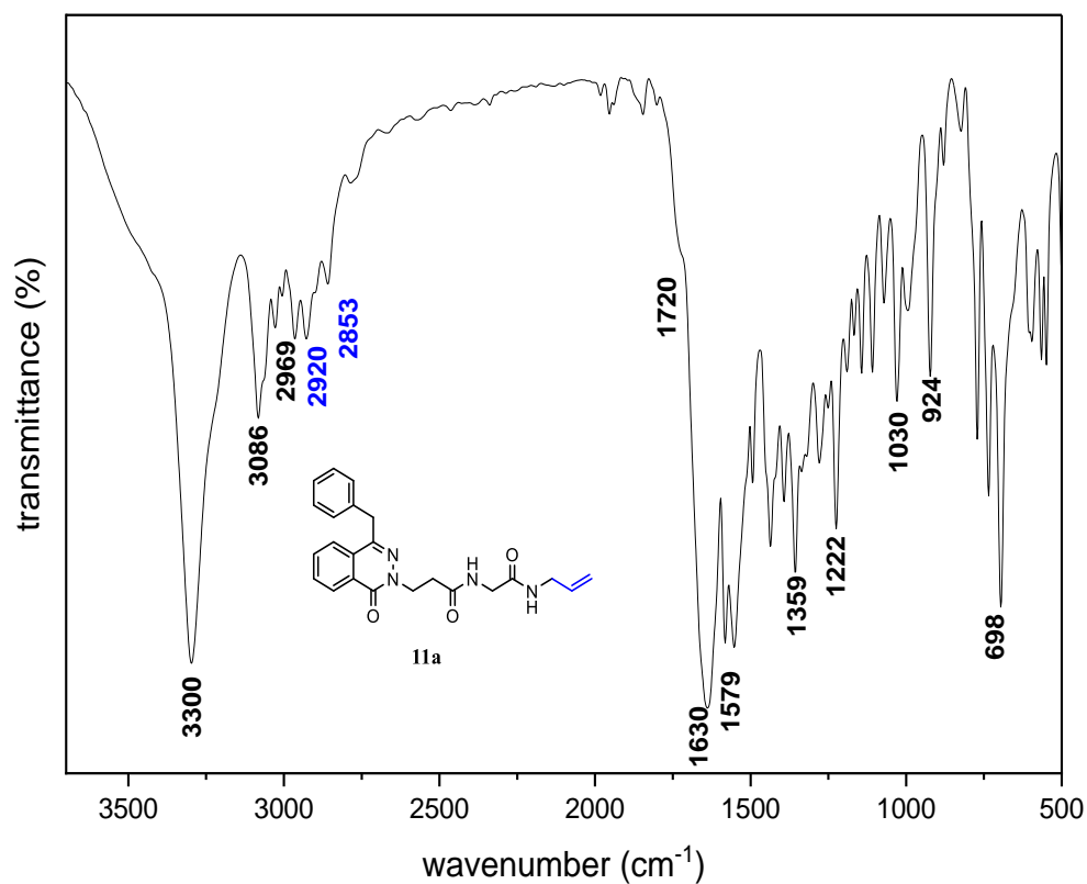
Figure S61: The IR spectrum of compound 11a
