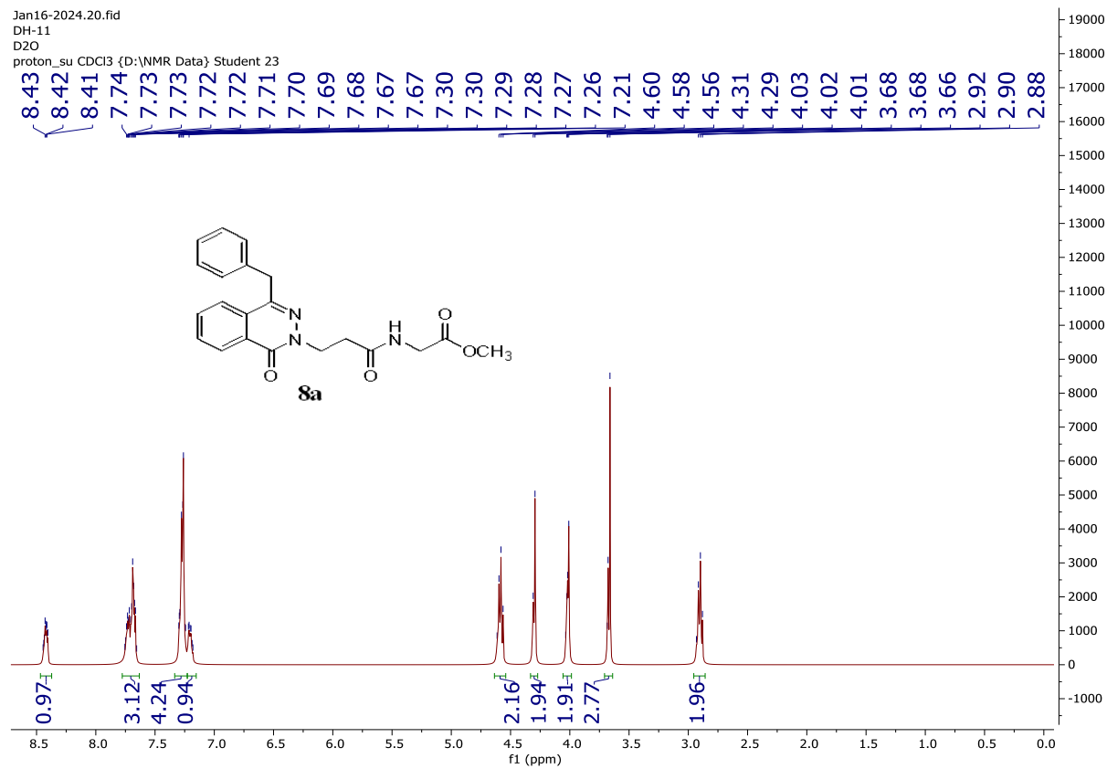
Figure S36 The D 2 O spectrum of compound 8a
