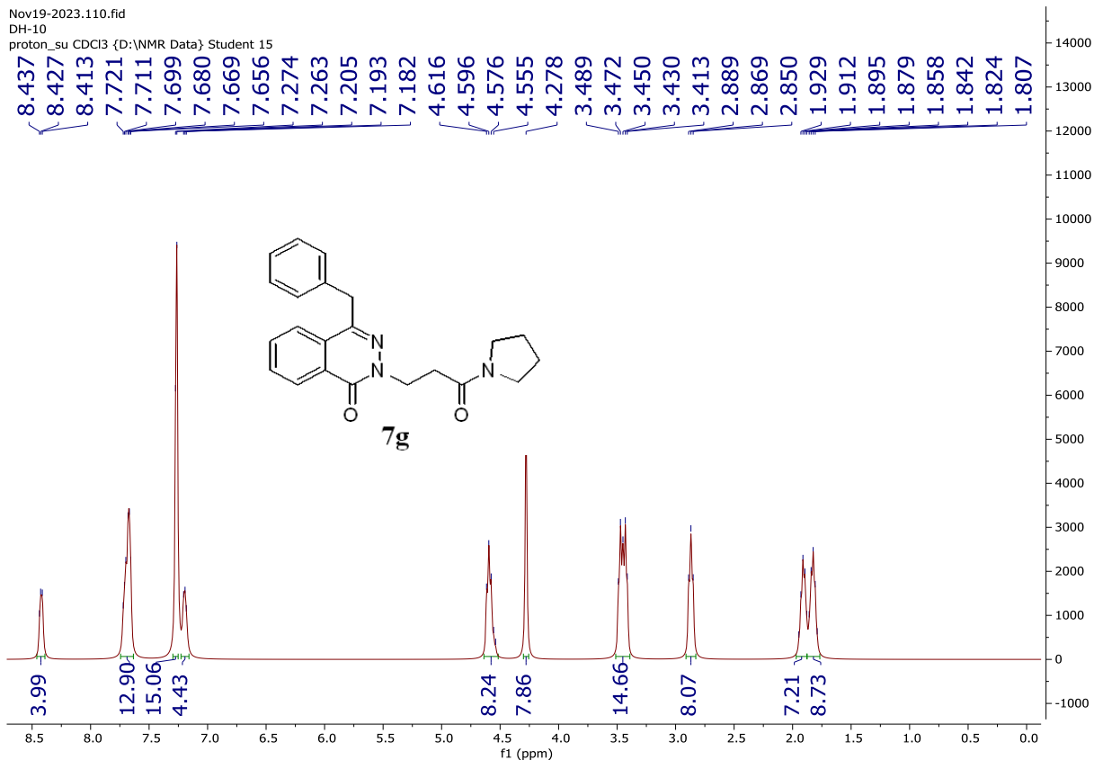
Figure S31 The ^1\text{H} -NMR spectrum of compound 7g
