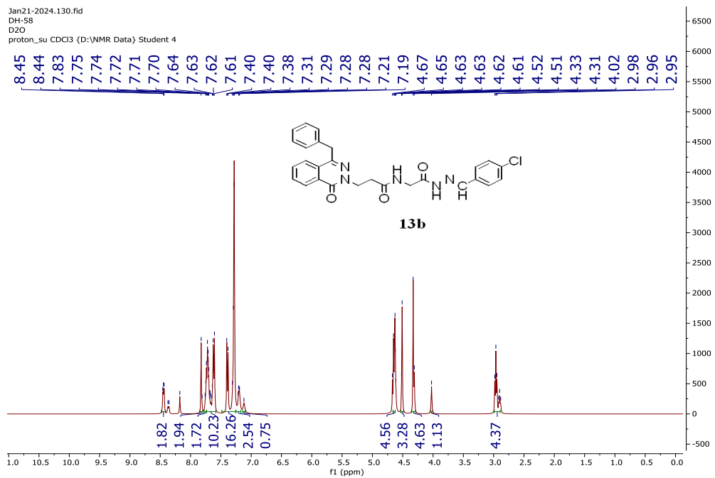
Figure S91: The \text{D}_2\text{O} spectrum of compound 13b
