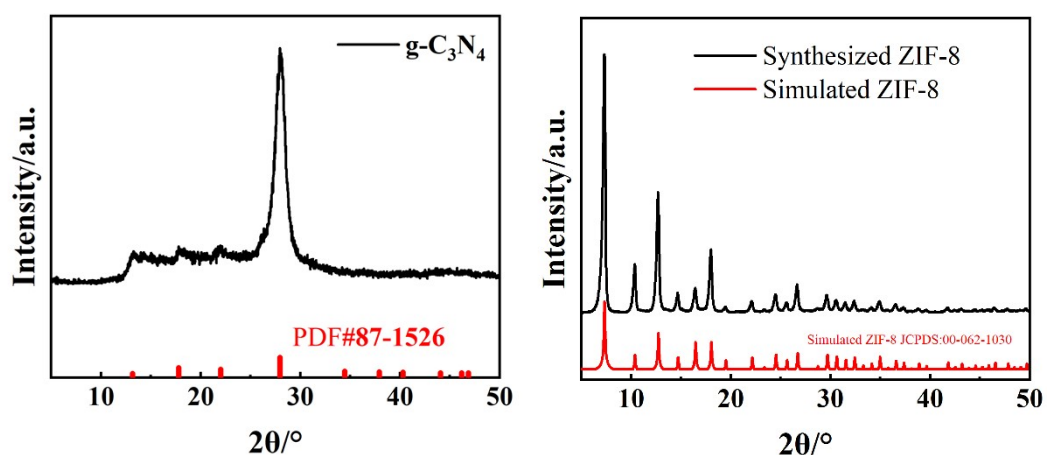
Figure S1 The standard PDF card of g-C 3 N 4 and Comparison of Simulated XRD with Synthesized XRD for ZIF-8
