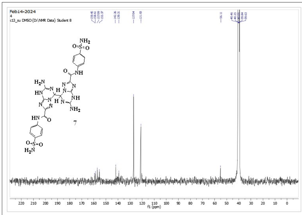
Figure 15: ^{13}\text{C} -NMR Spectrum of compound 7
