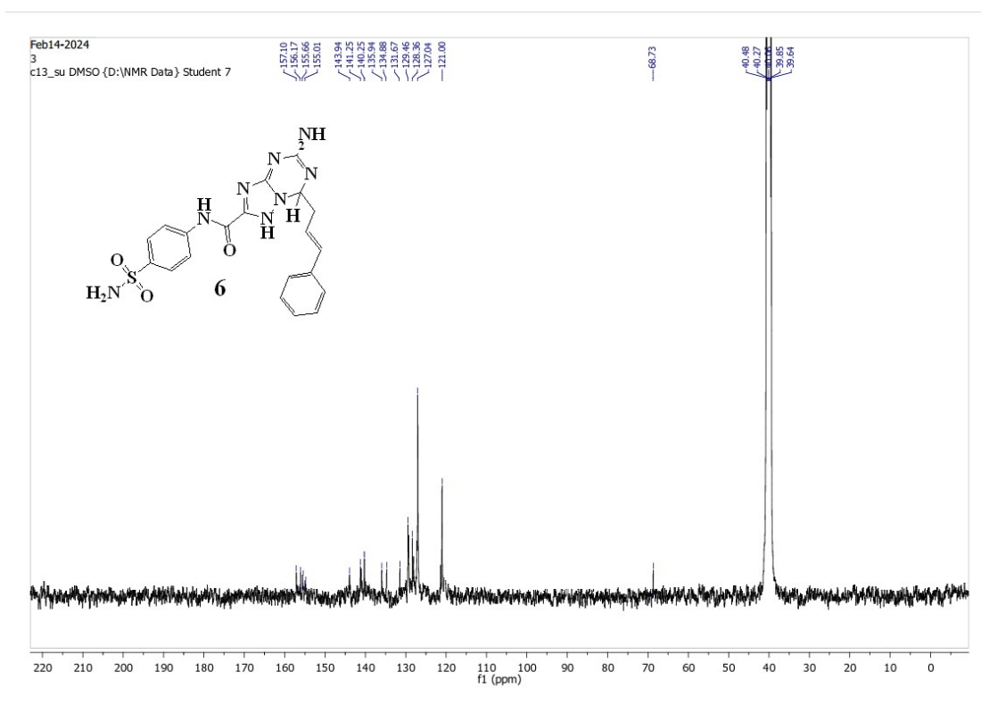
Figure 12: ^{13}\text{C} NMR Spectrum of compound 6
