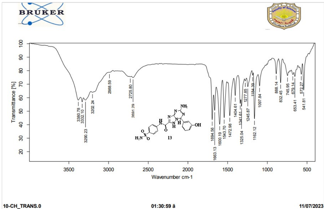
Figure 33: IR Spectrum of compound 13
