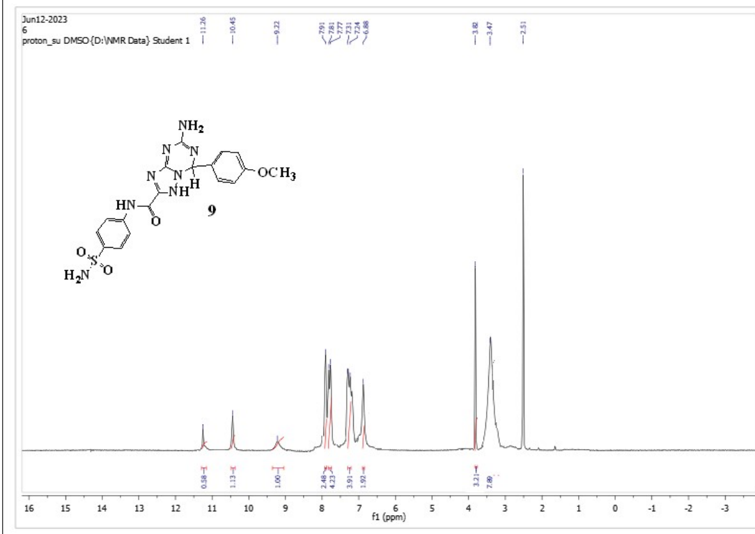
Figure 21: ^1\text{H} NMR Spectrum of compound 9
