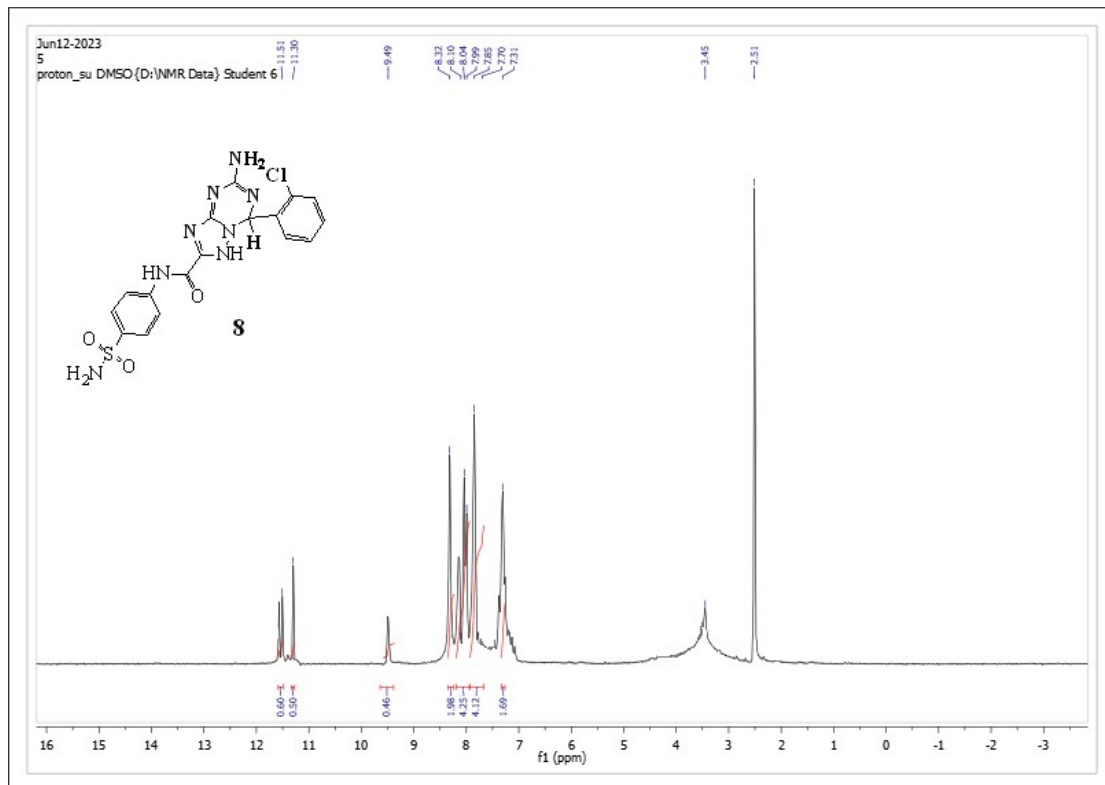
Figure 18: 1 H NMR Spectrum of compound 8
