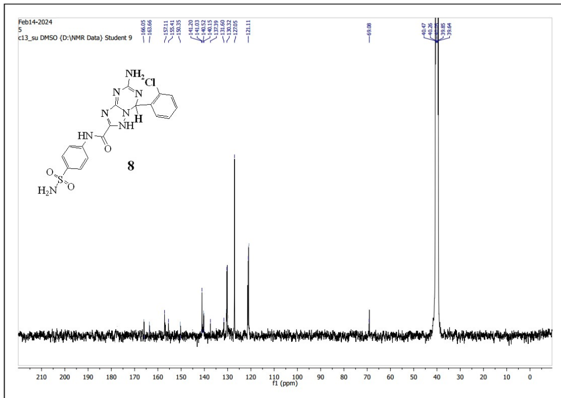
Figure 19: ^{13}\text{C} NMR Spectrum of compound 8
