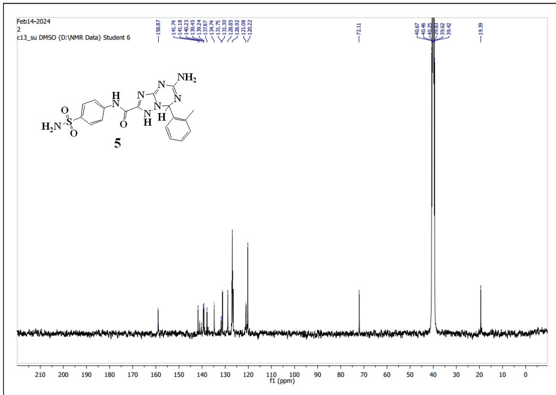
Figure 9: ^{13}\text{C} NMR Spectrum of compound 5
