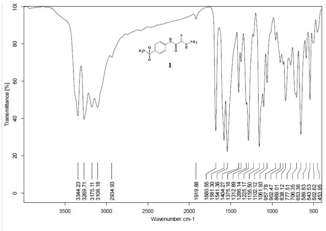
Figure 1: IR Spectrum of compound 1
