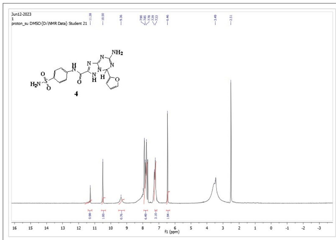
Figure 4: 1 H NMR Spectrum of compound 4
