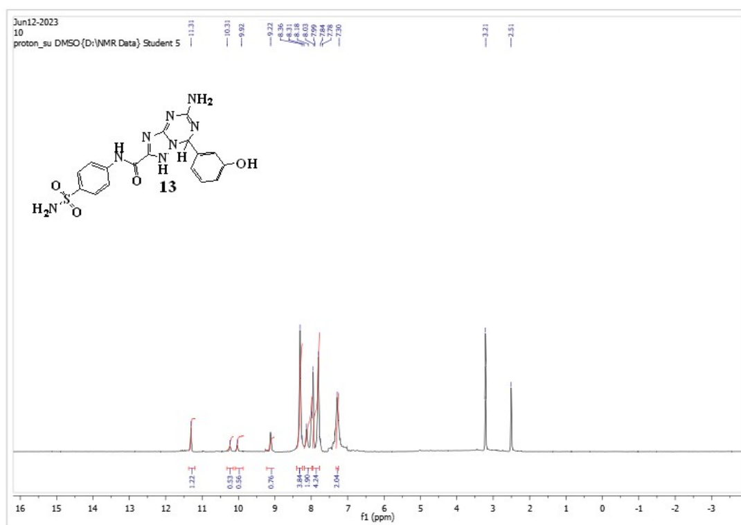
Figure 34: 1 H NMR Spectrum of compound 13
