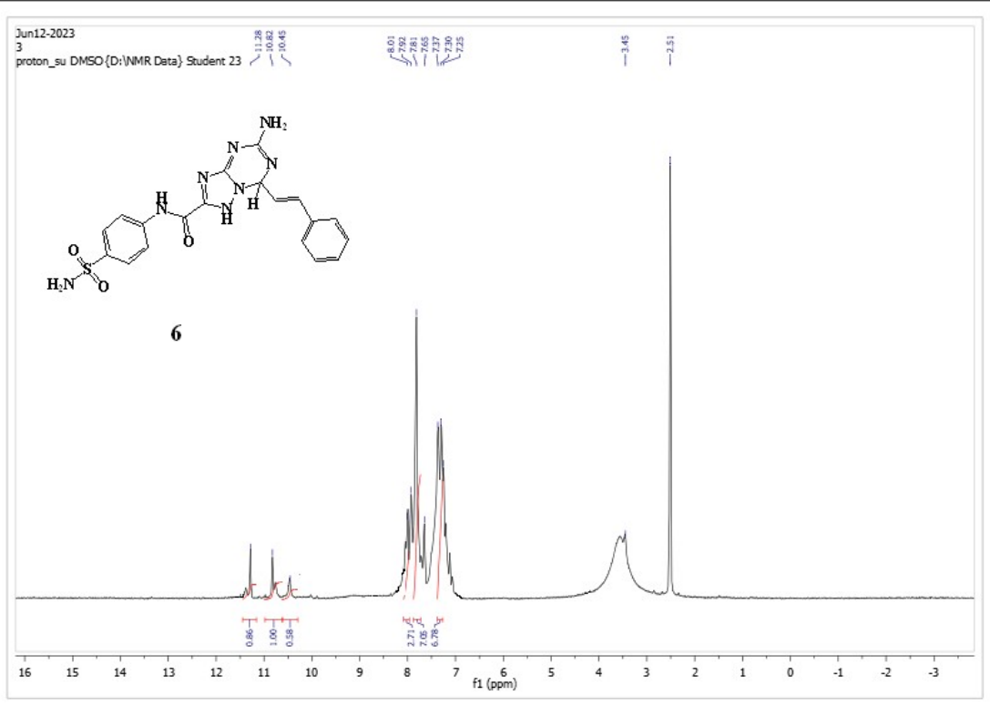
Figure 11: ^1\text{H} NMR Spectrum of compound 6
