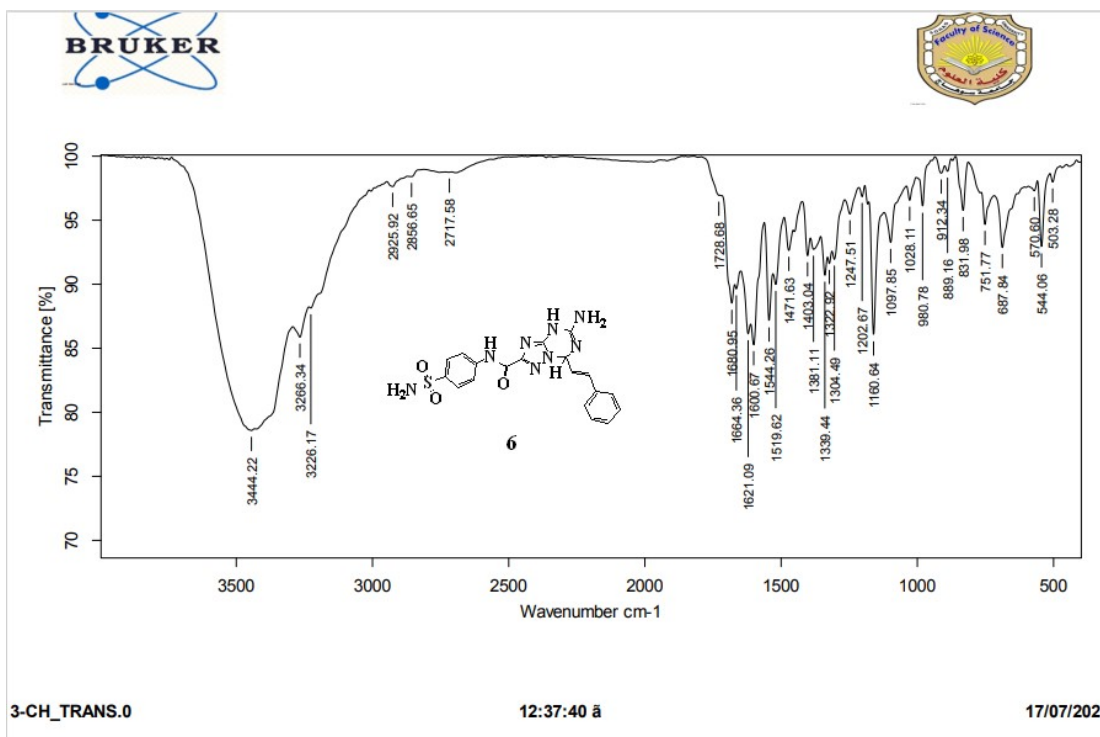
Figure 10: IR Spectrum of compound 6
