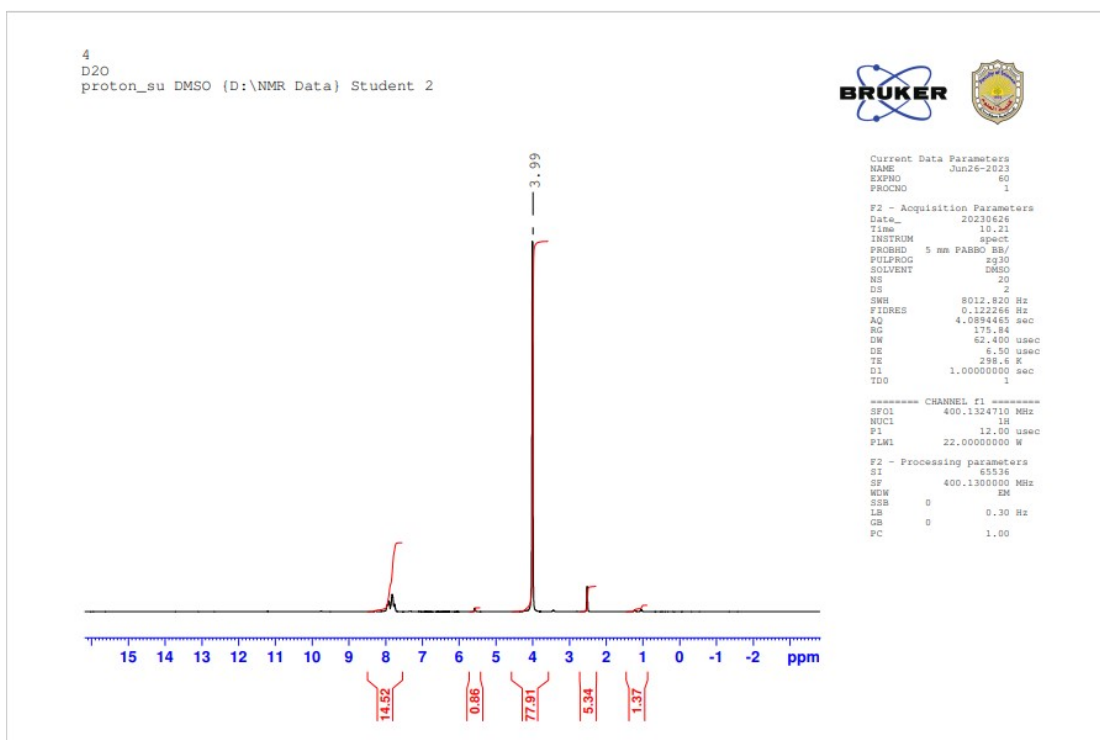
Figure 16: \text{D}_2\text{O} Spectrum of compound 8
