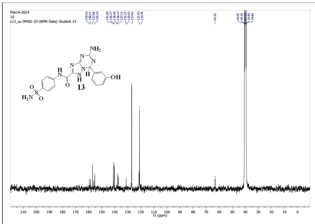
Figure 35: ^{13}\text{C} NMR Spectrum of compound 13
