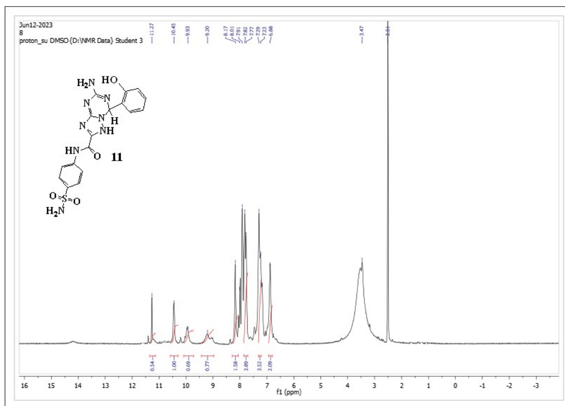
Figure 28: 1 H NMR Spectrum of compound 11
