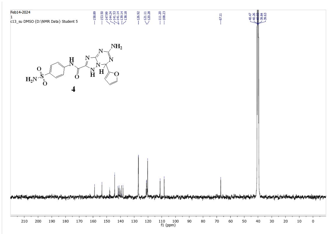
Figure 5: ^{13}\text{C} NMR Spectrum of compound 4
