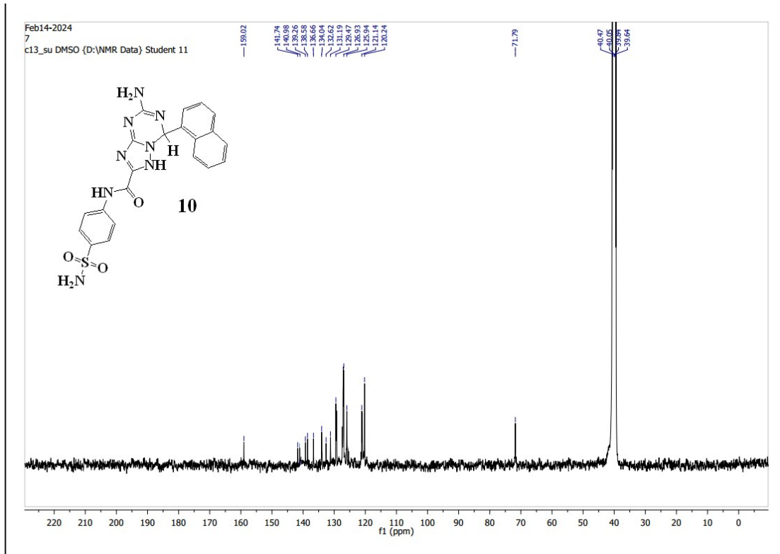
Figure 25: ^{13}\text{C} NMR Spectrum of compound 10
