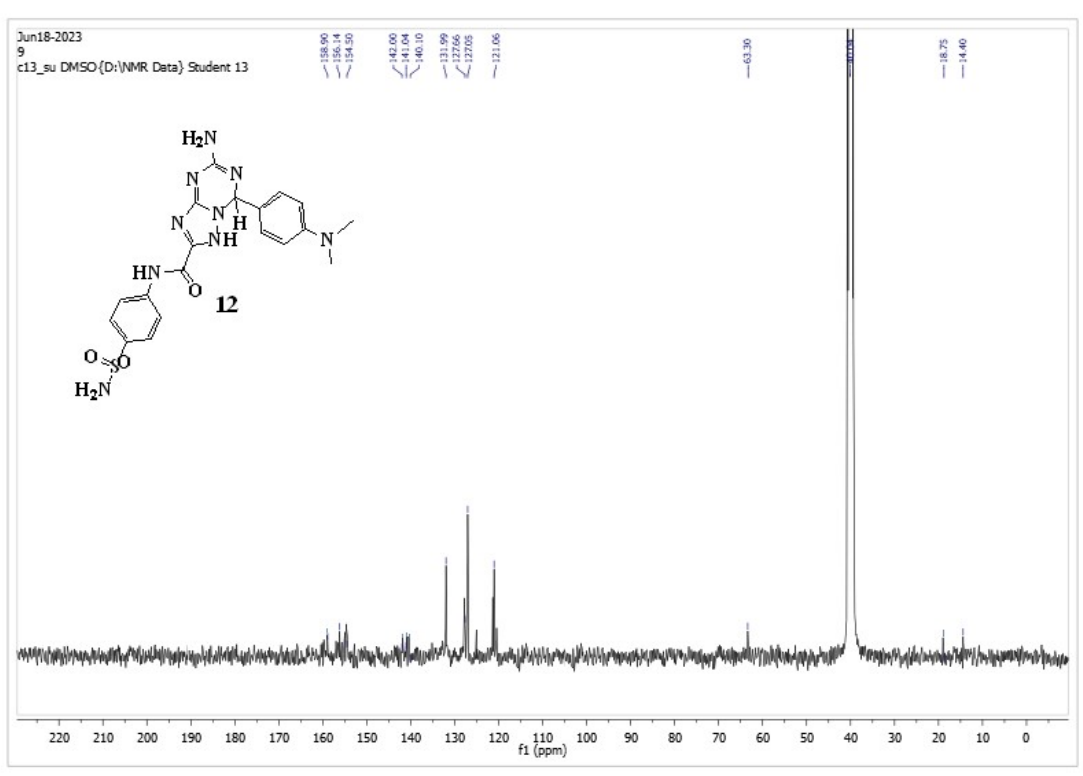
Figure 32: ^{13}\text{C} NMR Spectrum of compound 12
