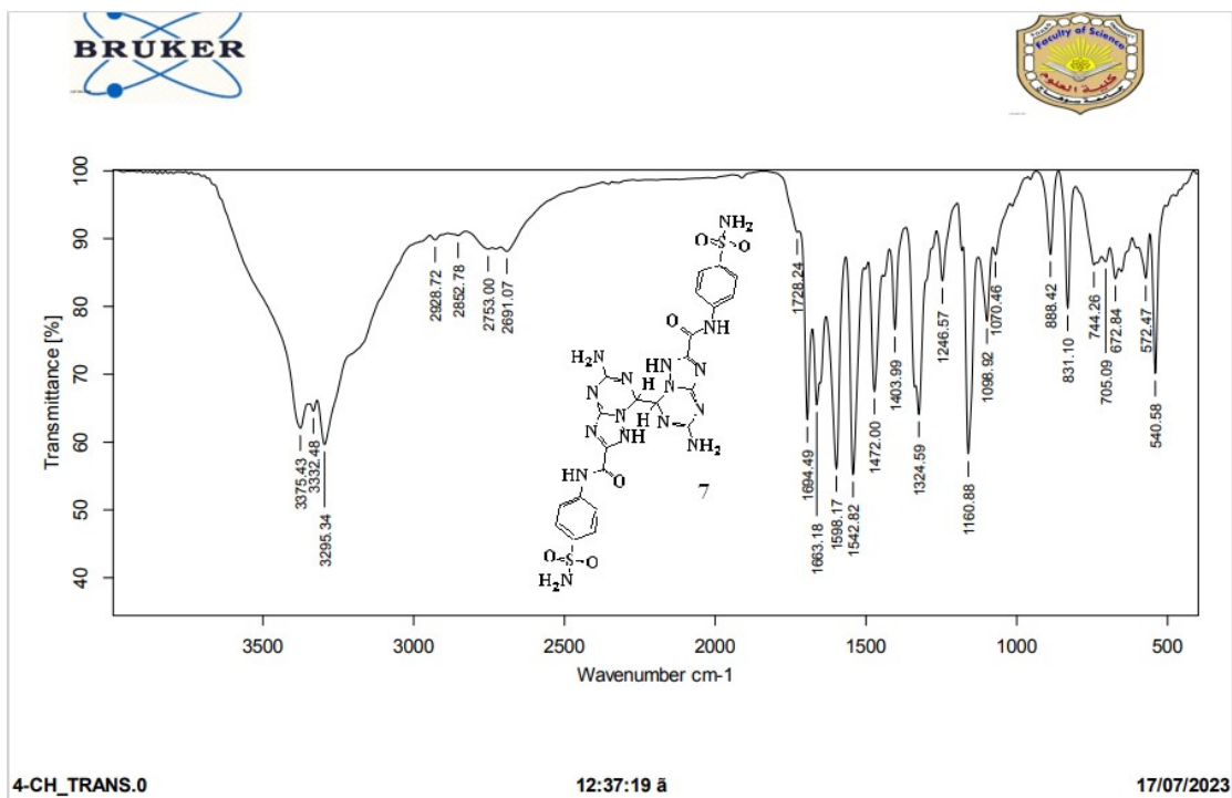
Figure 13: IR Spectrum of compound 7
