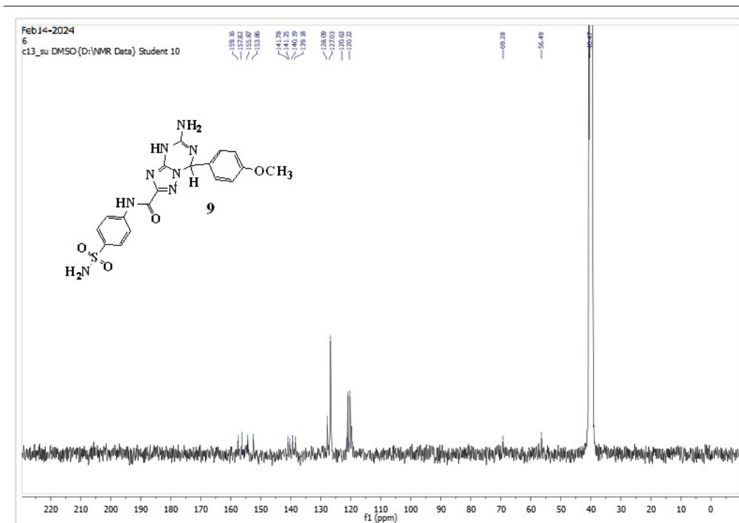
Figure 22: ^{13}\text{C} NMR Spectrum of compound 9
