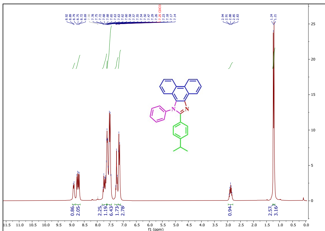
^1\text{H} NMR spectrum of 2-(4-isopropylphenyl)-1-phenyl-1H-phenanthro[9,10-d]imidazole ( a5 ):
