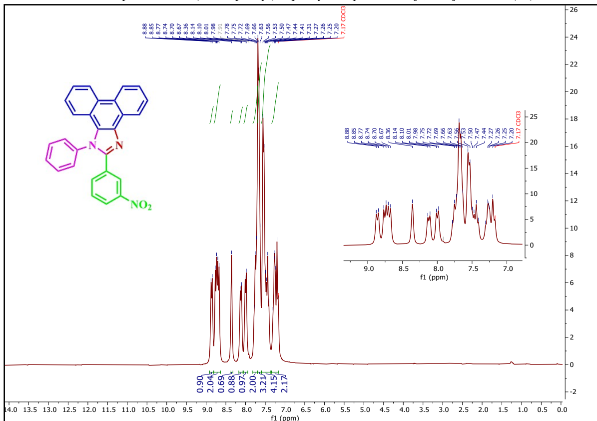
^1\text{H} NMR spectrum of 2-(3-nitrophenyl)-1-phenyl-1H-phenanthro[9,10-d]imidazole ( a1 ):
