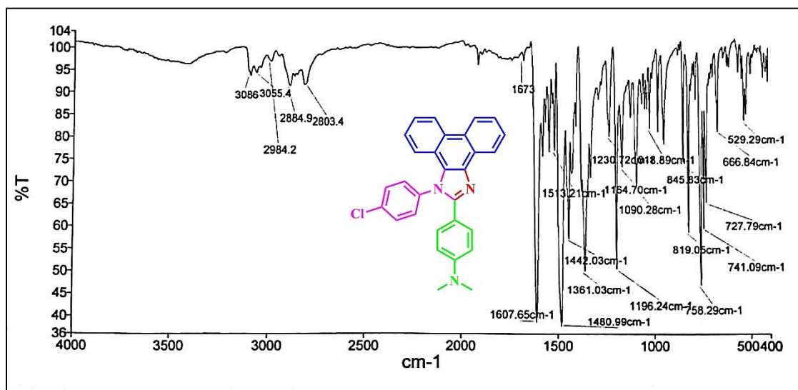
FT-IR spectrum of 4-(1-(4-chlorophenyl)-1 H -phenanthro[9,10- d ]imidazol-2-yl)- N,N -dimethylaniline ( a12 ):
