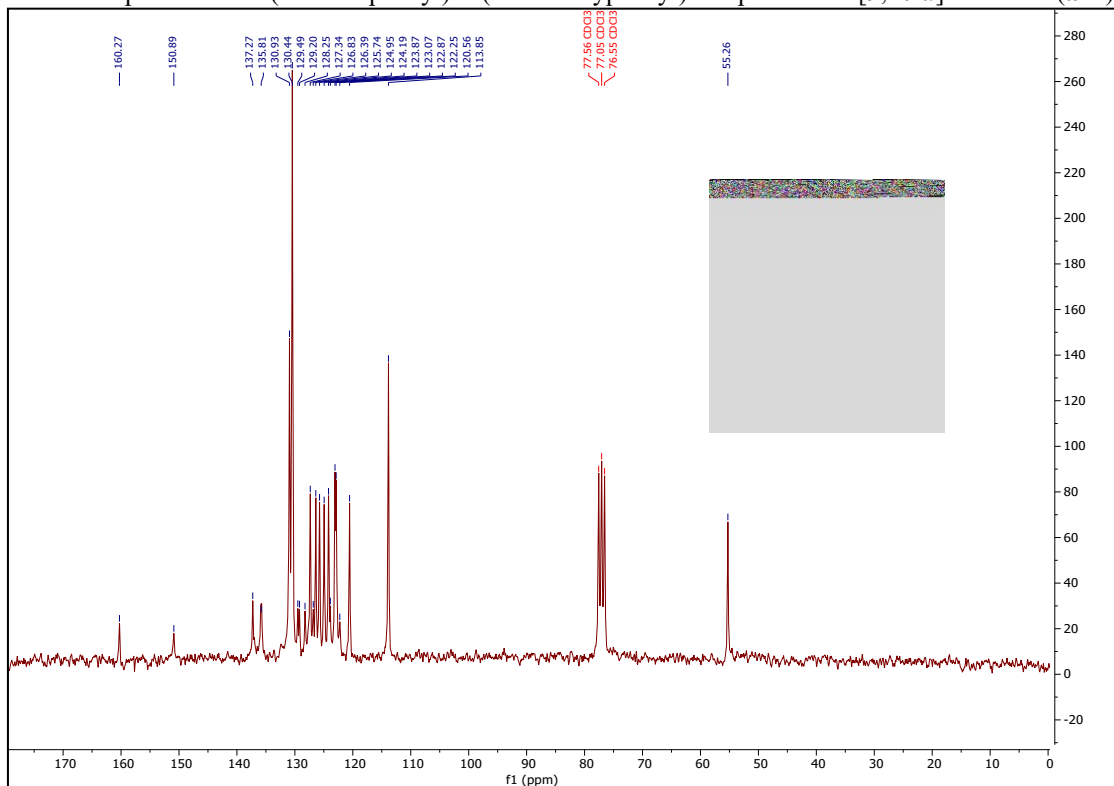
13 CNMR spectrum of 1-(4-chlorophenyl)-2-(4-methoxyphenyl)-1 H -phenanthro[9,10- d ]imidazole ( a11 ):
