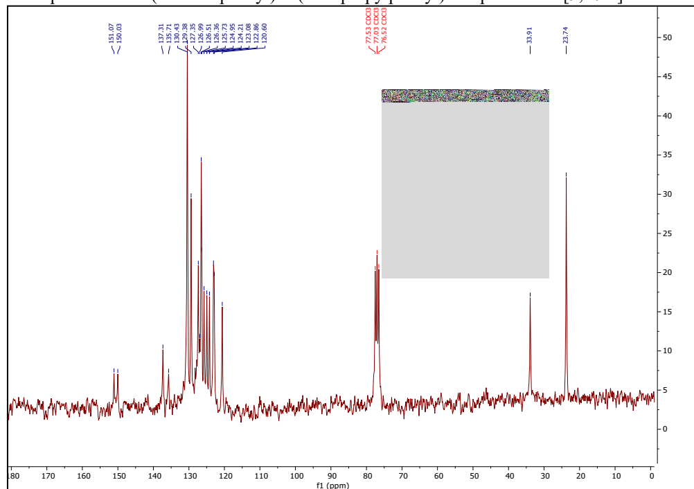
^{13}\text{C} NMR spectrum of 1-(4-chlorophenyl)-2-(4-isopropylphenyl)-1H-phenanthro[9,10-d]imidazole ( a2 ):
