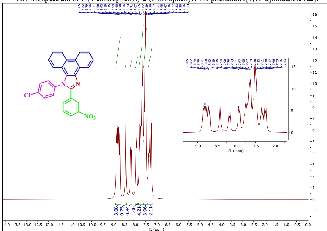
1 HNMR spectrum of 1-(4-chlorophenyl)-2-(3-nitrophenyl)-1H-phenanthro[9,10-d]imidazole ( a3 ):
