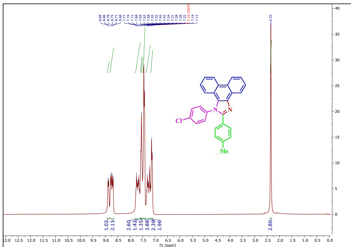
1 H NMR spectrum of 1-(4-chlorophenyl)-2-(p-tolyl)-1H-phenanthro[9,10-d]imidazole ( a4 ):
