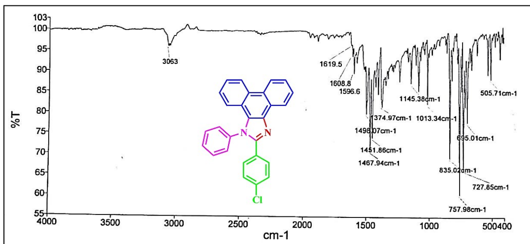
FT-IR spectrum of 2-(4-chlorophenyl)-1-phenyl-1H-phenanthro[9,10-d]imidazole ( a8 ):
