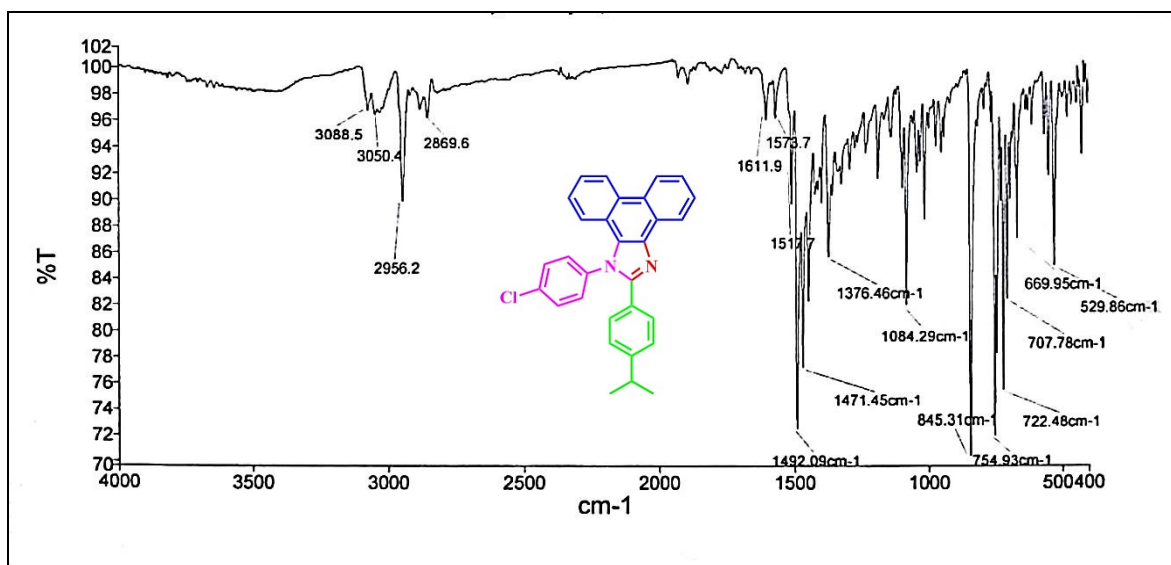
FT-IR spectrum of 1-(4-chlorophenyl)-2-(4-isopropylphenyl)-1H-phenanthro[9,10-d]imidazole ( a2 ):
