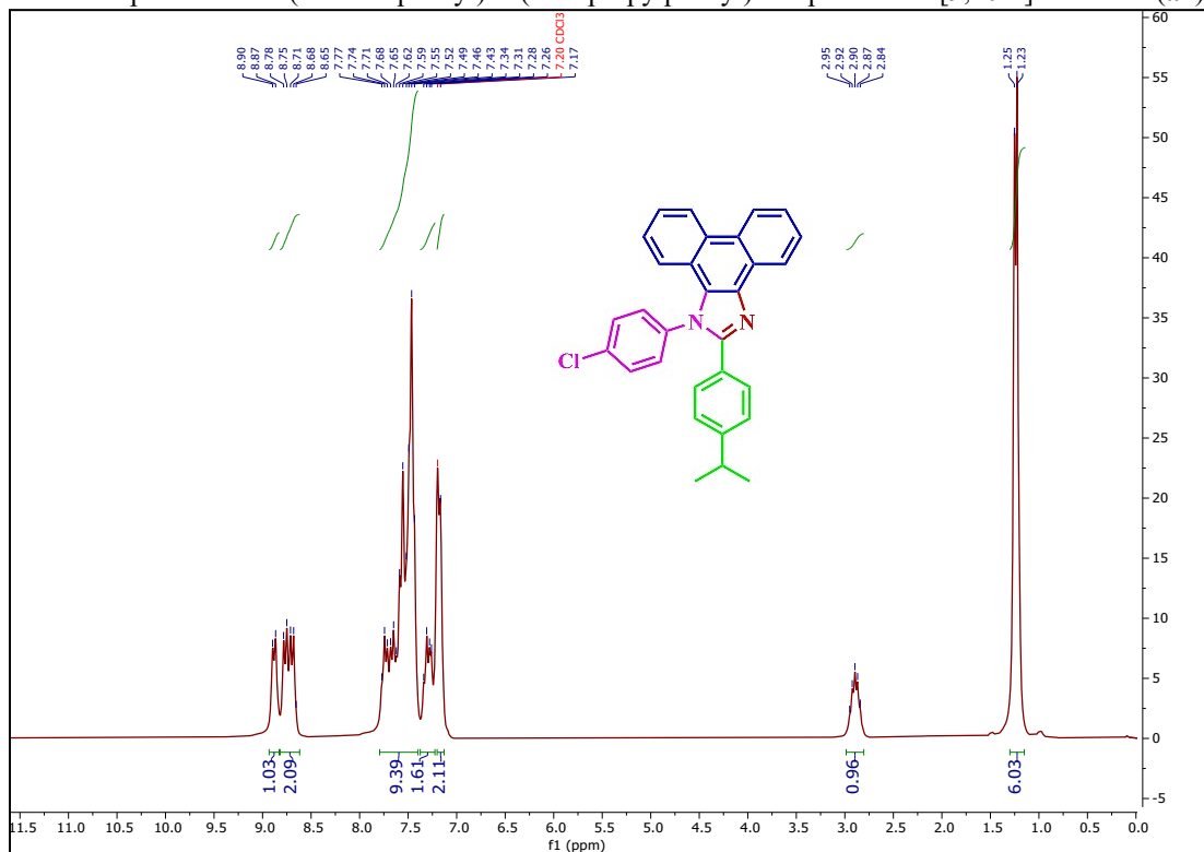
1 H NMR spectrum of 1-(4-chlorophenyl)-2-(4-isopropylphenyl)-1H-phenanthro[9,10-d]imidazole ( a2 ):
