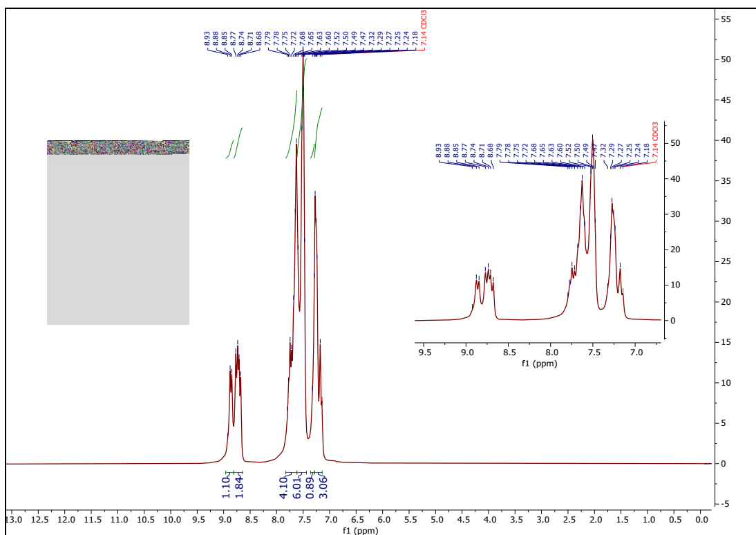
1 HNMR spectrum of 2-(4-chlorophenyl)-1-phenyl-1H-phenanthro[9,10-d]imidazole ( a8 ):
