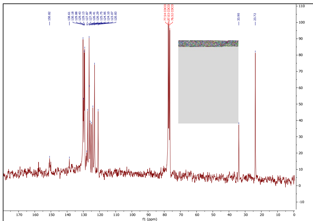
13 CNMR spectrum of 2-(4-isopropylphenyl)-1-phenyl-1H-phenanthro[9,10-d]imidazole ( a5 ):
