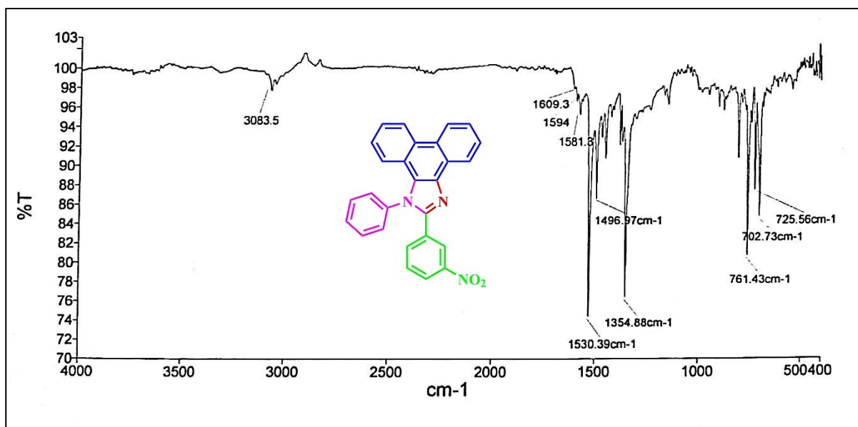
FT-IR spectrum of 2-(3-nitrophenyl)-1-phenyl-1H-phenanthro[9,10-d]imidazole ( a1 ):
