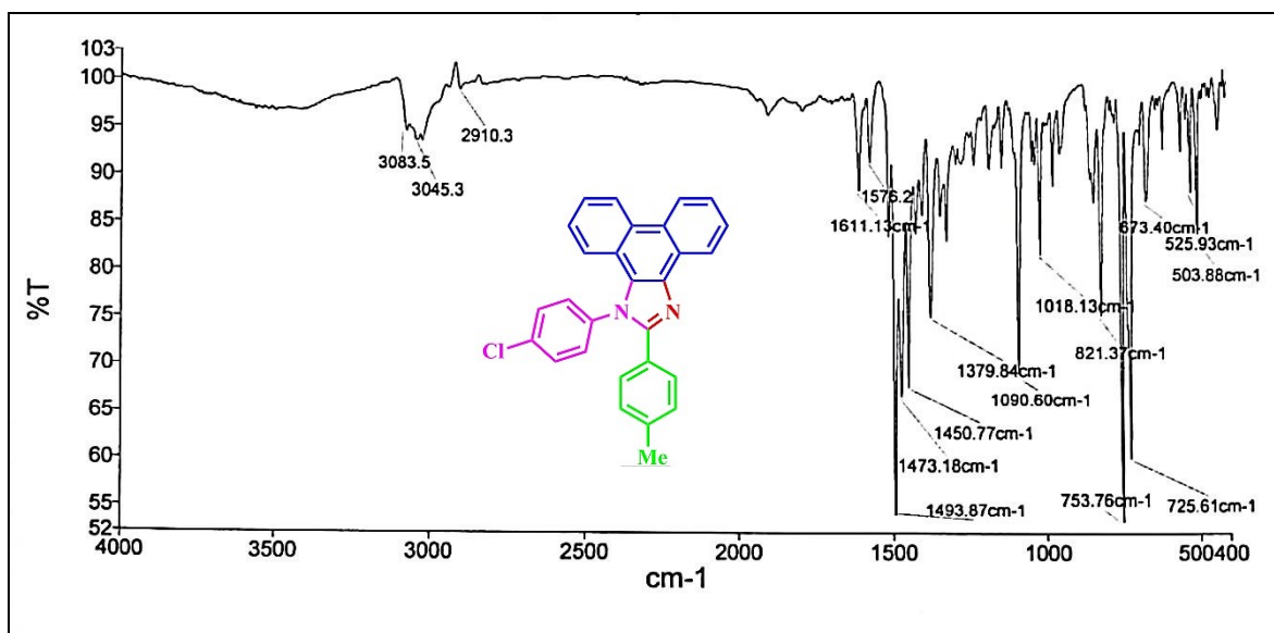
FT-IR spectrum of 1-(4-chlorophenyl)-2-(p-tolyl)-1H-phenanthro[9,10-d]imidazole ( a4 ):
