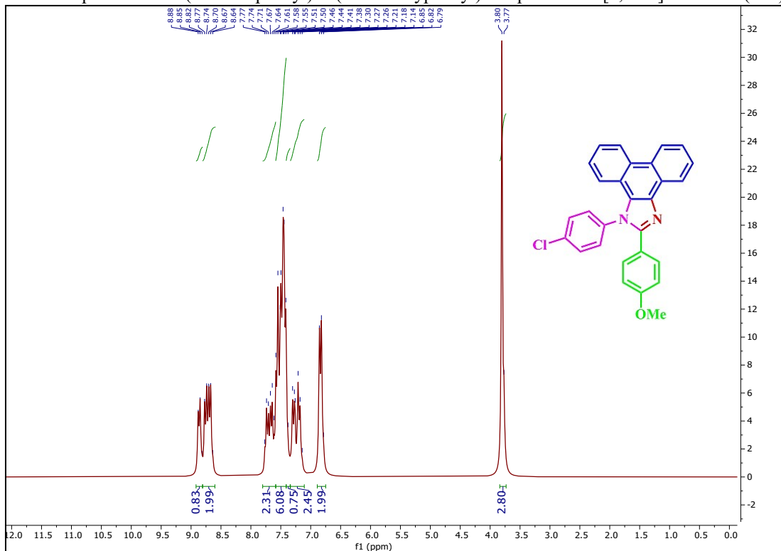
1 H NMR spectrum of 1-(4-chlorophenyl)-2-(4-methoxyphenyl)-1H-phenanthro[9,10-d]imidazole ( a11 ):
