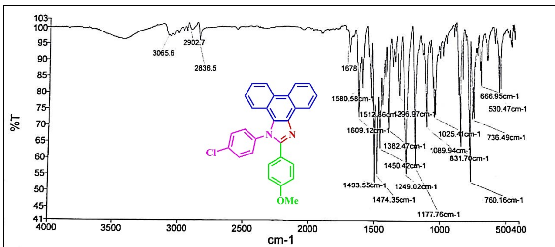
FT-IR spectrum of 1-(4-chlorophenyl)-2-(4-methoxyphenyl)-1H-phenanthro[9,10-d]imidazole ( a11 ):
