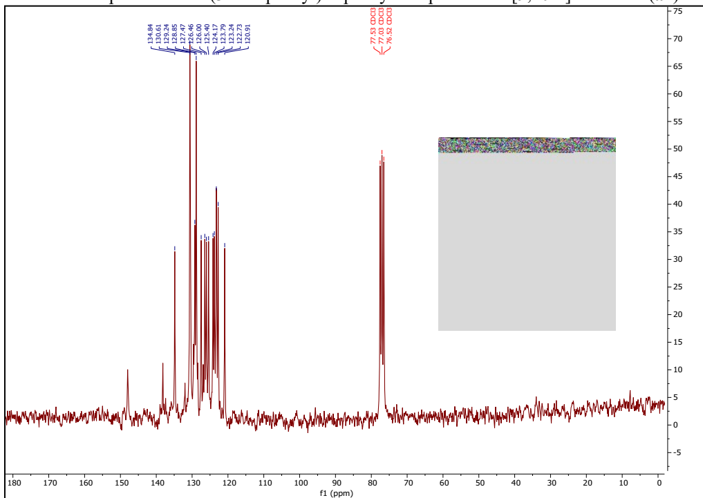
^{13}\text{C} NMR spectrum of 2-(3-nitrophenyl)-1-phenyl-1H-phenanthro[9,10-d]imidazole ( a1 ):
