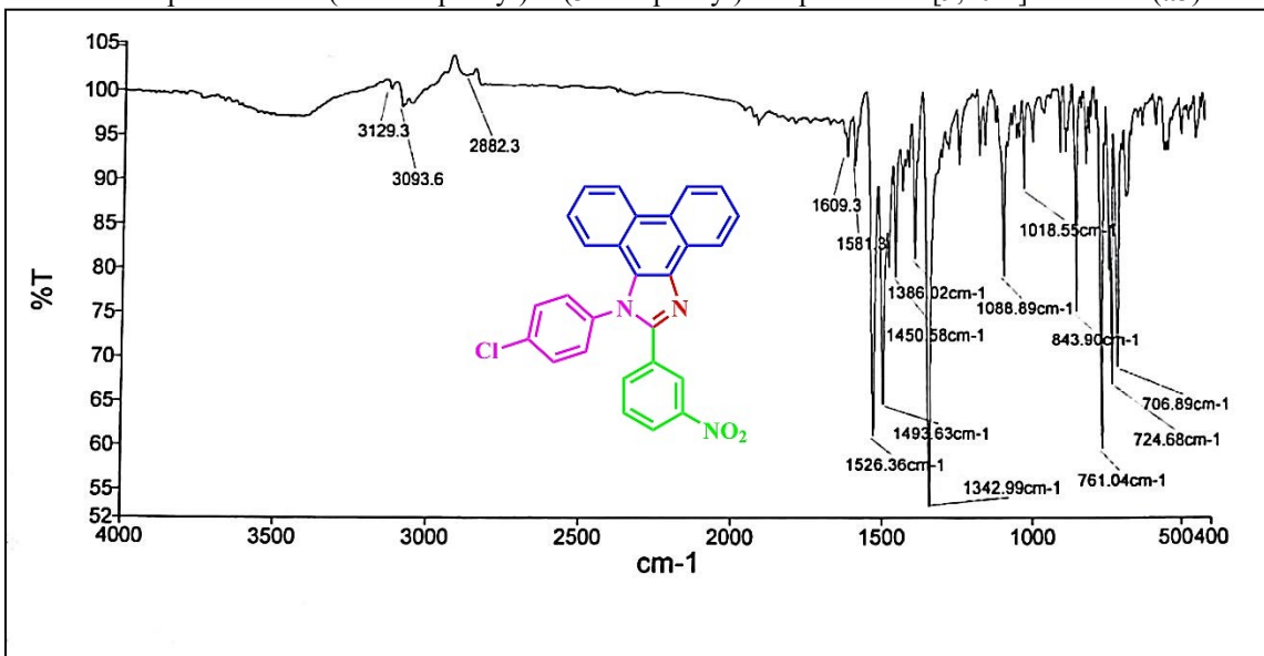
FT-IR spectrum of 1-(4-chlorophenyl)-2-(3-nitrophenyl)-1H-phenanthro[9,10-d]imidazole ( a3 ):
