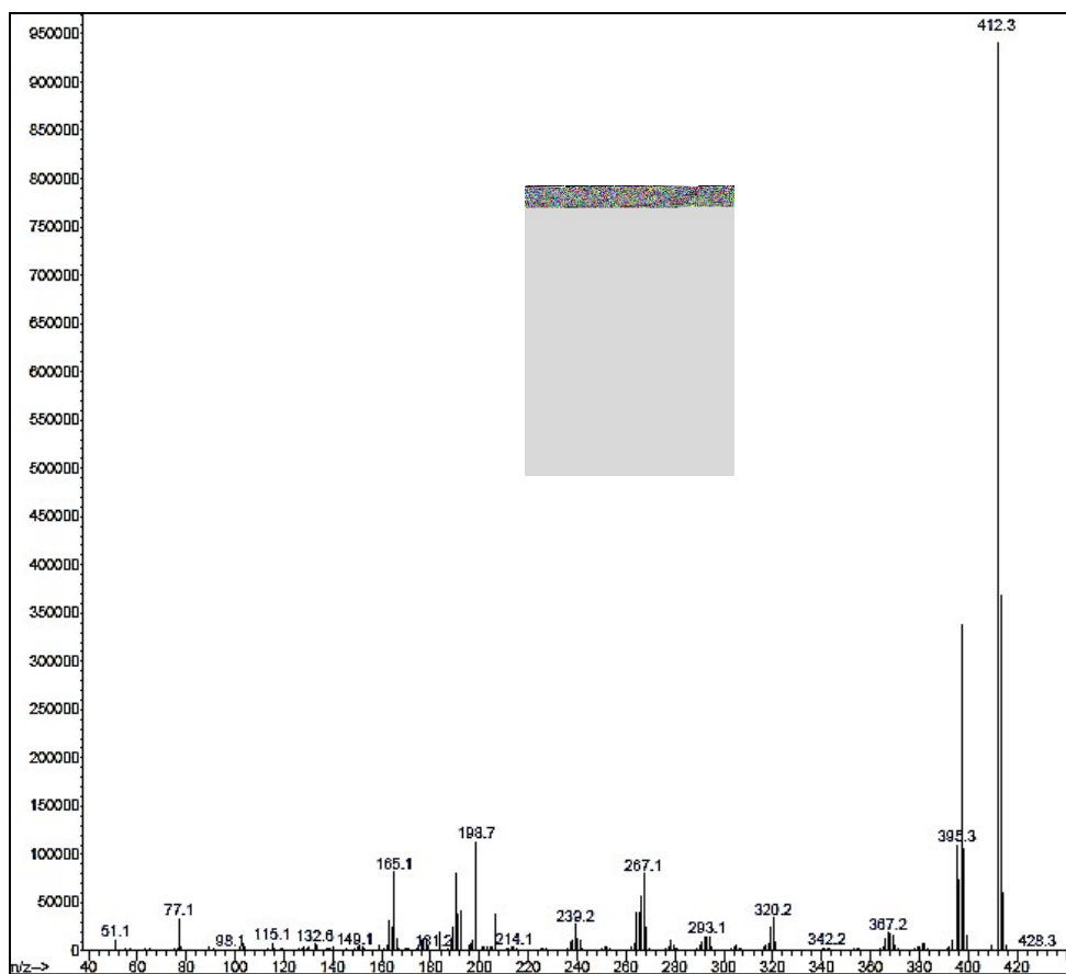
Mass spectrum of 2-(4-isopropylphenyl)-1-phenyl-1H-phenanthro[9,10-d]imidazole ( a5 ):
