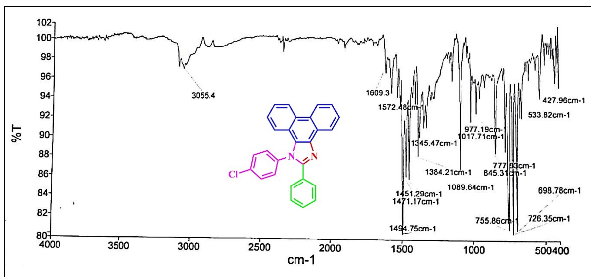
FT-IR spectrum of 1-(4-chlorophenyl)-2-phenyl-1H-phenanthro[9,10-d]imidazole ( a10 ):
