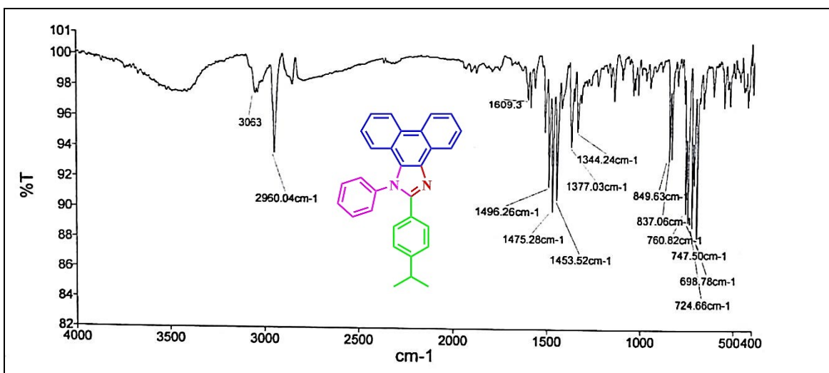
FT-IR spectrum of 2-(4-isopropylphenyl)-1-phenyl-1H-phenanthro[9,10-d]imidazole ( a5 ):
