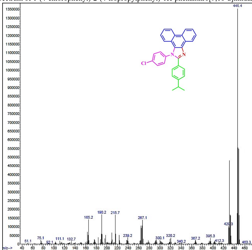
Mass spectrum of 1-(4-chlorophenyl)-2-(4-isopropylphenyl)-1H-phenanthro[9,10-d]imidazole ( a2 ):
