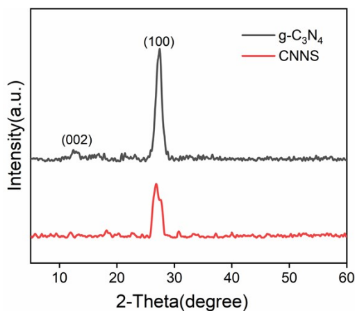
Figure S1. XRD patterns of g-C 3 N 4 and CNNS.
