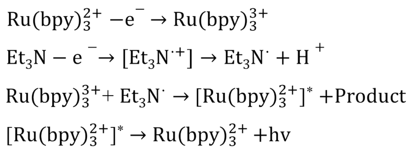
Figure S3. The illustration for the ECL process of Ru(bpy) 3+ /Et 3 N system.
