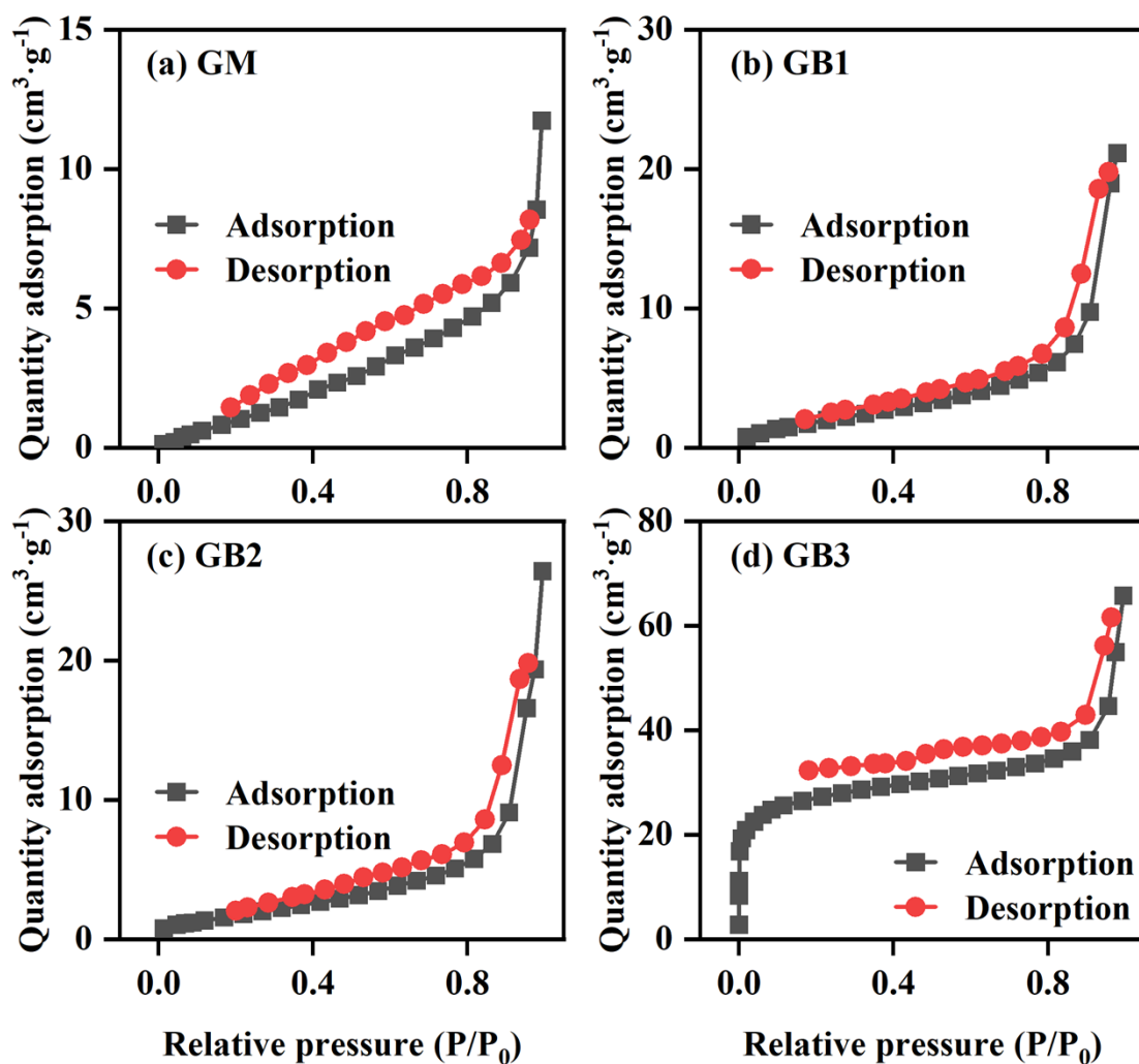
Fig. S1 The N_2 adsorption-desorption curve of grub manure (GM) and grub manure-derived biochar (GB). GB1, GB2 and GB3 represents grub manure-derived biochar produced at 450, 600 and 750 °C, respectively.
