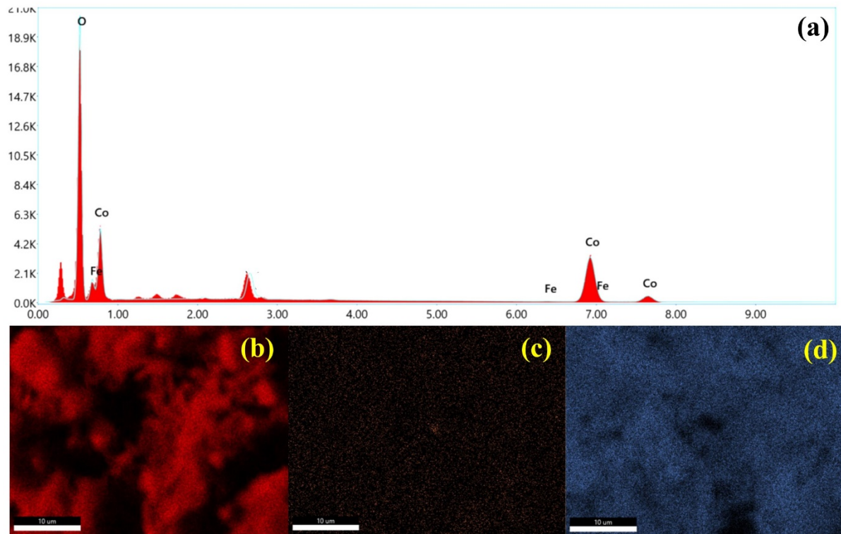
Figure S1- EDX spectra and elemental mapping of FCHNF.
