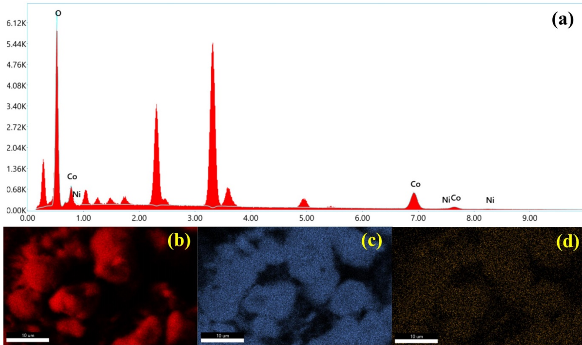
Figure S3-EDX spectra and elemental mapping of NCHNF.
