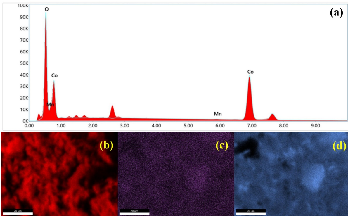
Figure 2-EDX spectra and elemental mapping of MCHNF.
