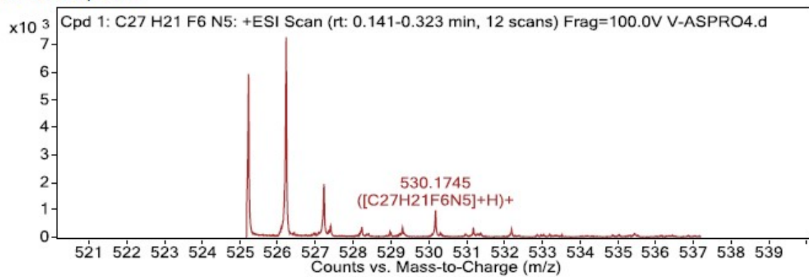
HRMS spectrum of compound 3a .
