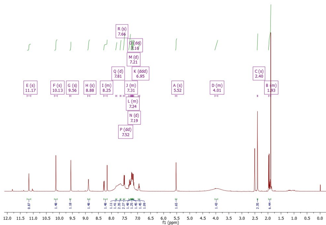
1 H NMR spectrum of compound 3f in DMSO-d 6 .
