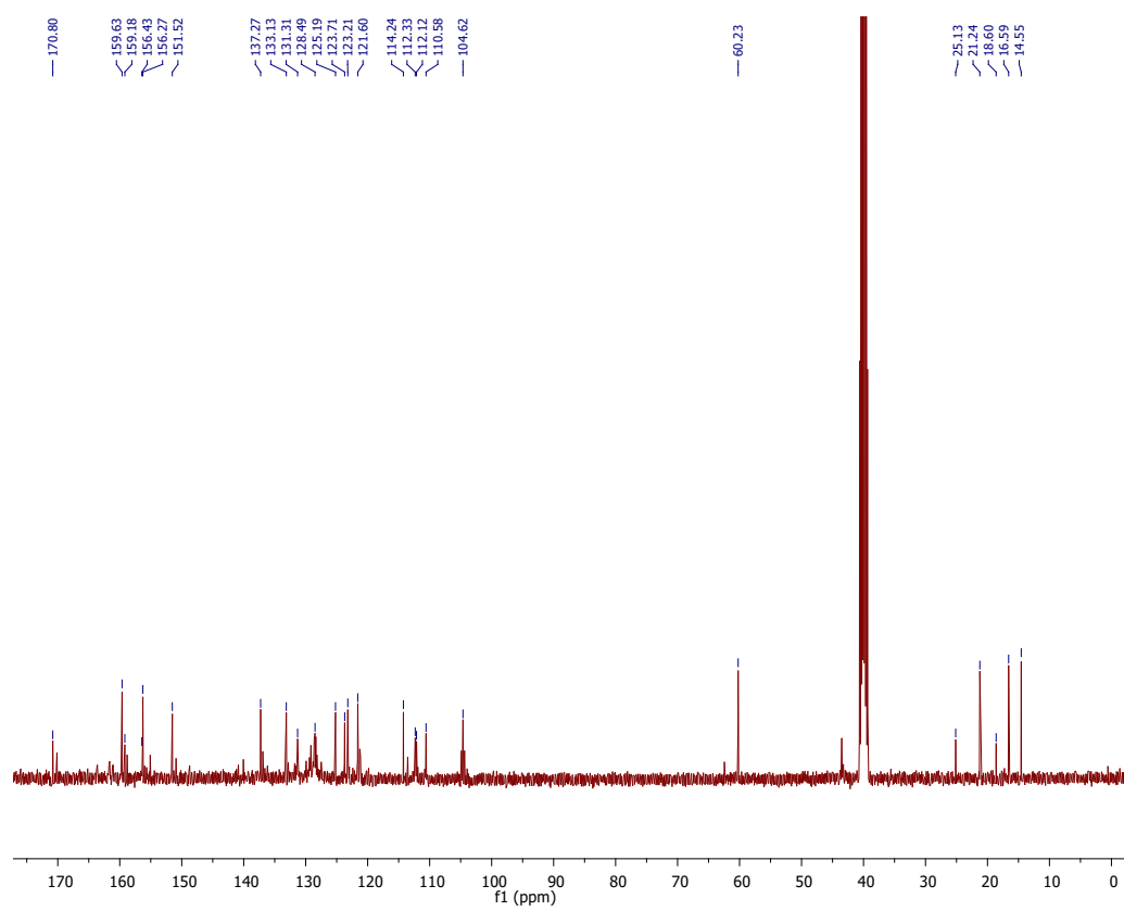
NMR spectrum of compound 2a in DMSO- d_6 .
