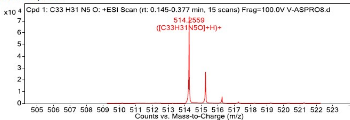
HRMS spectrum of compound 3e .
