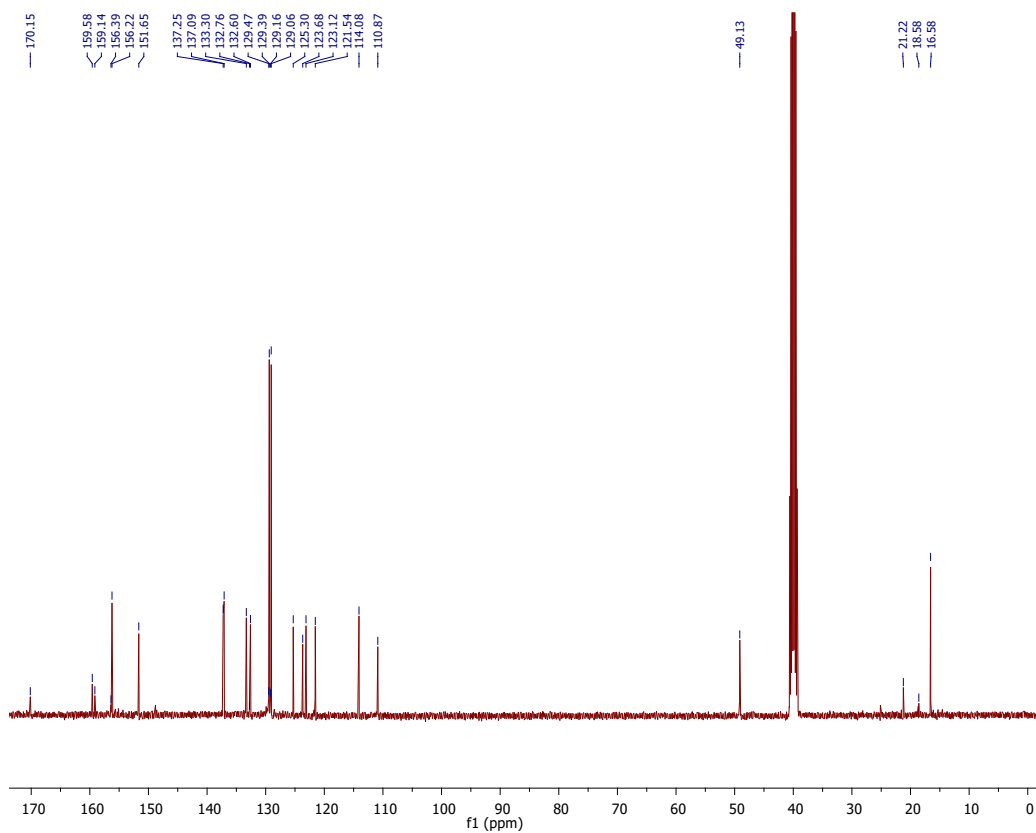
NMR spectrum of compound 2f in \text{DMSO-d}_6 .
