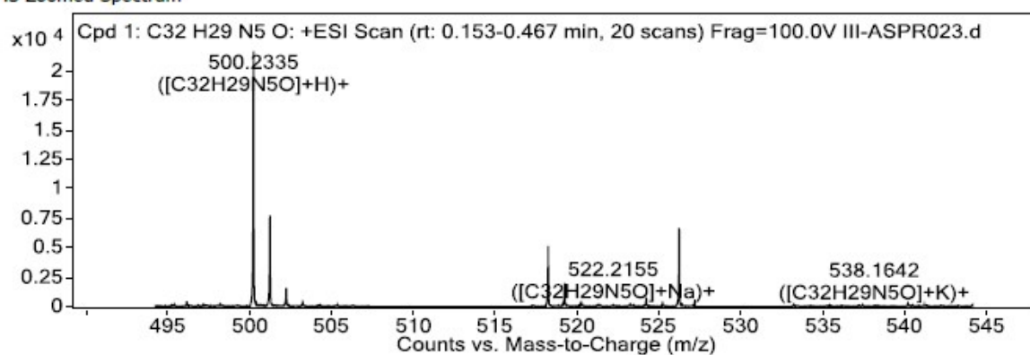
HRMS spectrum of compound 1o .
