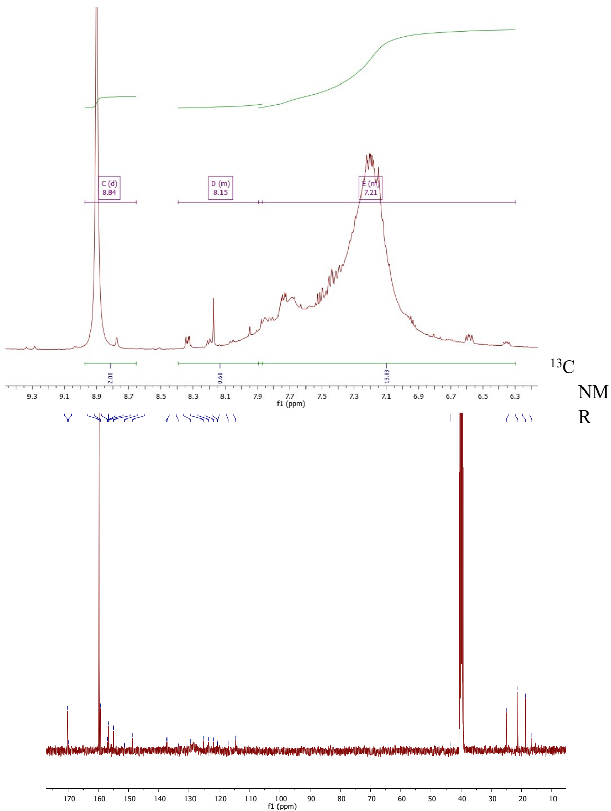
spectrum of compound 2d in DMSO- d_6 .
