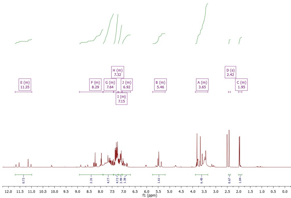
13 C NMR spectrum of compound 1p in DMSO-d 6 .
