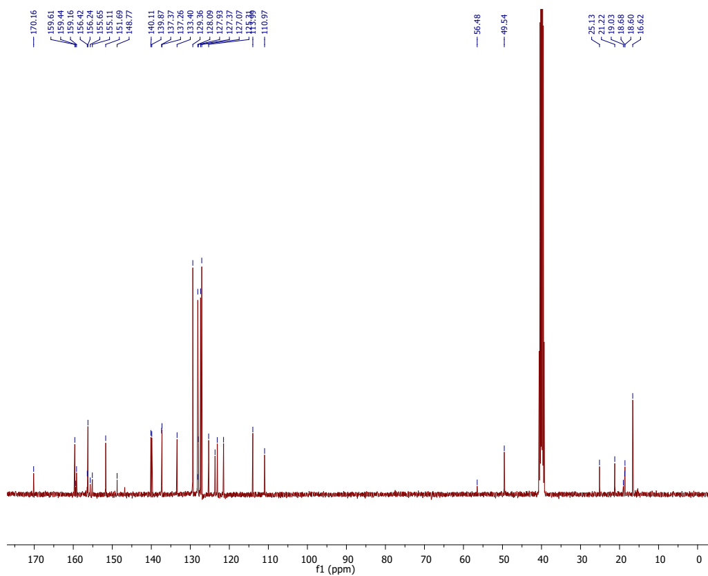
NMR spectrum of compound 3c in \text{DMSO-d}_6 .
