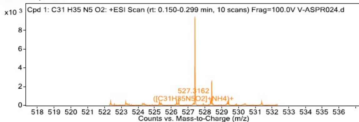
HRMS spectrum of compound 3l .
