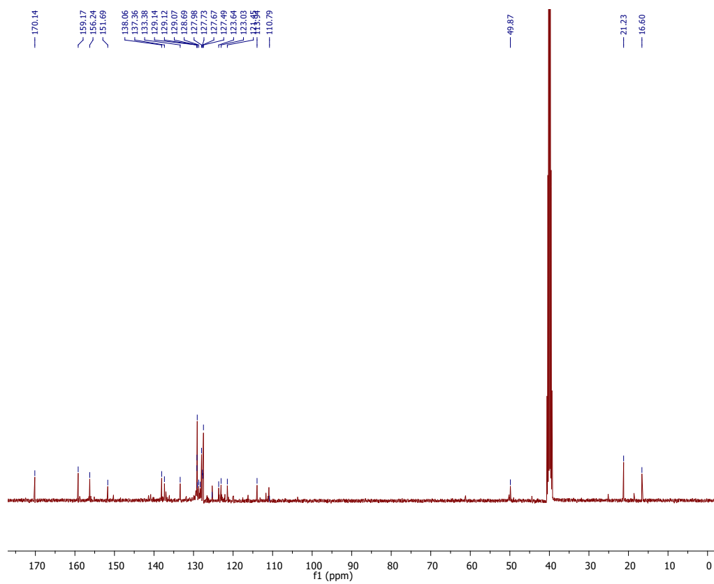
NMR spectrum of compound 11 in \text{DMSO-d}_6 .
