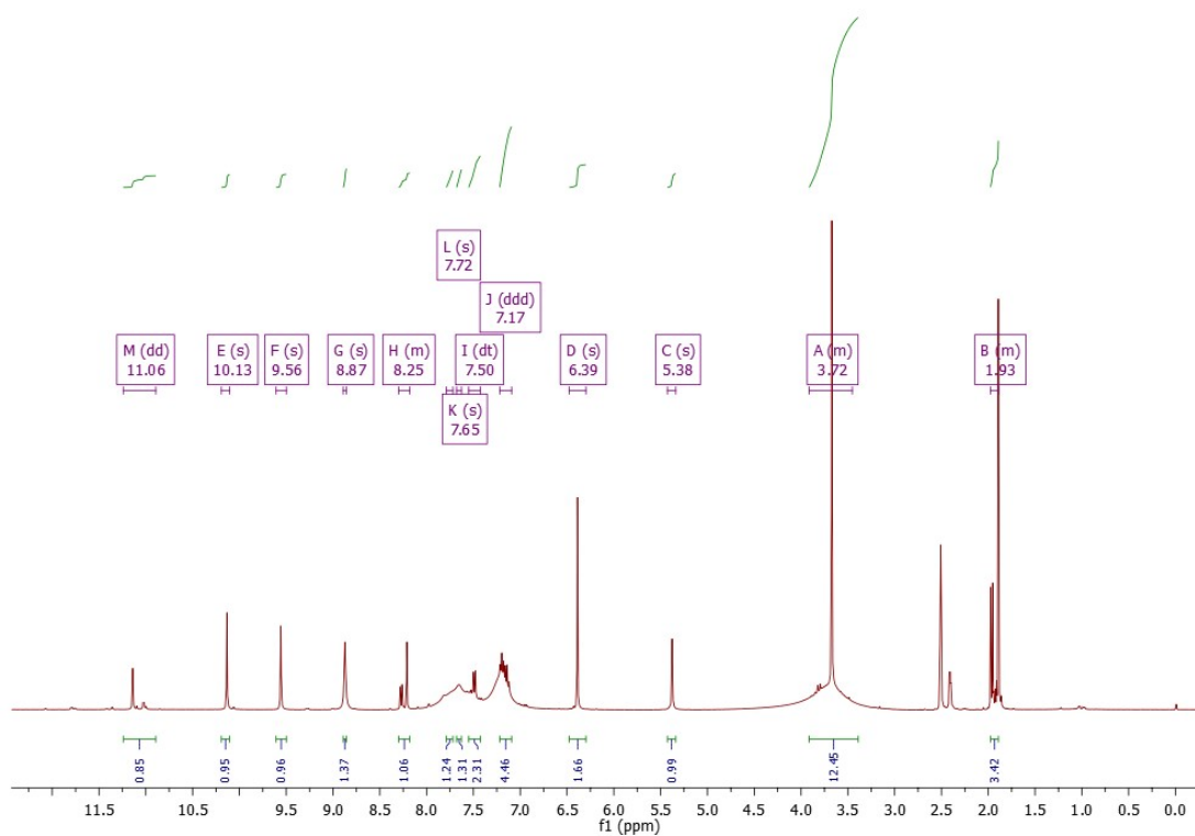
1 H NMR spectrum of compound 3b in DMSO-d 6 .
