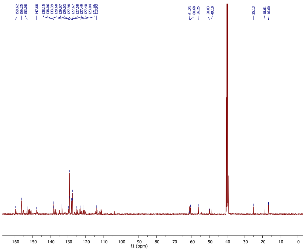
13 C NMR spectrum of compound 1p in DMSO-d 6 .
