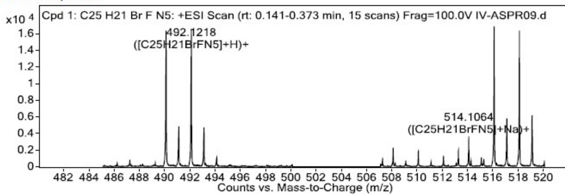
HRMS spectrum of compound 2i .
