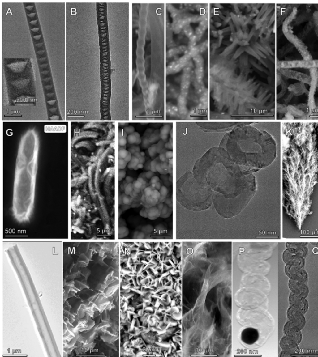
Figure S4. SEM of nanocarbon allotropes synthesized by the electrolytic splitting of \text{CO}_2 in molten carbonate. Top row (from A to F) conical CNF, nano-bamboo, nano-pearl, Ni coated CNT, nano-flower, nano-dragon. Middle row (from G to K): nano-rod, nano-belt, nano-onion, hollow nano-onion, and nano-tree. Bottom row (from L to Q) Carbon nanotube, nano-scaffold (ref. 50), nano-platelet, graphene, nanohelices. Modified from open access paper X. Liu, G. Licht, X. Wang, S. Licht, Controlled Growth of Unusual Nanocarbon Allotropes by Molten Electrolysis of \text{CO}_2 . Catalysts 12 (2022) 137. https://doi.org/10.3390/catal12020125 .
