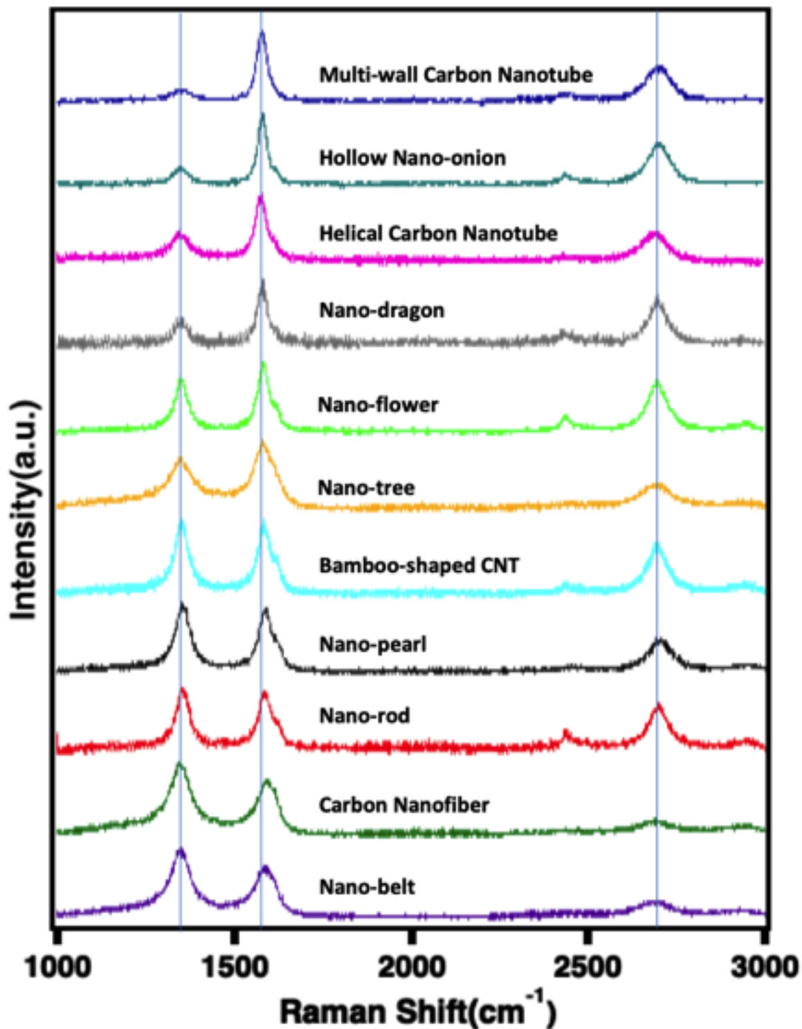
Figure S6. Raman spectra of the synthesis products consist of various labeled GNCs and packed carbon nanotube assemblies synthesized by the electrolytic splitting of CO 2 in 770°C Li 2 CO 3 with a variety of systematically varied electrochemical conditions.
