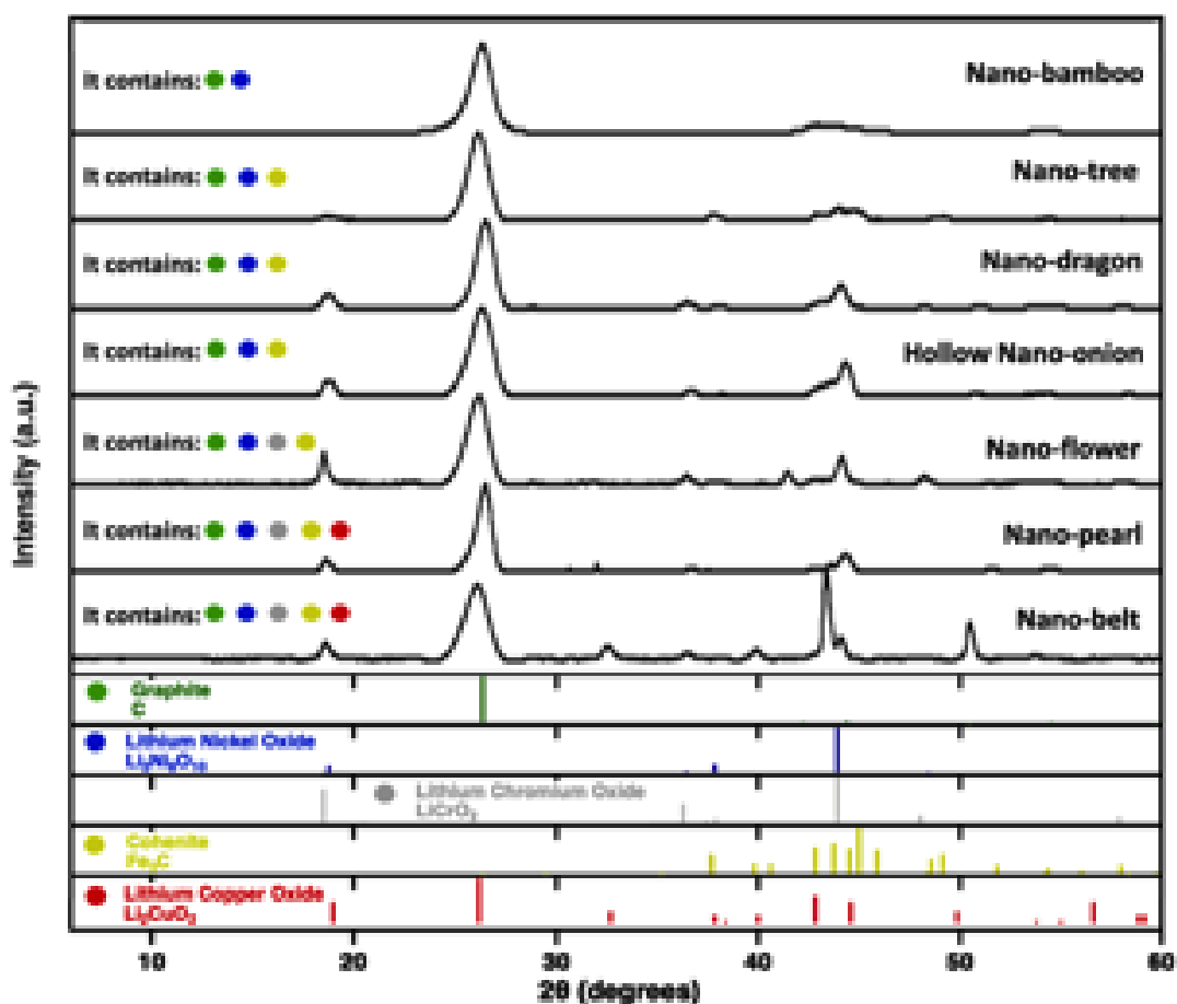
Figure S5. XRD of the synthesis product consisting of various labeled unusual nanocarbon morphologies synthesized by the electrolytic splitting of \text{CO}_2 in 770^\circ\text{C} \text{Li}_2\text{CO}_3 with a variety of systematically varied electrochemical conditions. Modified from open access paper X. Liu, G. Licht, X. Wang, S. Licht, Controlled Growth of Unusual Nanocarbon Allotropes by Molten Electrolysis of \text{CO}_2 . Catalysts 12 (2022) 137. https://doi.org/10.3390/catal12020125 .
