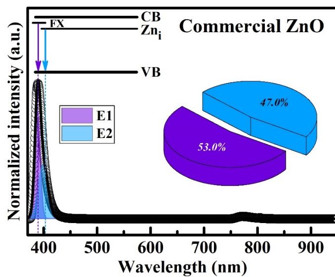
Figure S3. Photoluminescence analysis attaching with possible electronic transition diagram of commercial ZnO sample. The pie chart depicts the contribution of resolved emissions to the total spectrum.
