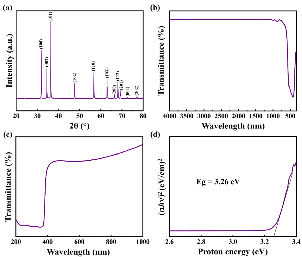
Figure S2. (a) XRD pattern, (b) The FTIR spectrum, (c) DRS and (d) Tauc plot of commercial ZnO NPs
