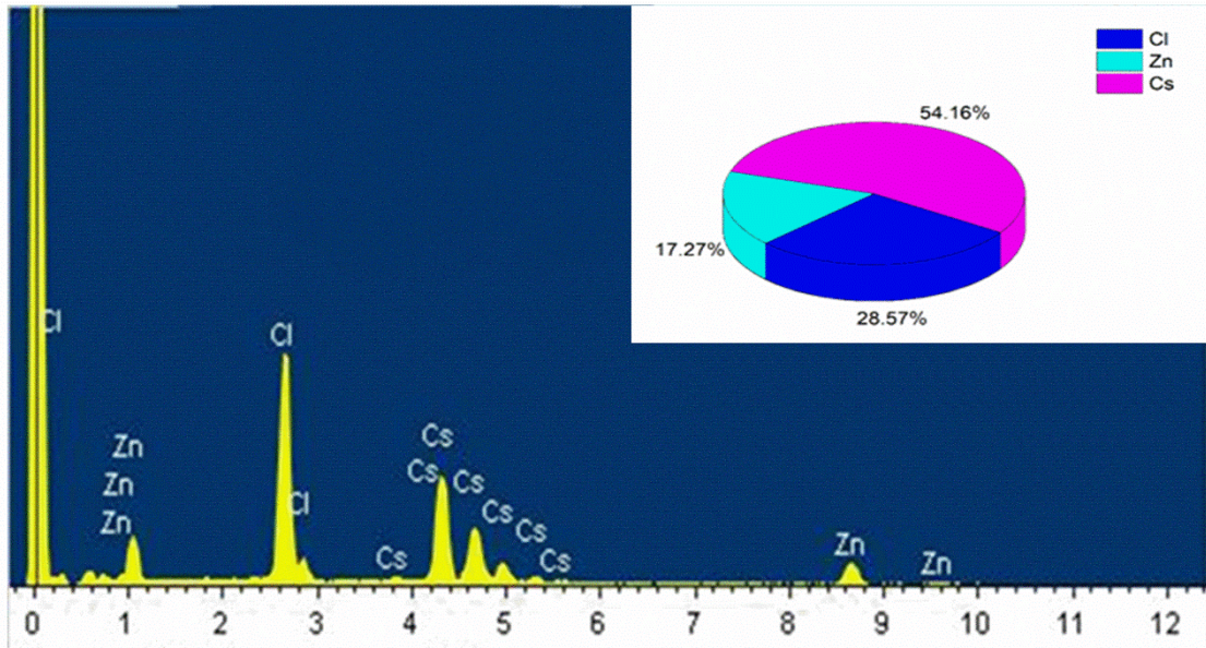
Figure S3: Elemental analysis by EDX
