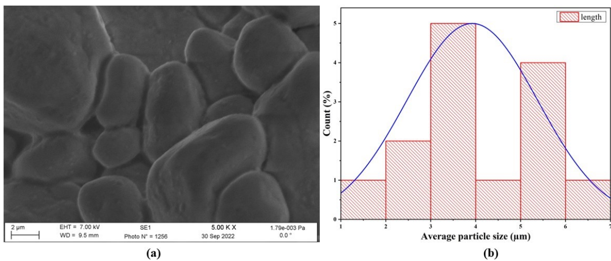
Figure S2 : a) SEM image, b) Particle size distribution of \text{Cs}_2\text{ZnCl}_4
