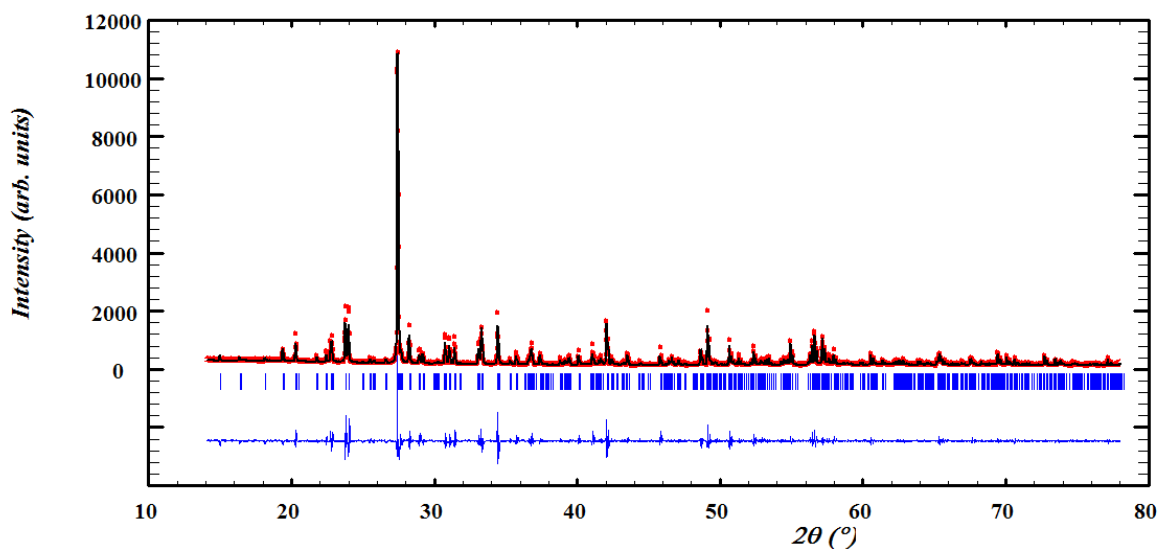
Figure S1 :XRD pattern of \text{Cs}_2\text{ZnCl}_4
