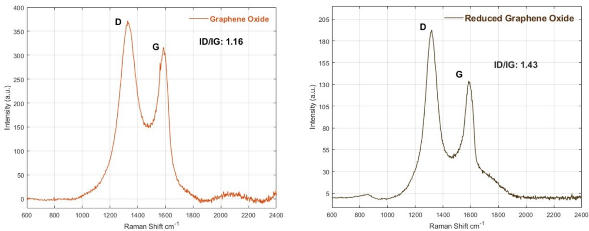
Supplementary Figure 2. Raman spectra of GO (left panel) and ERGO (right panel) electrodes. The spectral profiles and ID/IG ratios indicated a successful reduction of GO through cyclic voltammetry.
