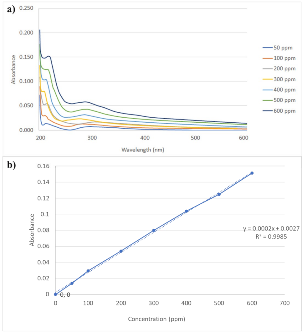
Fig. S1. a) Absorbance vs. wavelength (nm) for different oily water concentrations. b) Standard curve showing absorbance vs. concentration at 220 nm.
