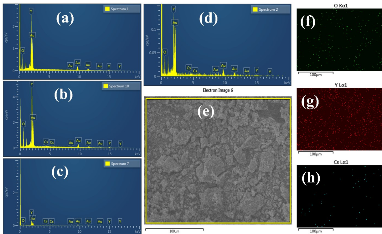
Fig. S1. EDS (a-d) and Mapping (e-h) image of Y 2 O 3 and Cs (2, 4 and 6 wt.%) doped Y 2 O 3 NSs
