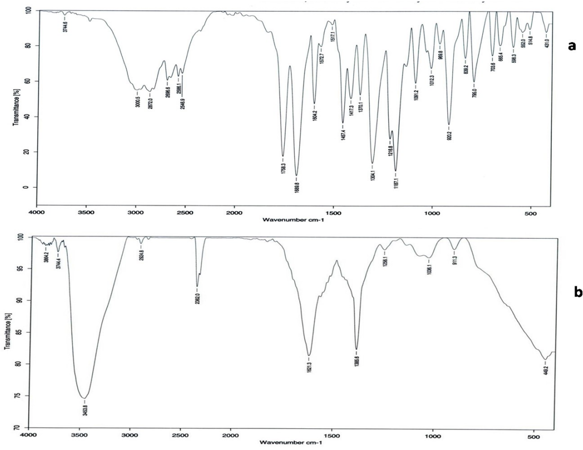
S2: FT-IR spectra of (A) Aspirin (B) Aspirin capped TNPs
