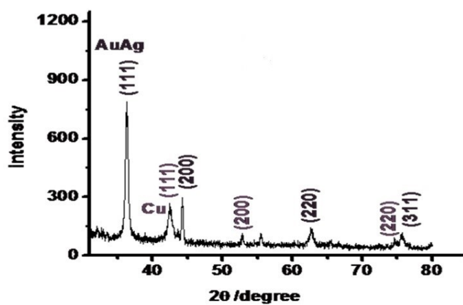
S1: XRD analysis of trimetallic nanoparticles
