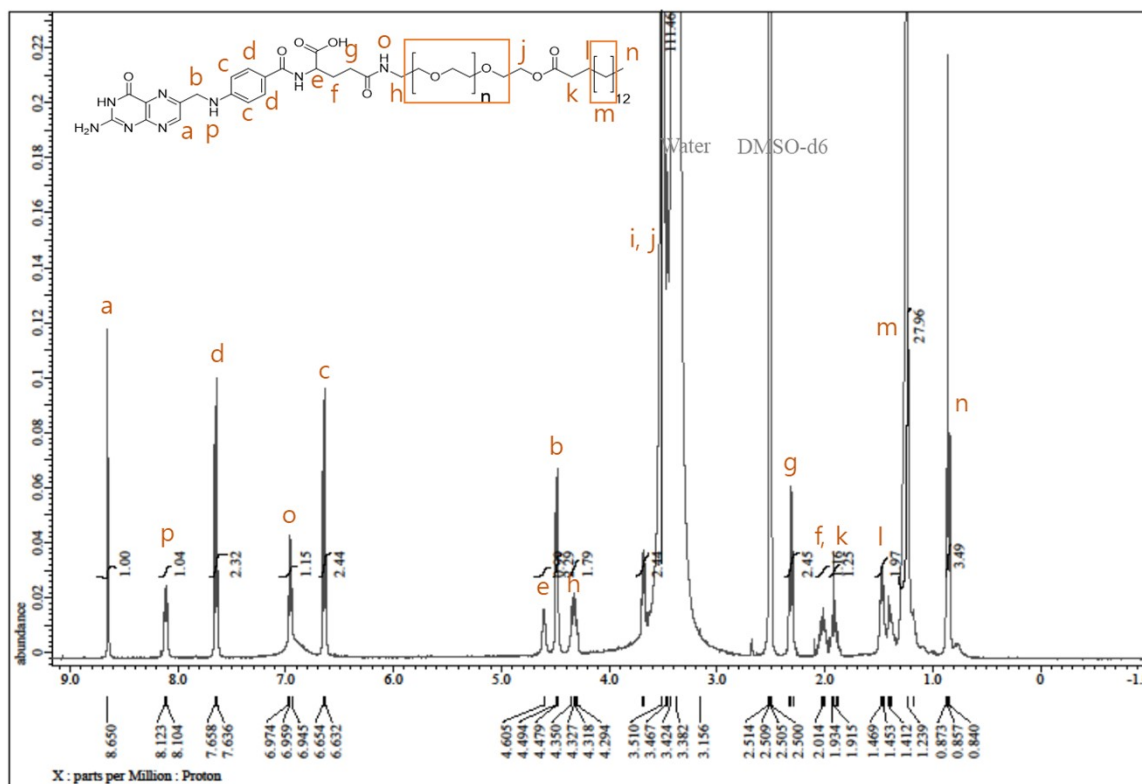
Figure S5. 1 H NMR spectral data of PPFA
