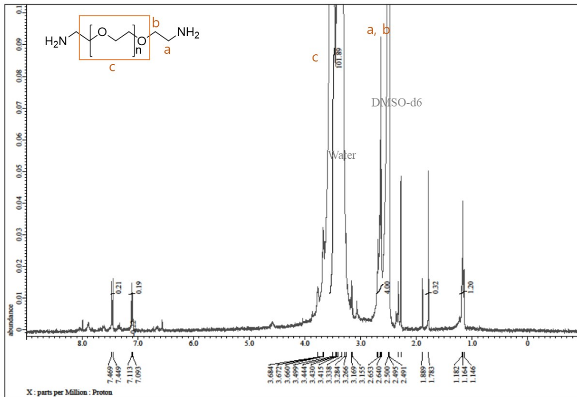
Figure S2. 1 H NMR spectral data of polyethylene glycol
