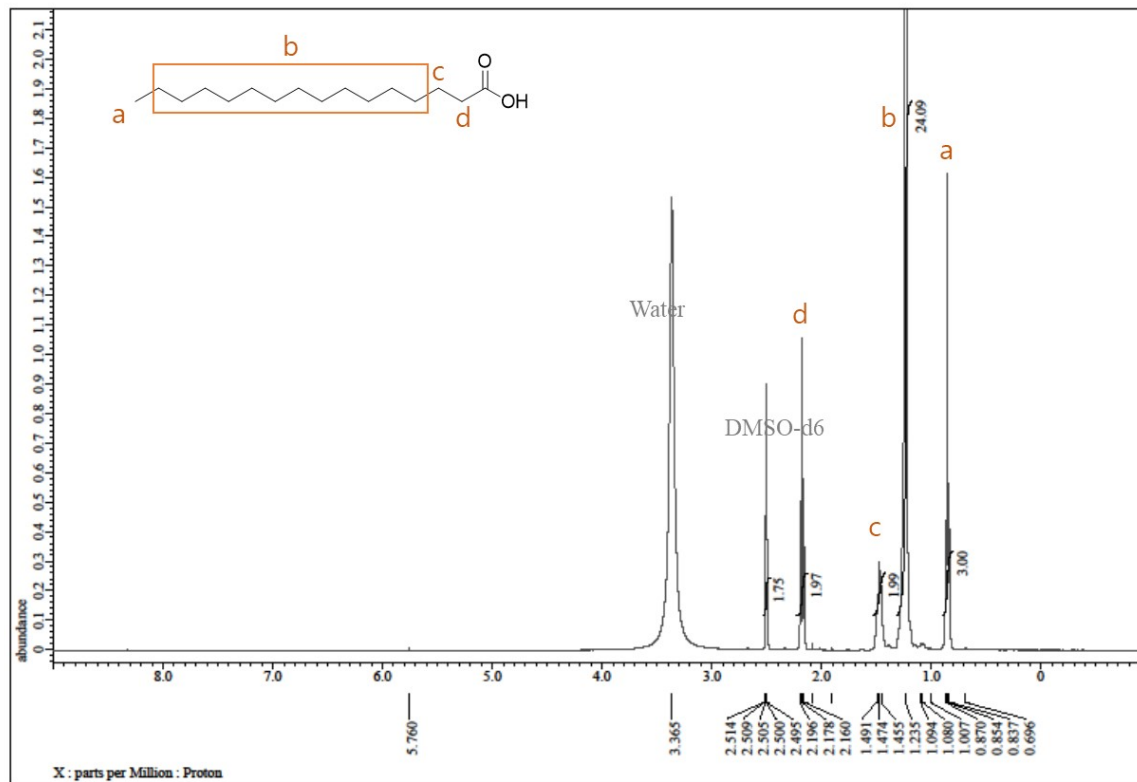
Figure S1. 1 H NMR spectral data of palmitic acid
