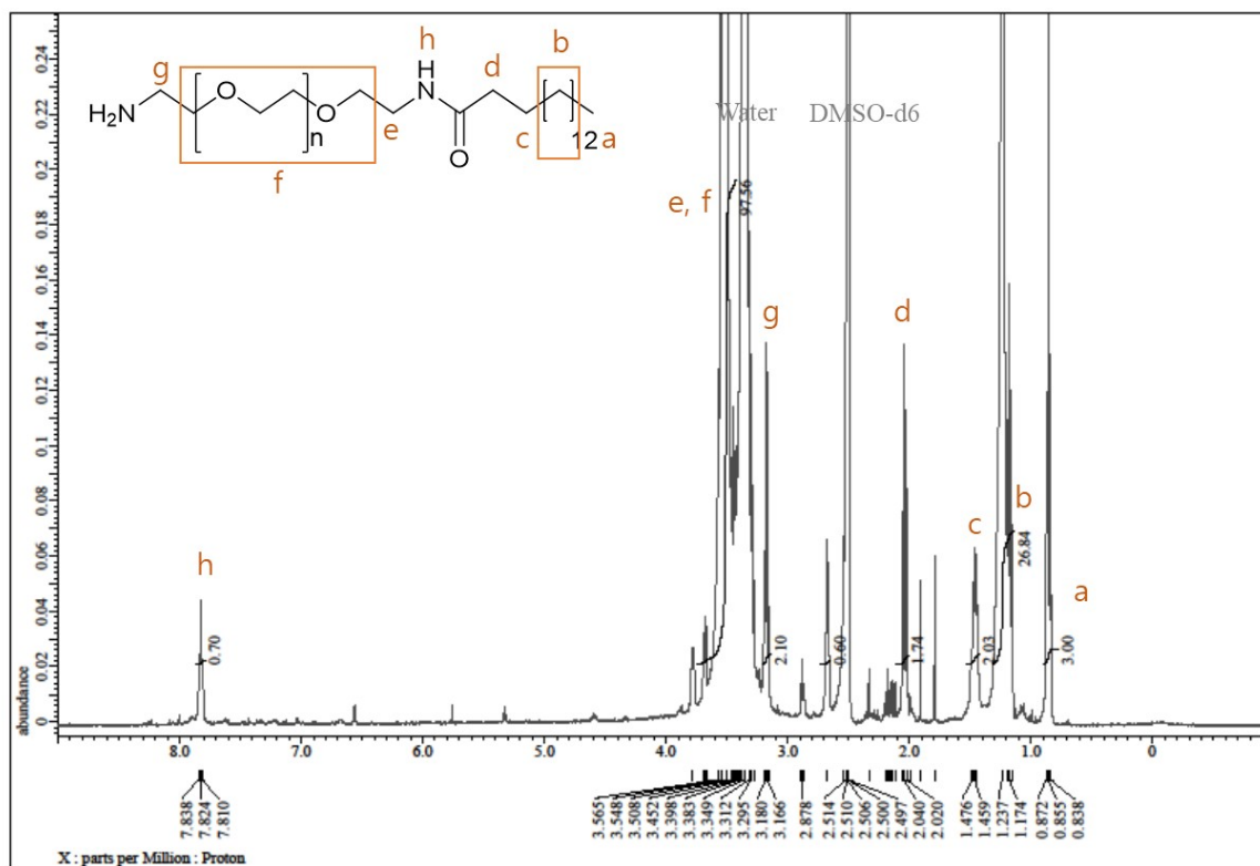
Figure S3. 1 H NMR spectral data of PP
