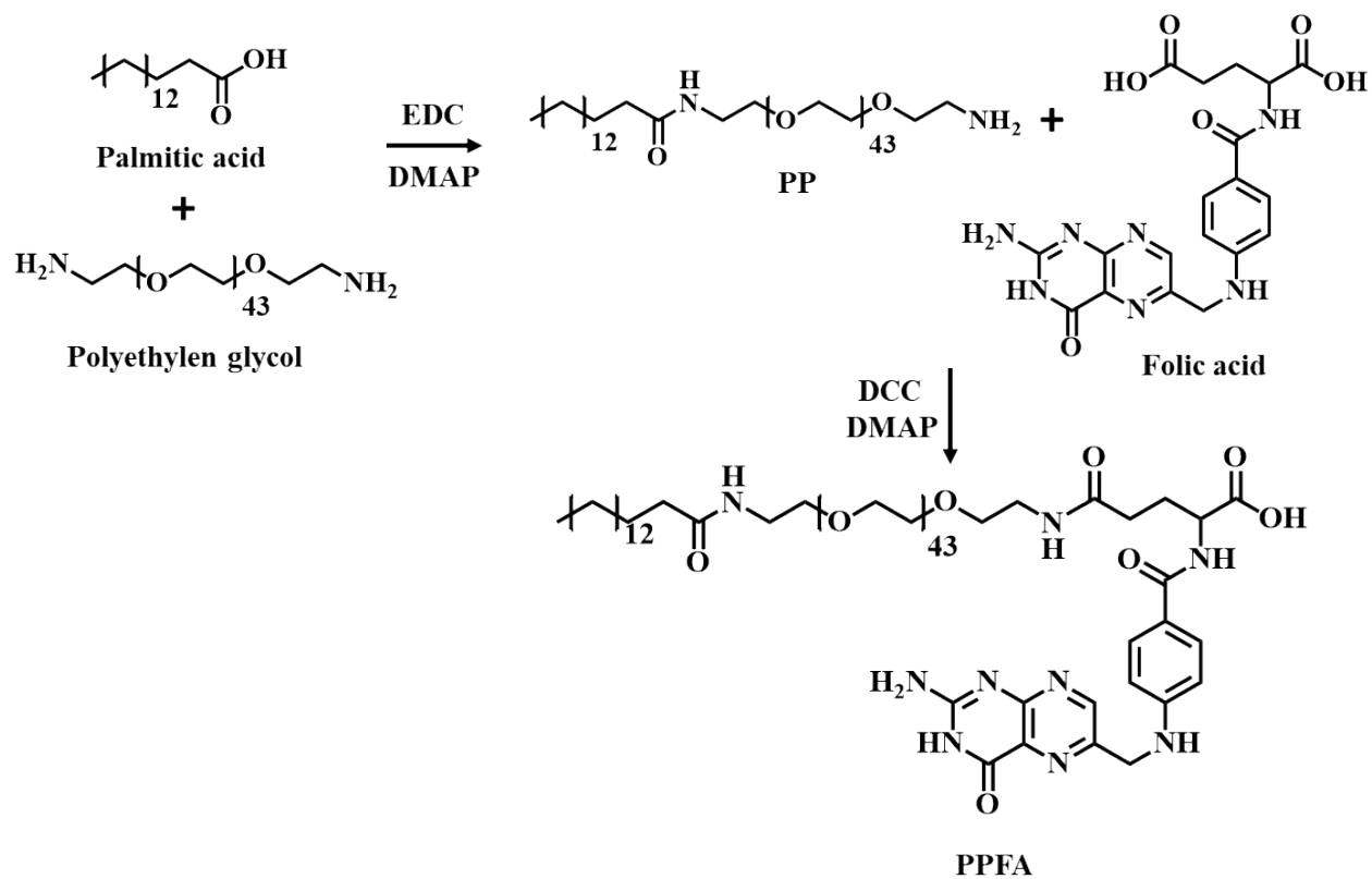
Scheme S1. Synthesis scheme of PPFA.
