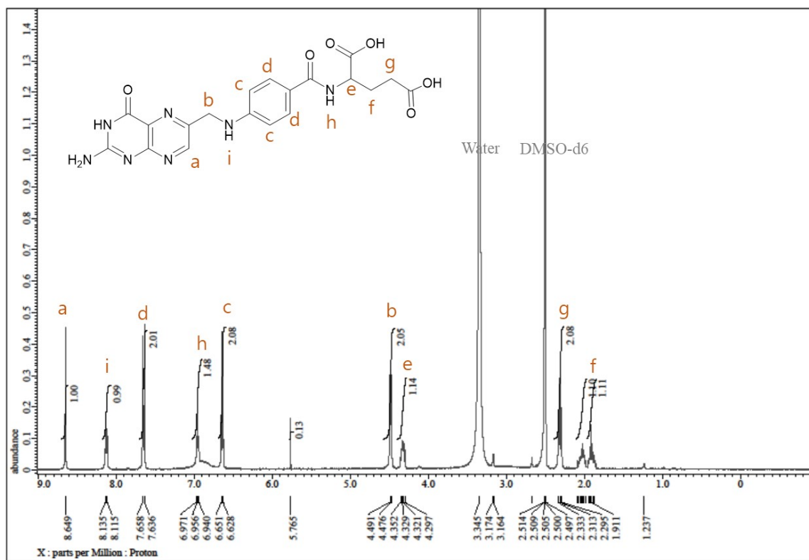
Figure S4. 1 H NMR spectral data of folic acid
