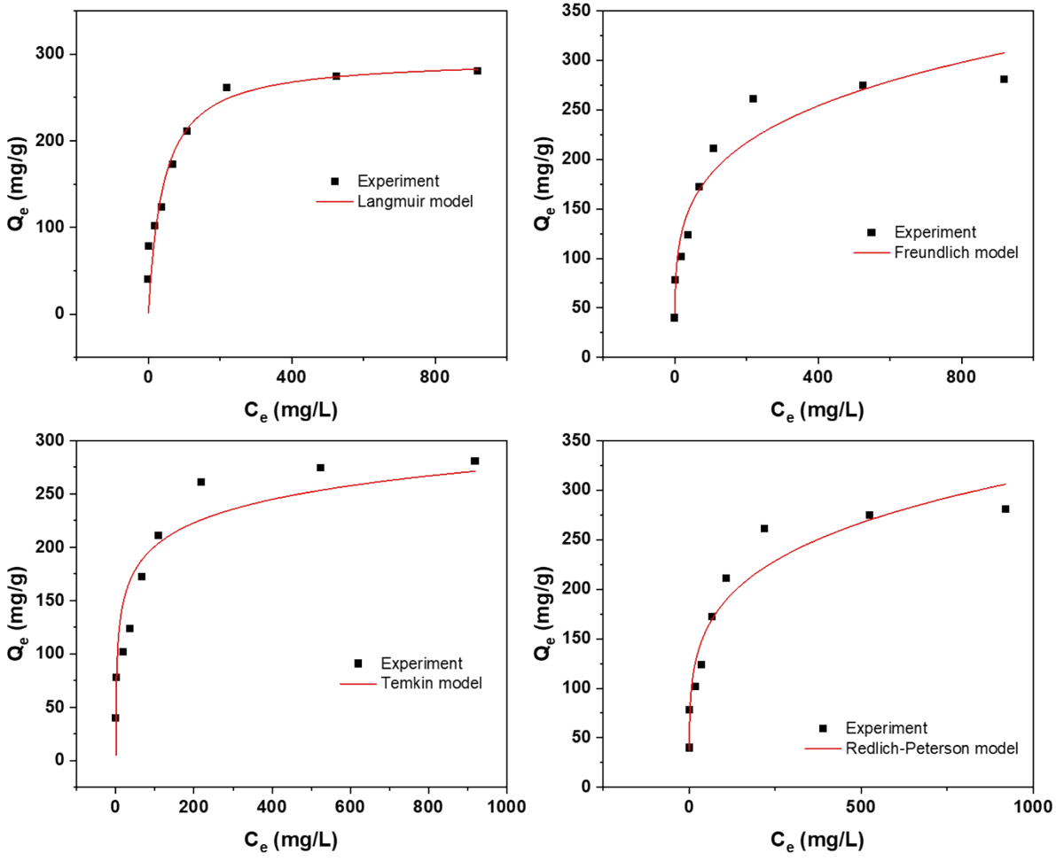
Figure S1: Isotherms for H_2SO_4 activation at 318K
