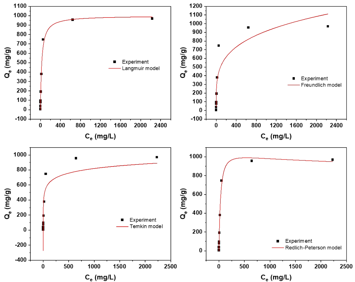
Figure S4: Isotherms for NaOH activation at 338K
