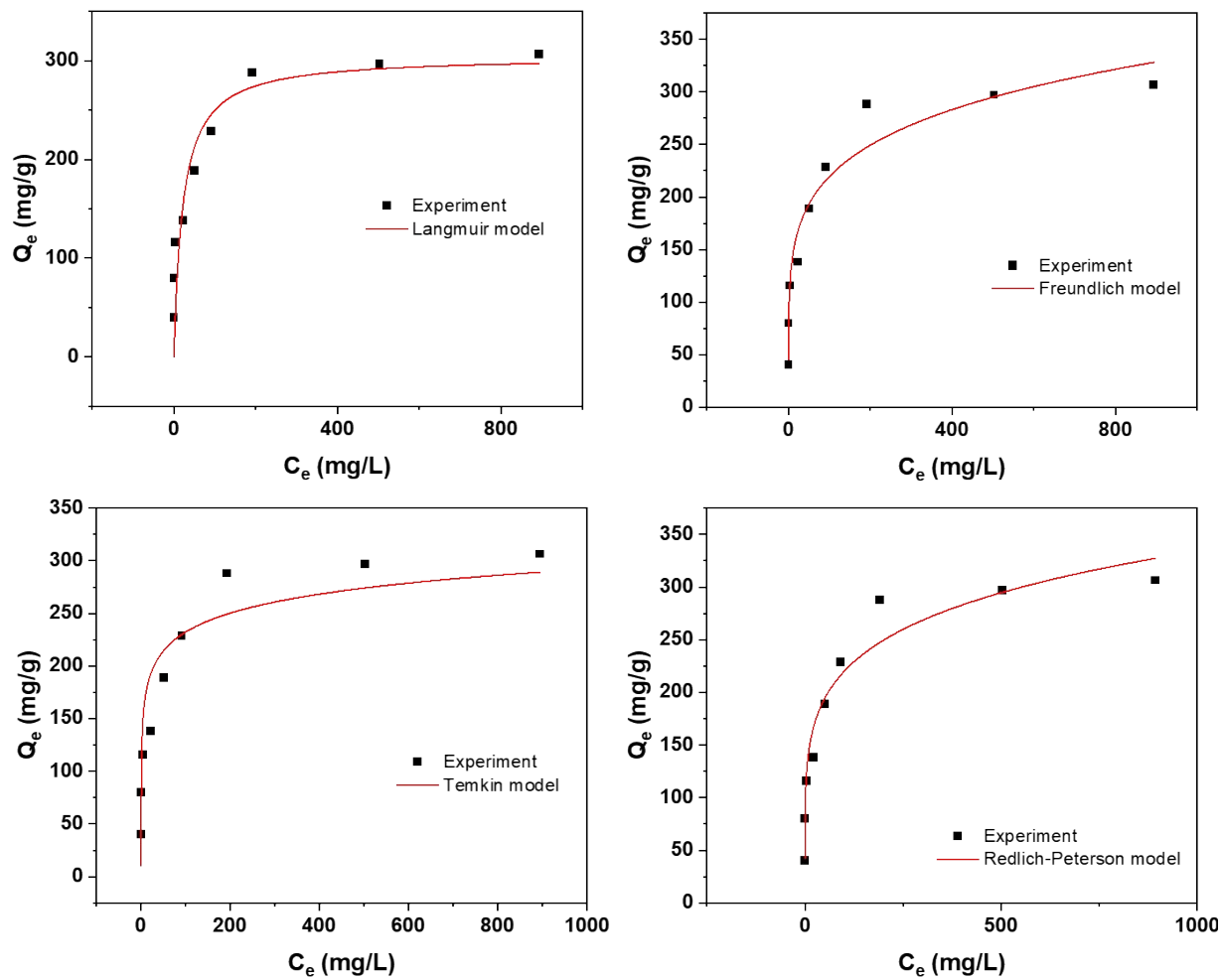
Figure S2: Isotherms for H_2SO_4 activation at 338K
