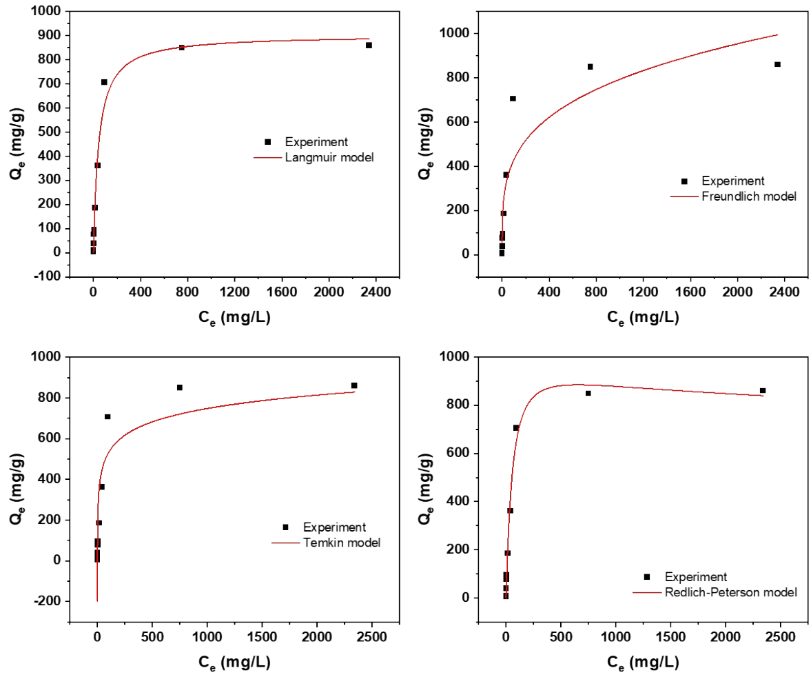
Figure S3: Isotherms for NaOH activation at 318K
