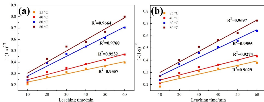
Fig. S1. Plots of 1-(1-x)^{1/3} vs. time at various temperatures for (a) Tb, and (b)
