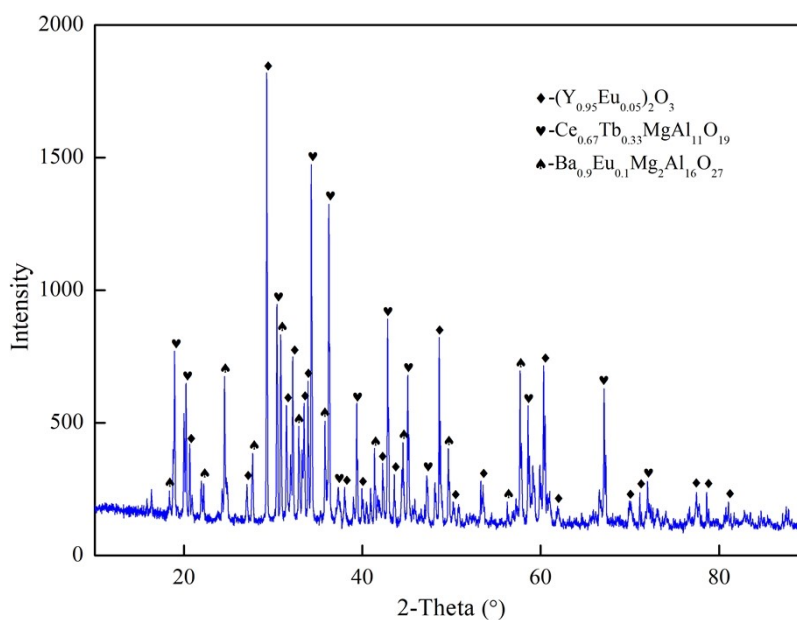
Fig. S2. XRD pattern of the original phosphors.
