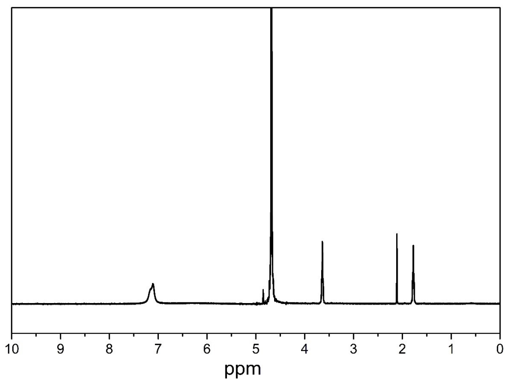
Figure S3: NMR spectra of [\text{Co}(\text{NTB})\text{Cl}]\text{Cl} in water
