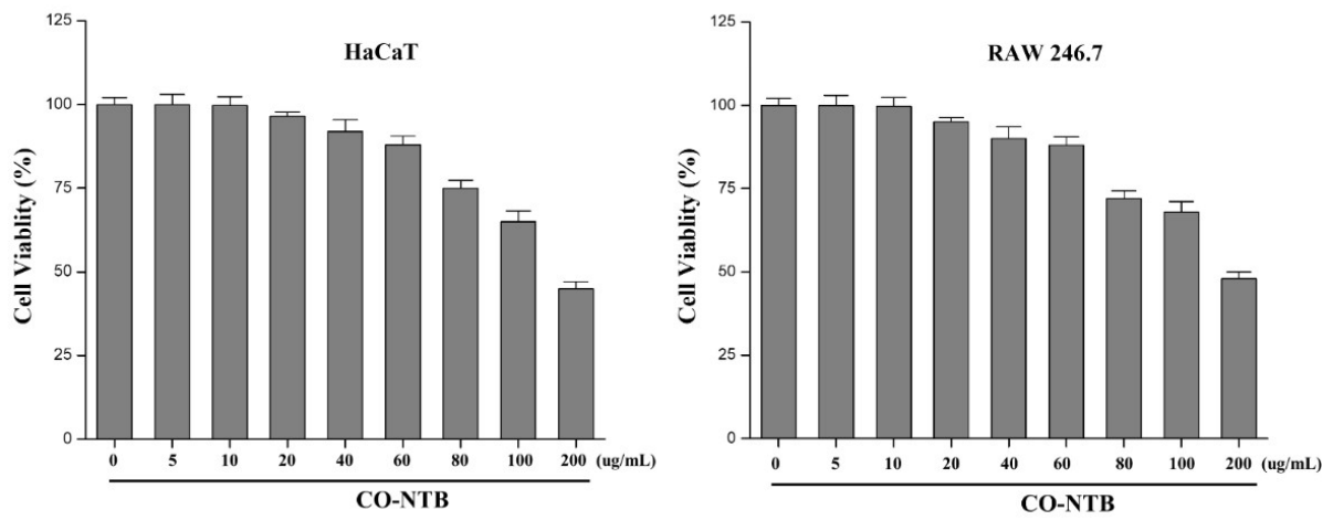
Figure S4: Toxicity assessment of Co-NTB in human keratinocyte cell line (HaCaT) and murine mouse macrophage (RAW 246.7)
