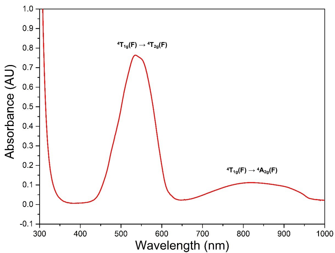
Figure S1: UV-Visible spectra of [Co(NTB)Cl]Cl in water (0.3mM)
