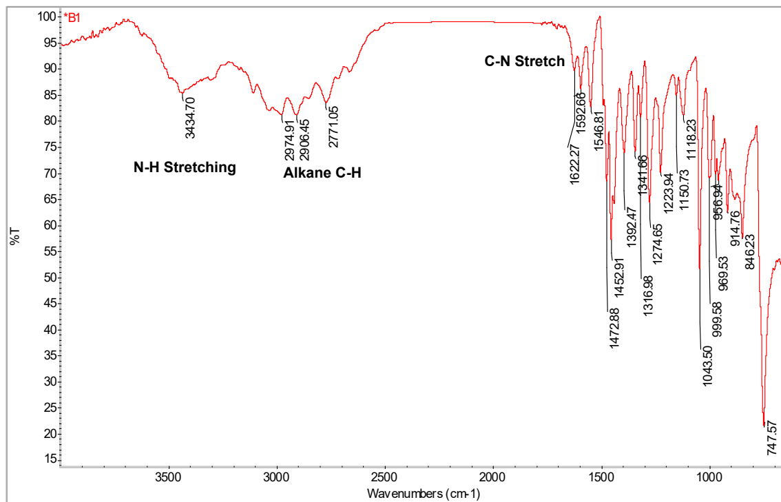
Figure S2: IR spectra of [Co(NTB)Cl]Cl
