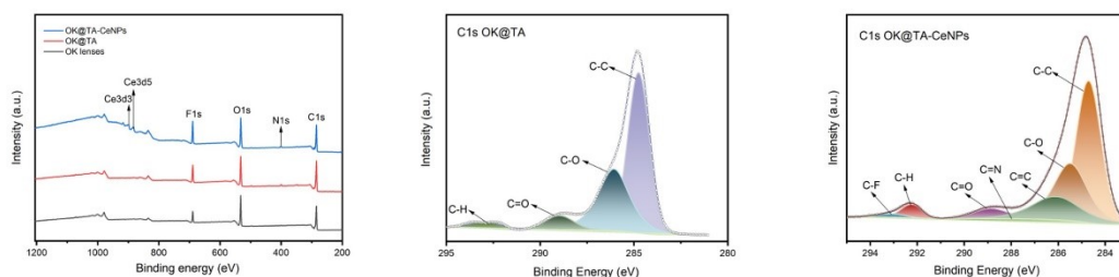
Figure S3. XPS analysis of OK, OK@TA, and OK@TA-CeNPs
