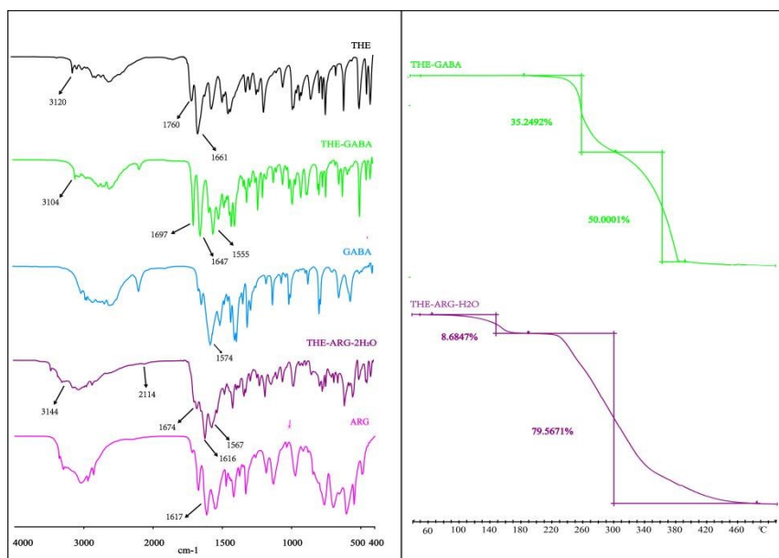
Figure S3. IR (left) and TGA (right) profiles of API, CCFs, and the corresponding cocrystals.
