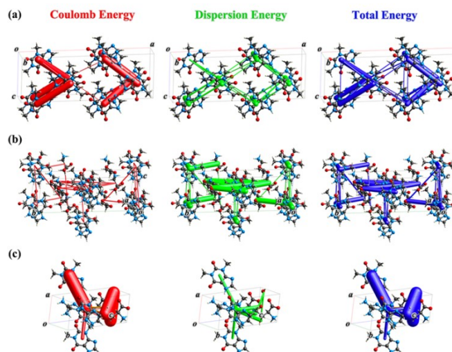
Figure S5. Energy frameworks of THE (a), THE-GABA (b), and THE-ARG-2H 2 O (c).
