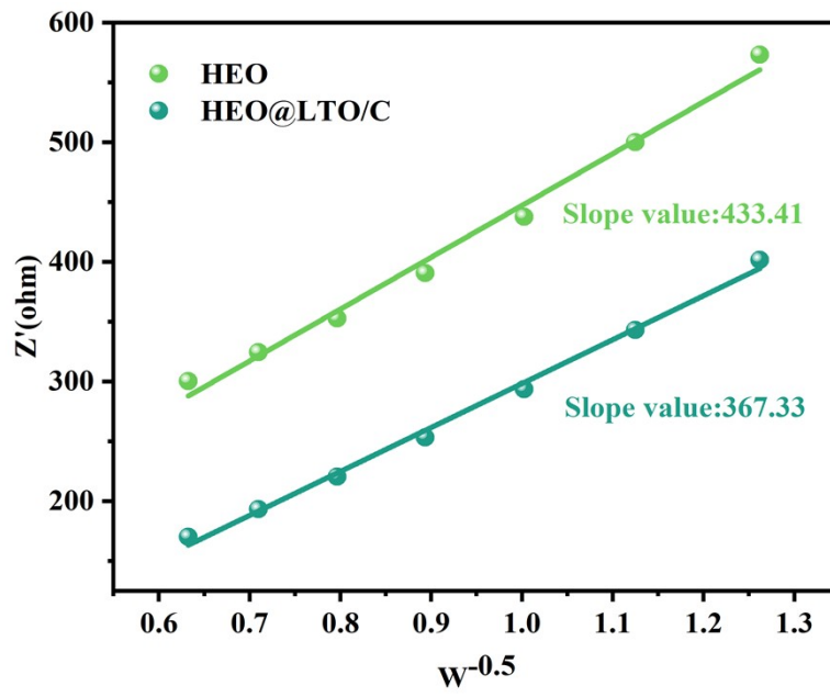
Fig. S1 plots of Z' versus \omega^{-0.5} from EIS data
