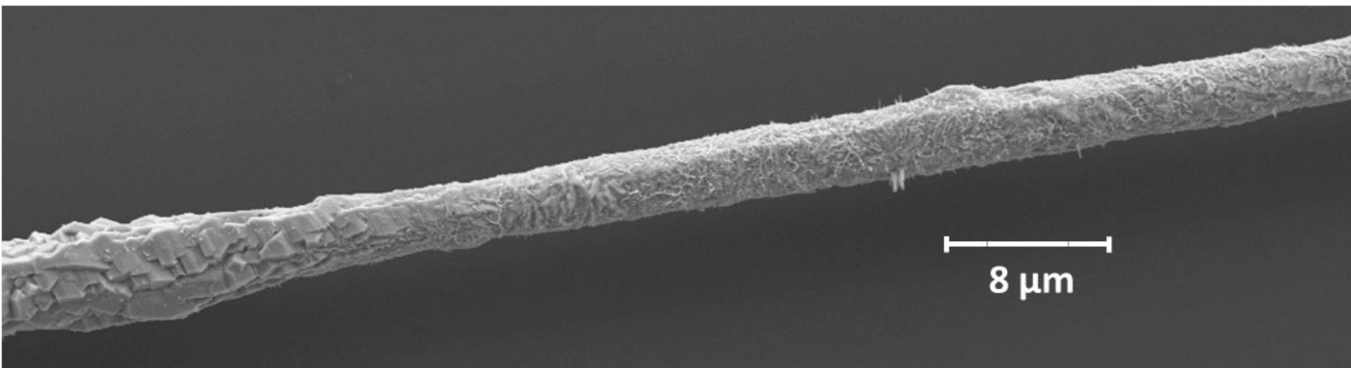
SEM image showing that the diameter of the ZnO:Sb microwires varies from one place to another and shows the wire to be polycrystalline with a rough surface.
