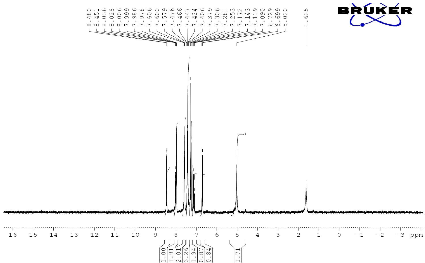
1 H-NMR spectrum of HSB-6
