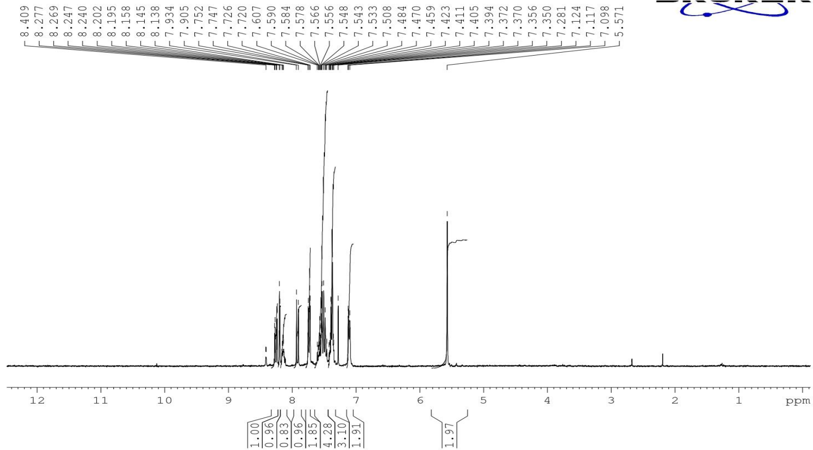
1 H-NMR spectrum of HSB-5
