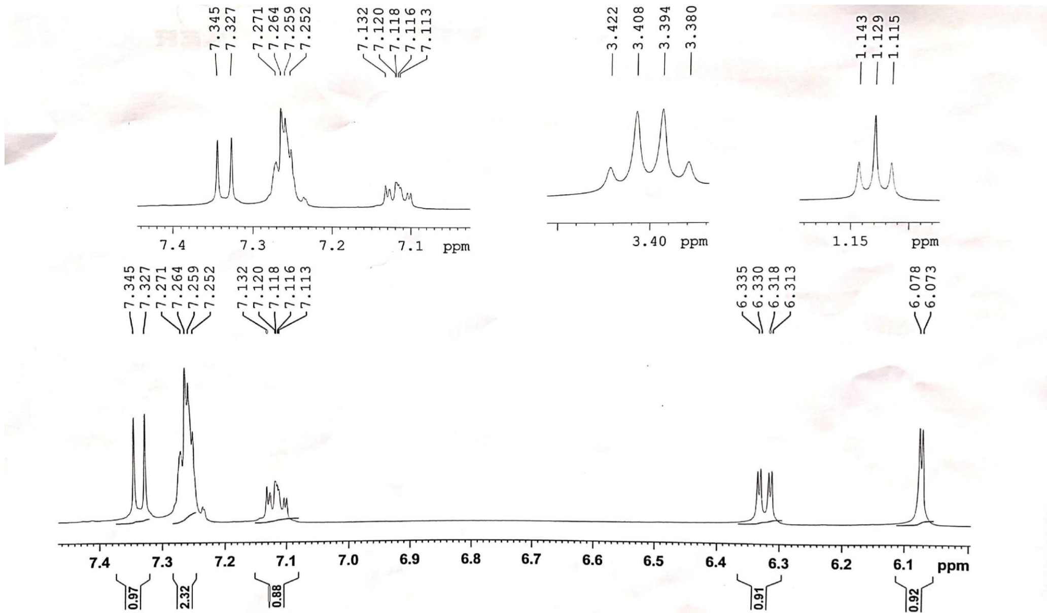
^1\text{H-NMR} expanded spectrum of HSB-3
