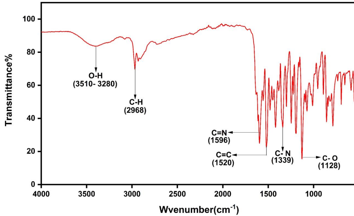
Fourier Transform Infrared (FTIR) spectrum of HSB-2
