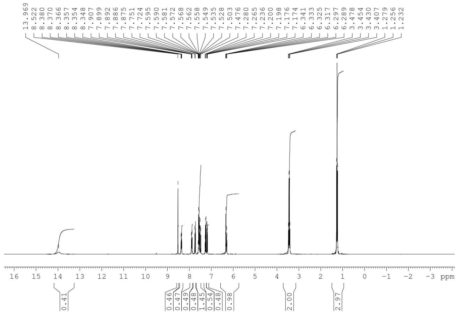
1 H-NMR spectrum of HSB-4
