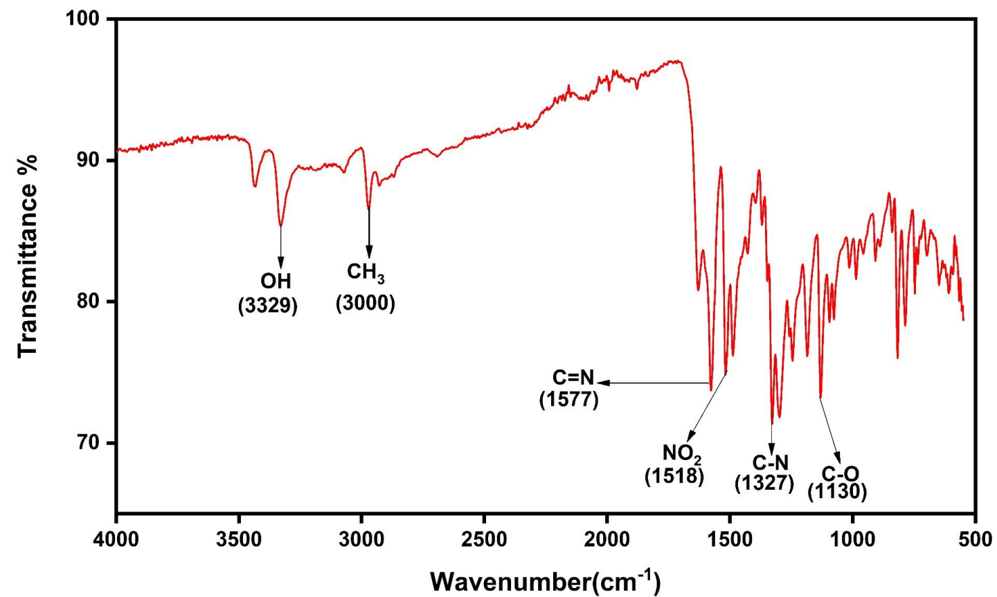
Fourier Transform Infrared (FTIR) spectrum of HSB-1
