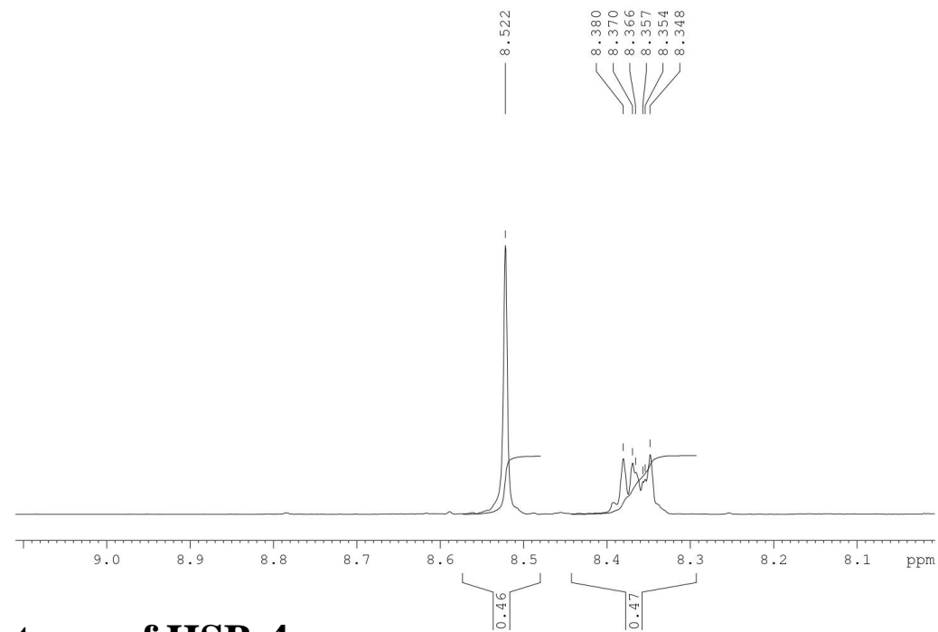
1 H-NMR expanded spectrum of HSB-4
