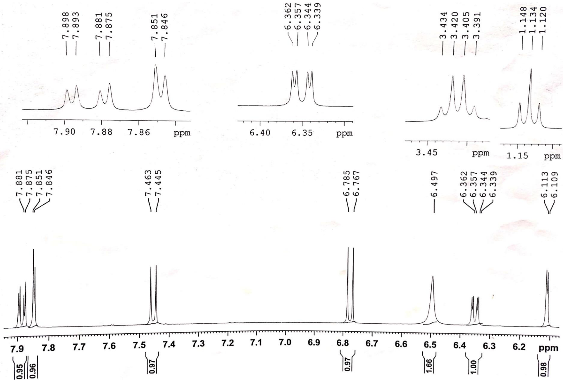
^1\text{H-NMR} expanded spectrum of HSB-1
