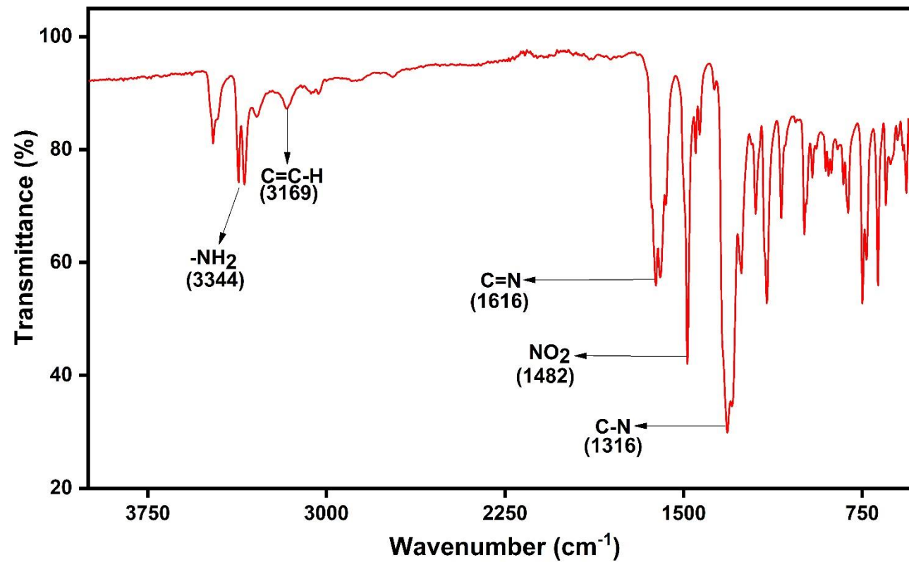
Fourier Transform Infrared (FTIR) spectrum of HSB-6
