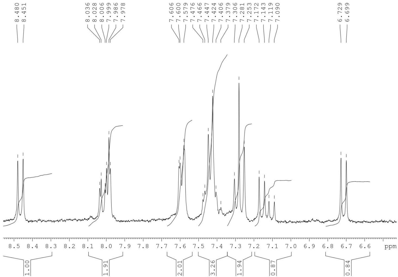
^1\text{H-NMR} expanded spectrum of HSB-6
