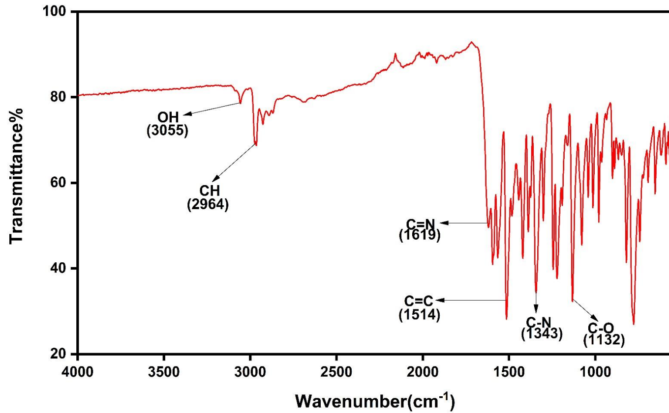
Fourier Transform Infrared (FTIR) spectrum of HSB-4
