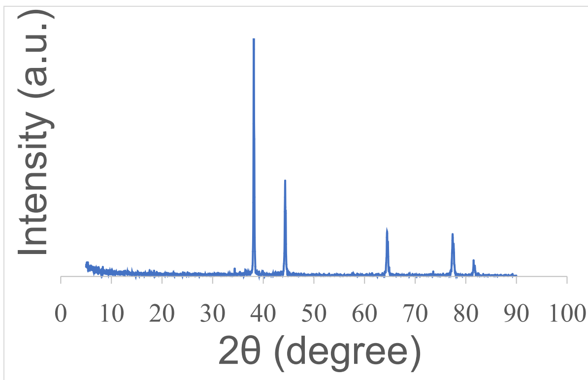
Fig. S1. The XRD pattern of the Free Ag NPs.
