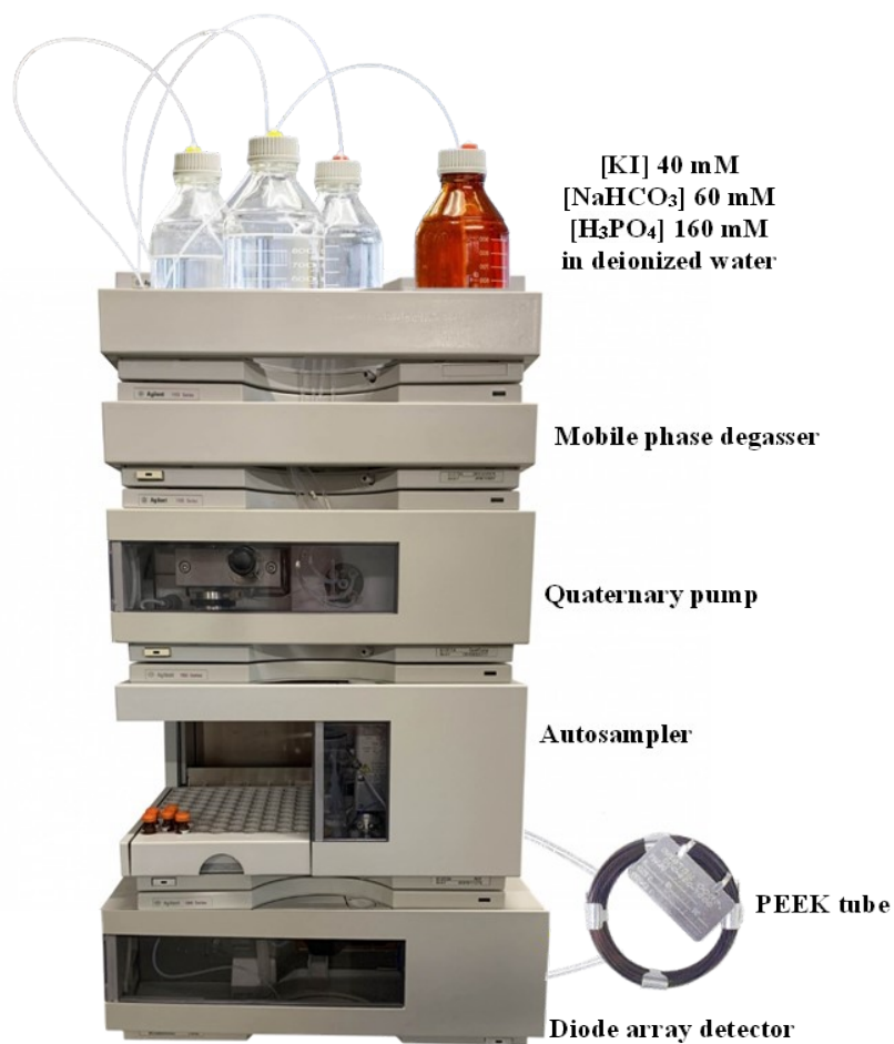
Fig. 1S. Modified HPLC setup for SPC quantification
