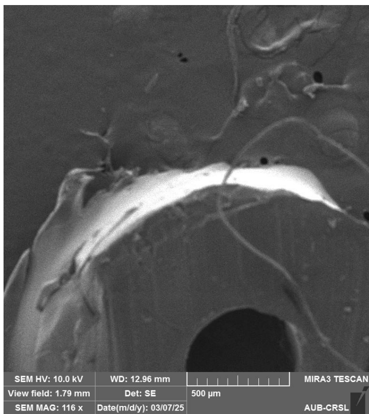
Fig. 5S. SEM image showing internal diameter of the used PEEK tube after more than 3000 samples.
