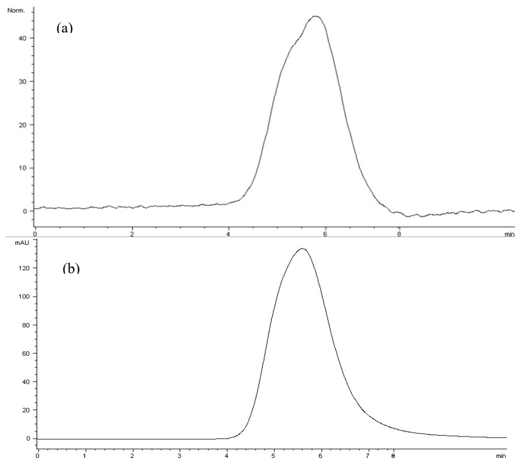
Fig. 3S. Chromatograms showing the peak of SPC in (a) Vanish detergent sample and (b) SPC standards
