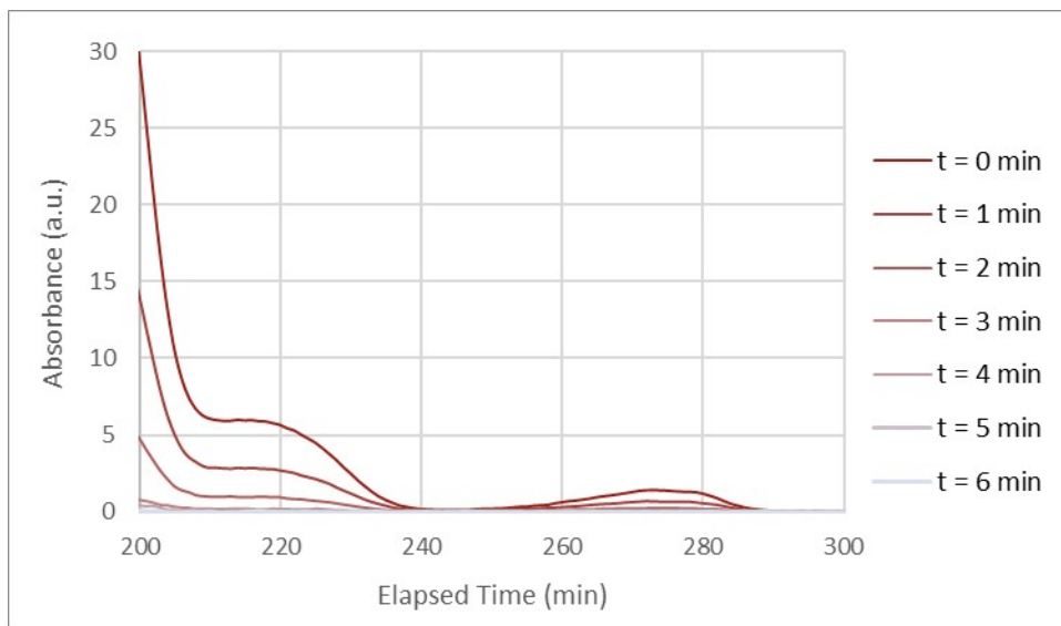
Fig. 4S. UV Spectra of Tramadol showing its degradation during AOP experiment
