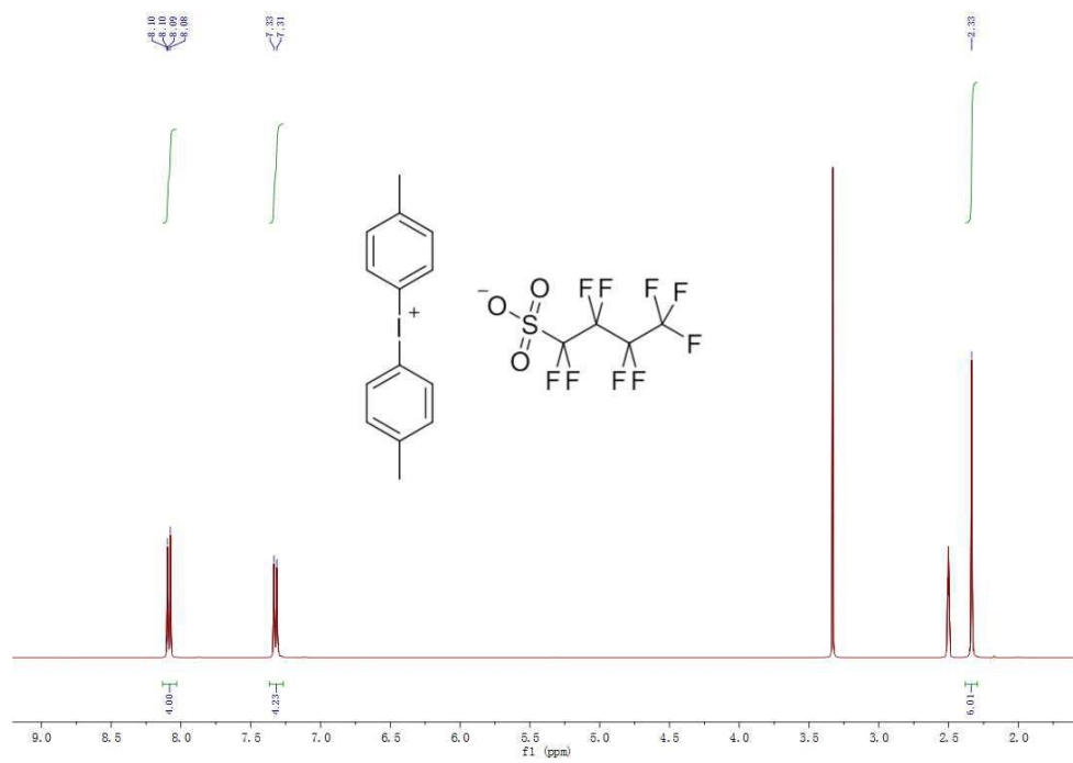
1 H NMR spectra of PAG2-3b
