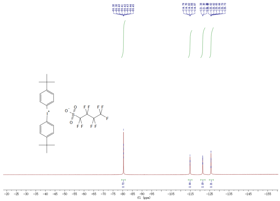
19 F NMR spectra of PAG3-3b
