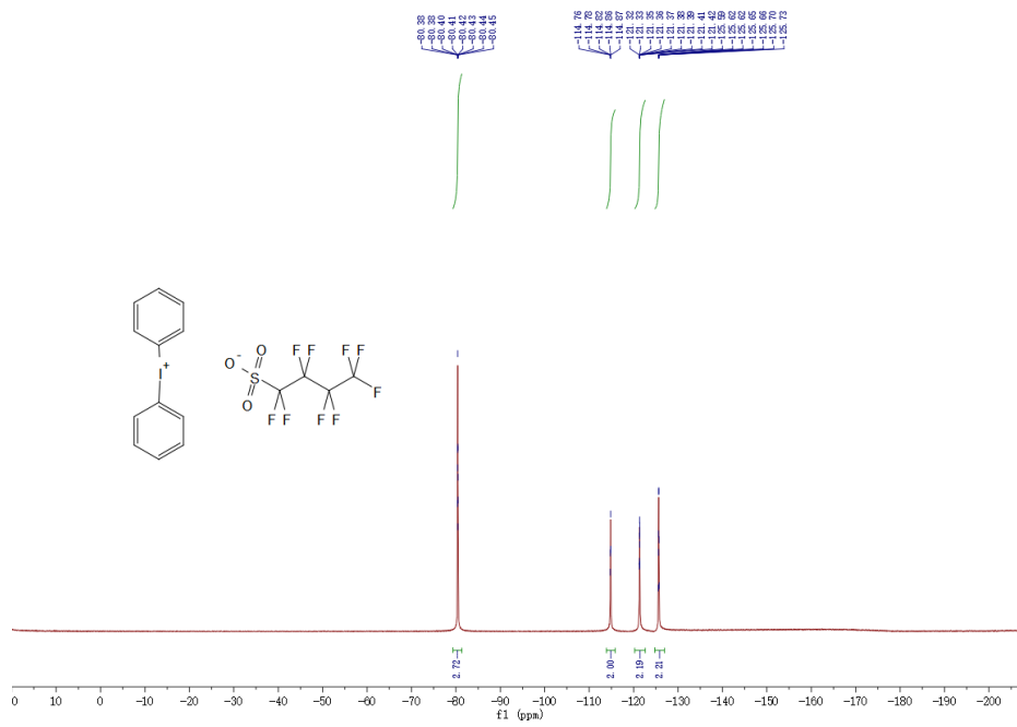
19 F NMR spectra of PAG1-3b
