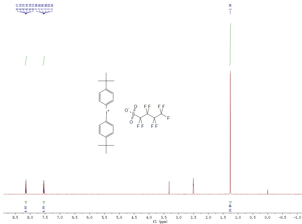
1 H NMR spectra of PAG3-3b
