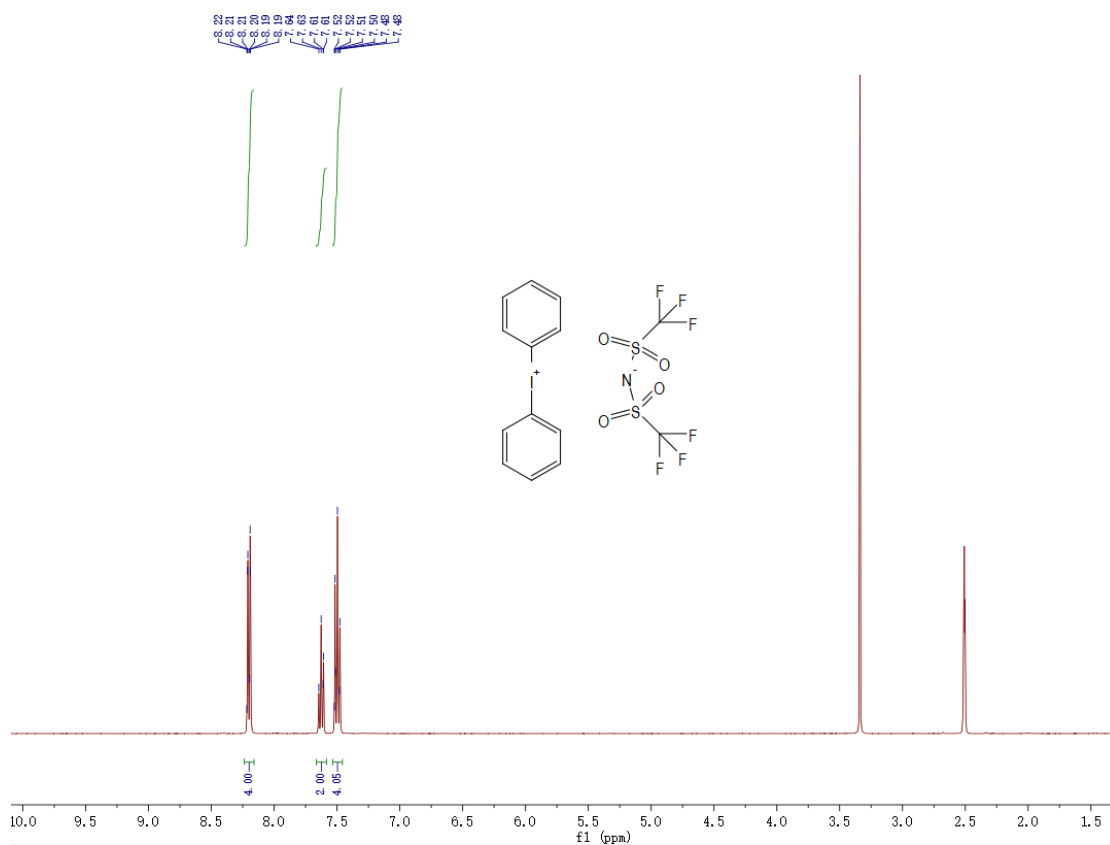
1 H NMR spectra of PAG1-3a
