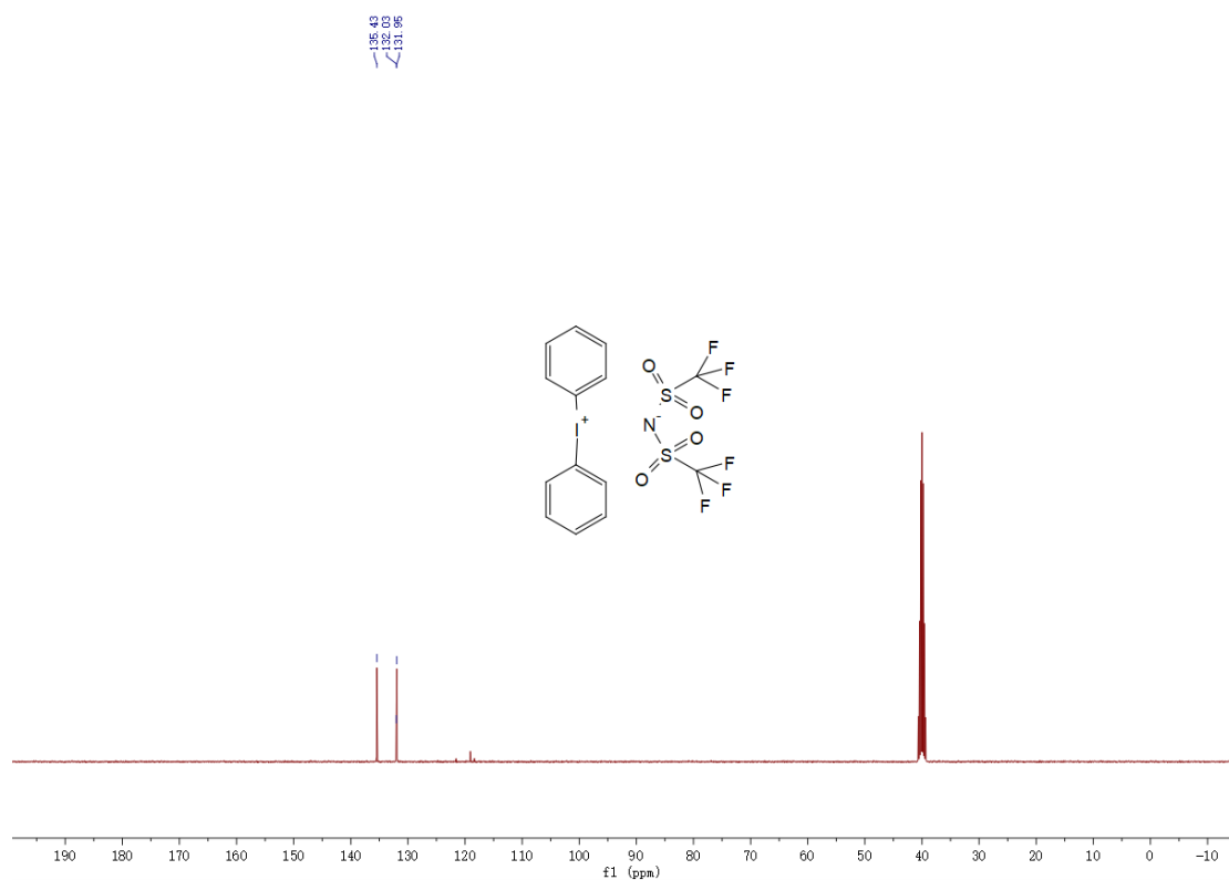
13 C NMR spectra of PAG1-3a
