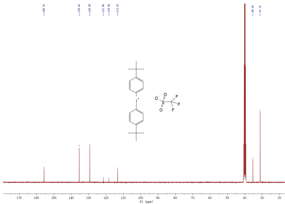
13 C NMR spectra of PAG3-3c
