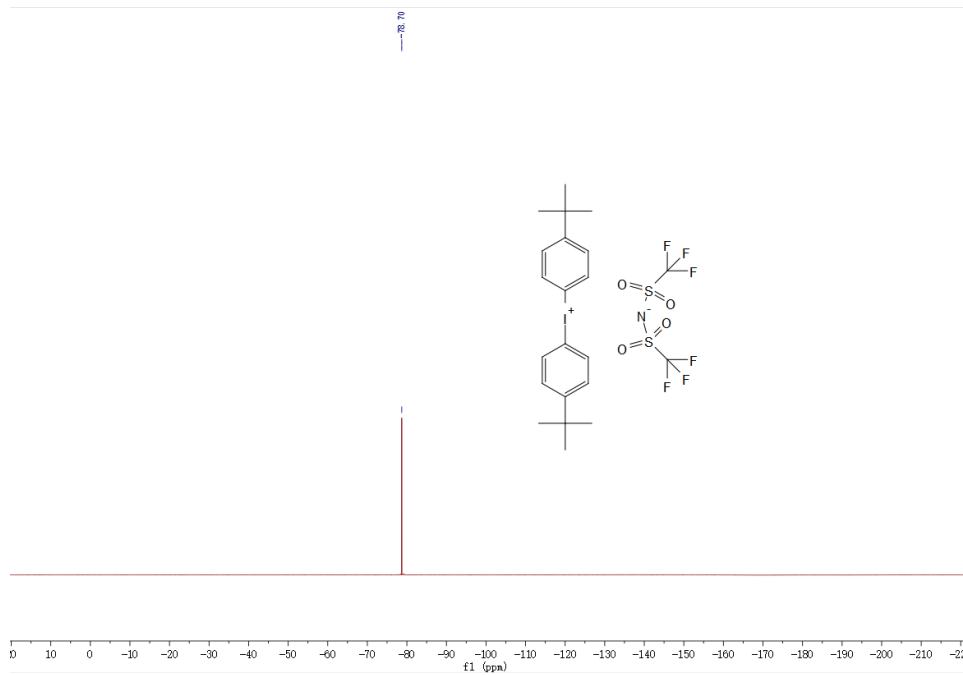
19 F NMR spectra of PAG3-3a
