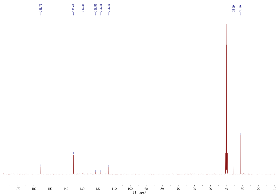
^{13}\text{C} NMR spectra of PAG3-3a
