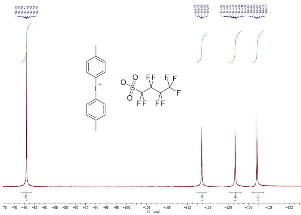
19 F NMR spectra of PAG2-3b
