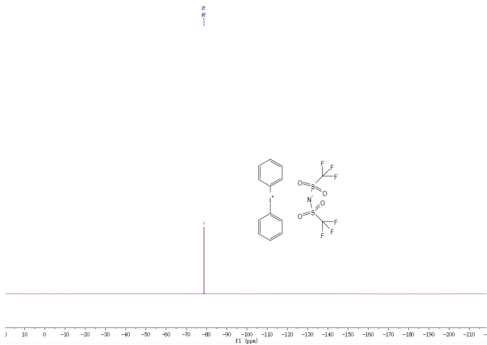
19 F NMR spectra of PAG1-3a
