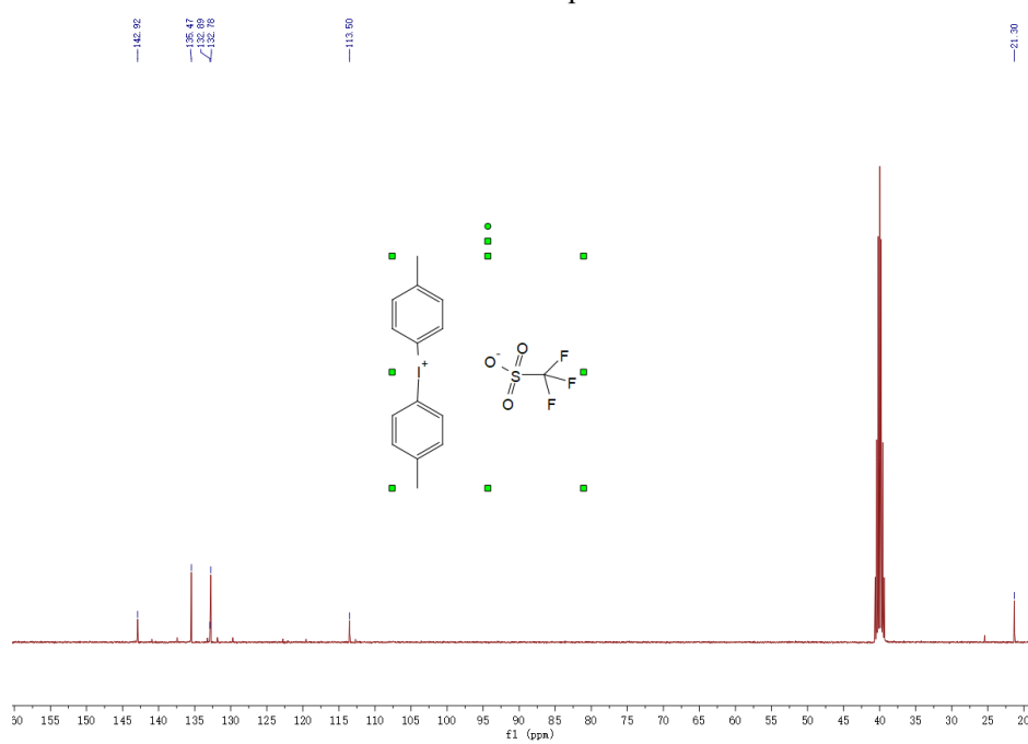
13 C NMR spectra of PAG2-3c
