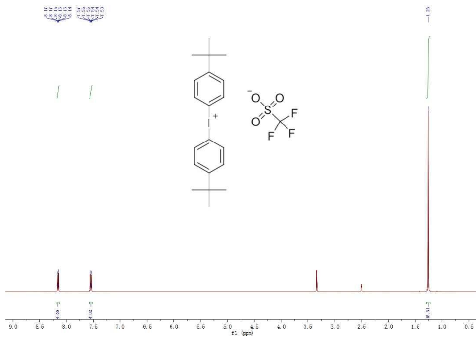
^1\text{H} NMR spectra of PAG3-3c
