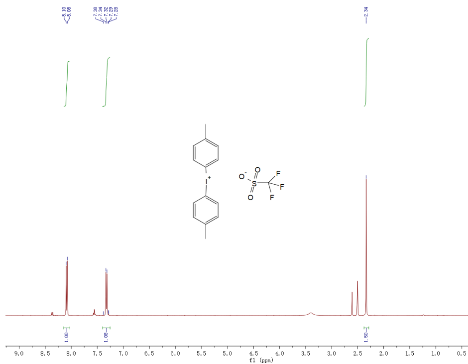
1 H NMR spectra of PAG2-3c
