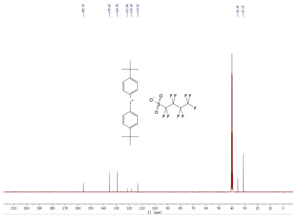
13 C NMR spectra of PAG3-3b
