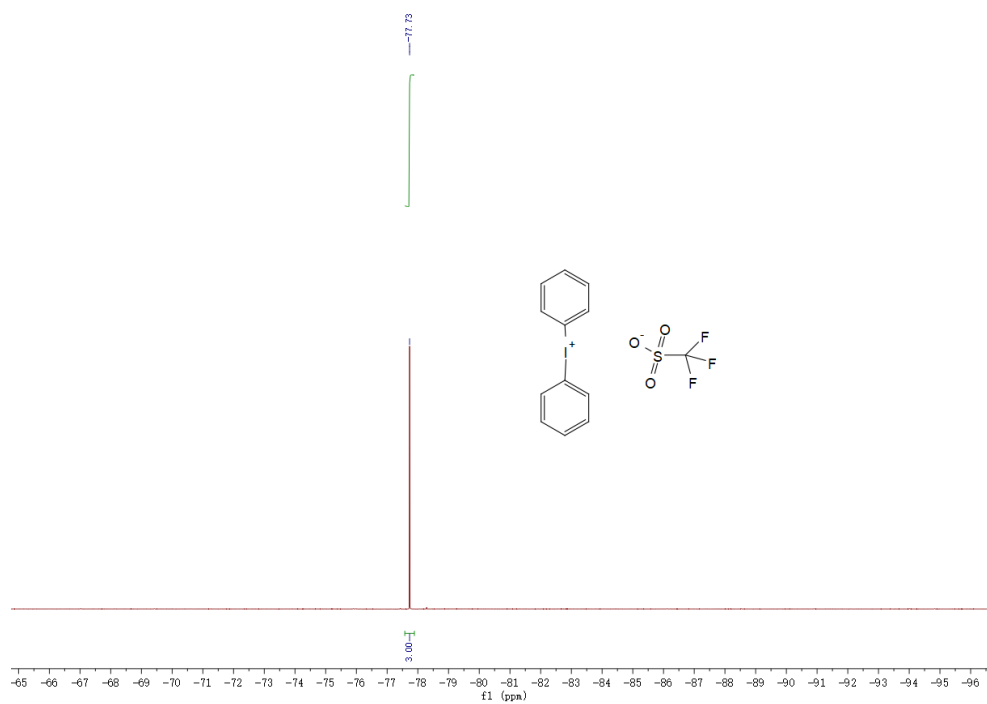
19 F NMR spectra of PAG1-3c
