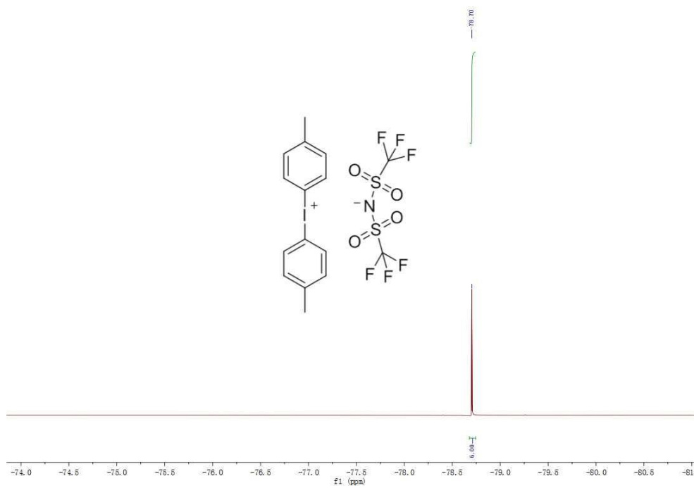
19 F NMR spectra of PAG2-3a
