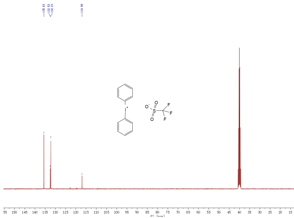
13 C NMR spectra of PAG1-3c
