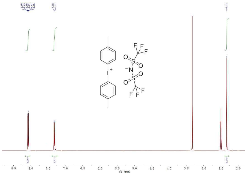
1 H NMR spectra of PAG2-3a
