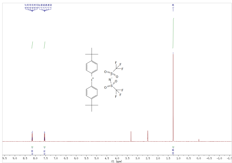
^1\text{H} NMR spectra of PAG3-3a
