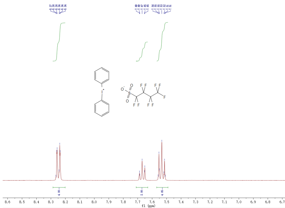
1 H NMR spectra of PAG1-3b
