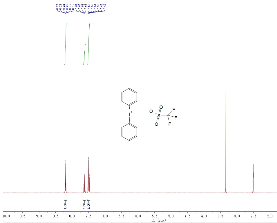
1 H NMR spectra of PAG1-3c
