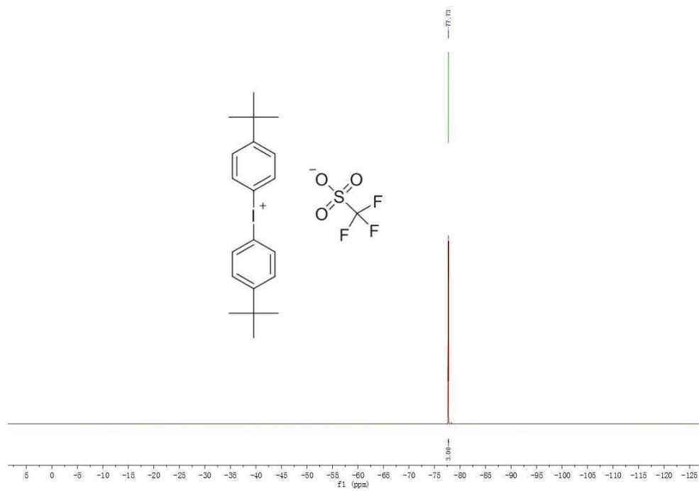
19 F NMR spectra of PAG3-3c
