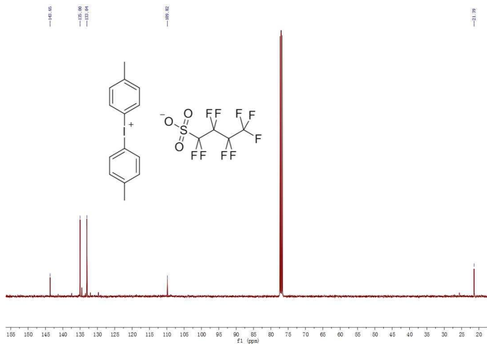
13 C NMR spectra of PAG2-3b
