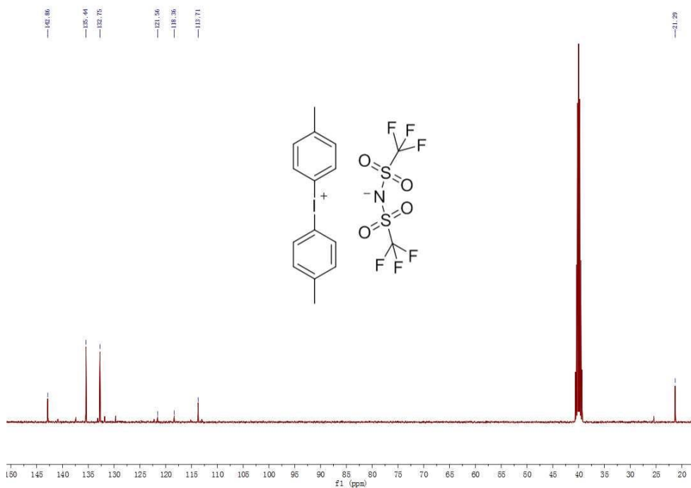
13 C NMR spectra of PAG2-3a
