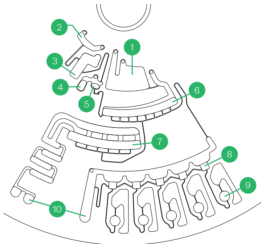
1R clinical chemistry disc schematic. Annotated structures: (1) Dilution buffer inlet chamber; (2) sample inlet chamber; (3) sample plasma separation chamber; (4) sample overflow chamber; (5) sample metering chamber; (6) dilution mixing chamber; (7) dilution ballast chamber; (8) diluted sample aliquot chamber; (9) reaction chamber (contains 1R reagent lysosphere); (10) overflow chambers.
