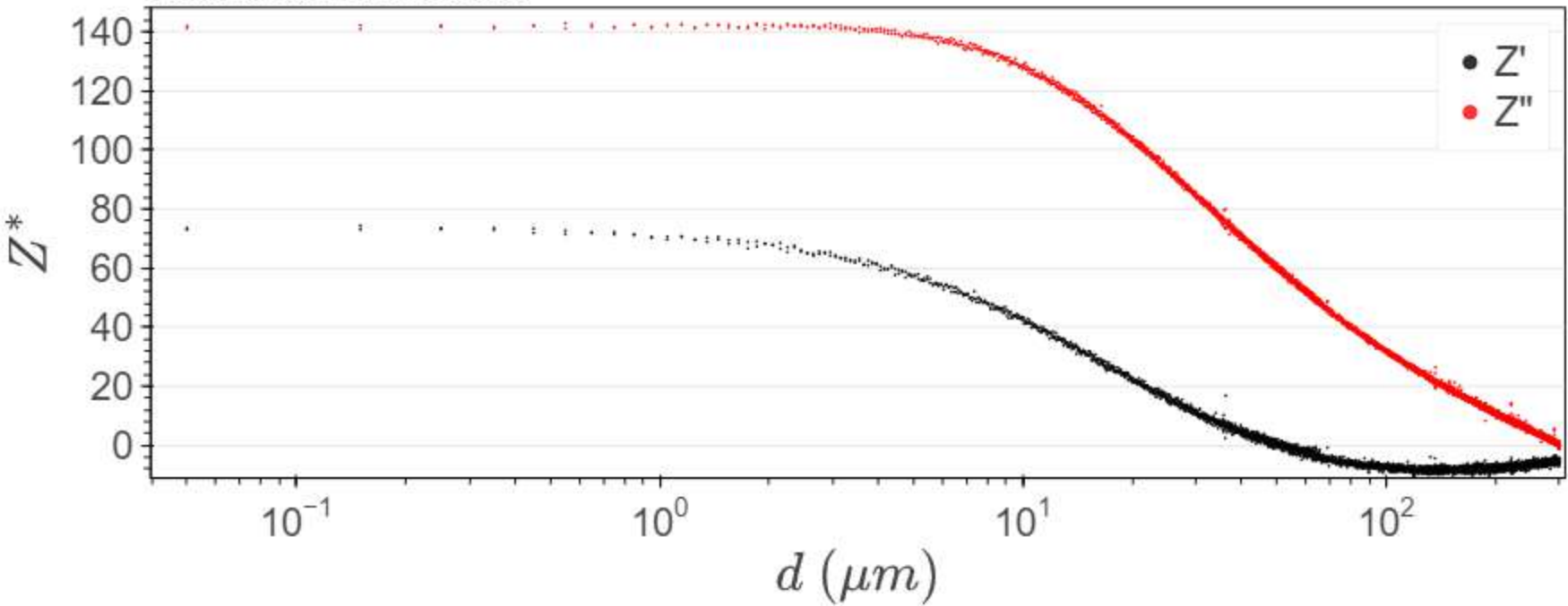
dioctylphthalate on PDMS glass sphere
