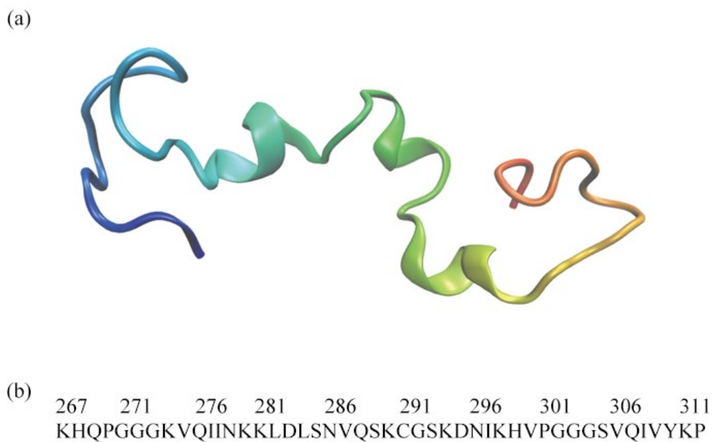
Fig. S1 Schematic ribbon diagrams of a. Tau(2MZ7) and b. primary sequence of the protein.
