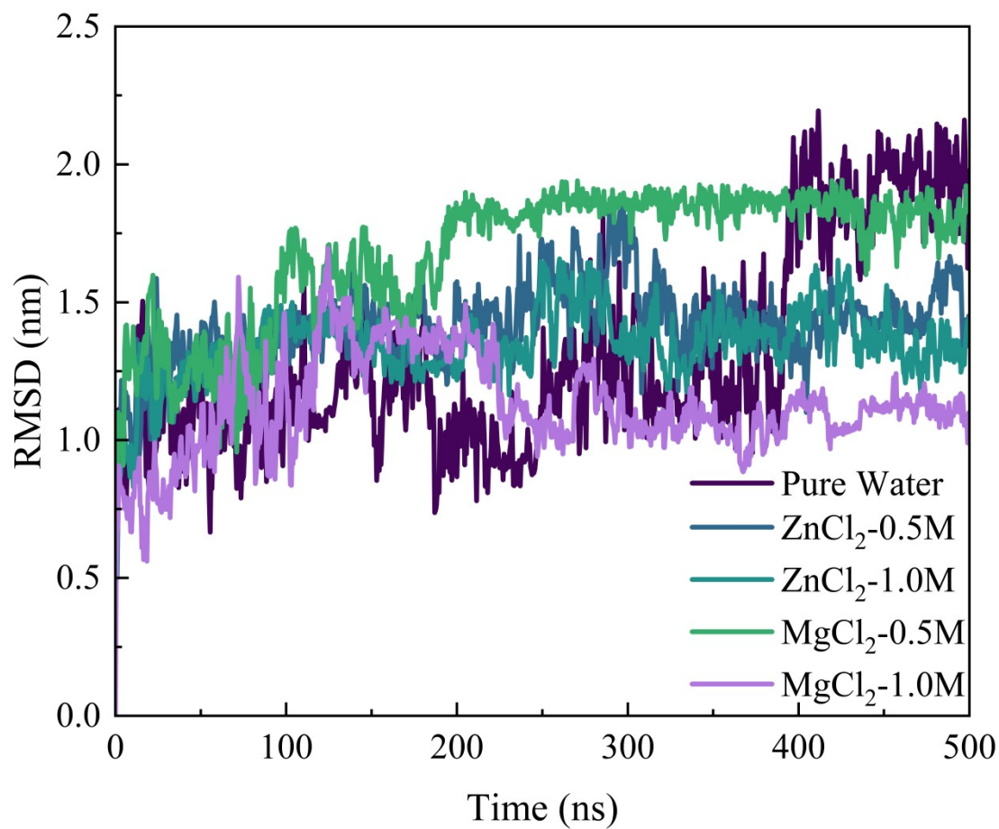
Fig. S2 Stability and rigidity of Tau protein. The RMSD values of each system.
