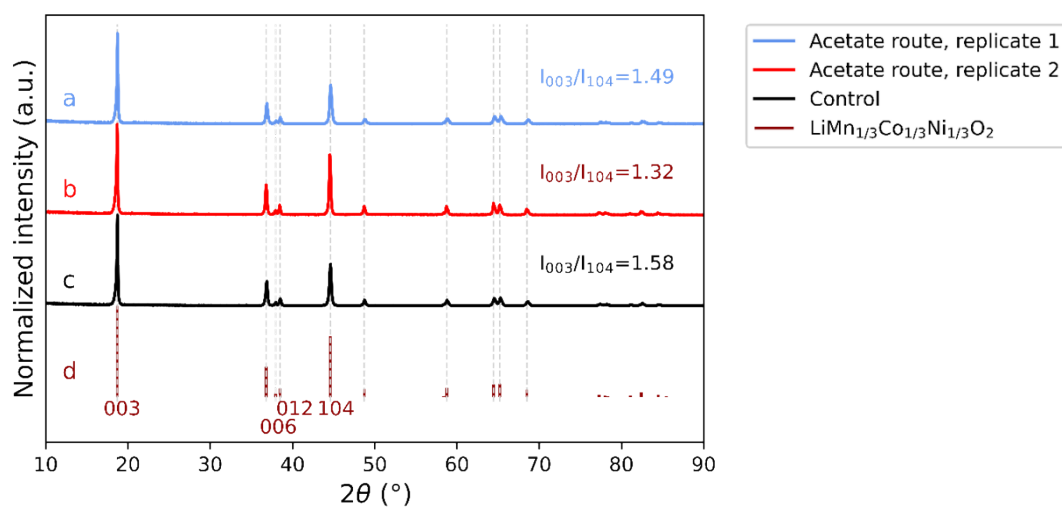
Figure S1. Normalized X-ray diffraction pattern from 10 to 90° 2\theta for samples from the acetate route with (a) replicate 1, (b) replicate 2 and (c) a control NMC111 sample. In (d) diffraction peaks of NMC111 (ICDD: 04-014-7636) with indexation of relevant peaks are shown.
