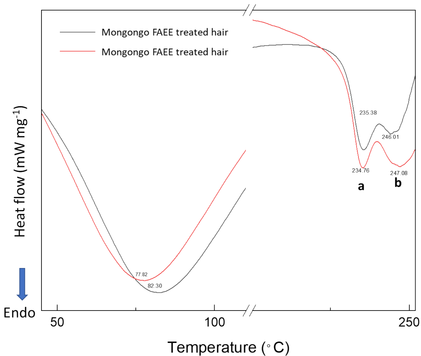
Figure S2. Comparison of DSC of hair treated with Mongongo FAEE and Mongongo oil.
