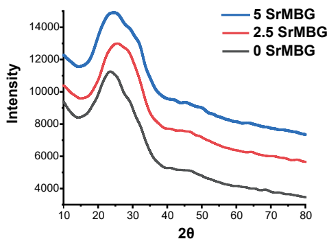
Supplementary figure 1 XRD analysis of SrMBG powder.
