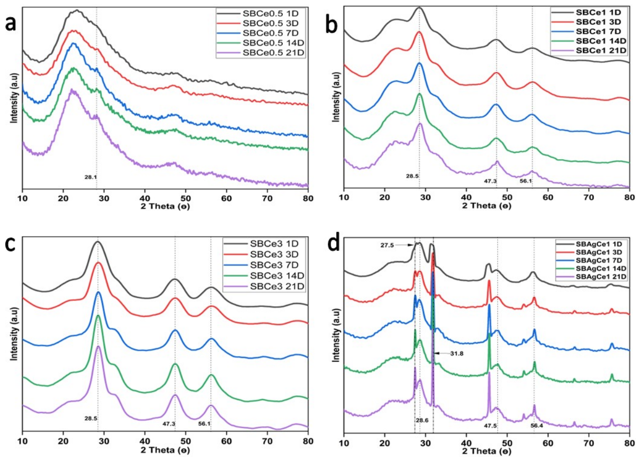
Supplementary Figure 2. XRD spectra of Incubated doped BGGs for 1,3,7,14 and 21 days (a) SBCE0.5, (b) SBCE1, (c) SBCE3 and (d) SBAgCe1
