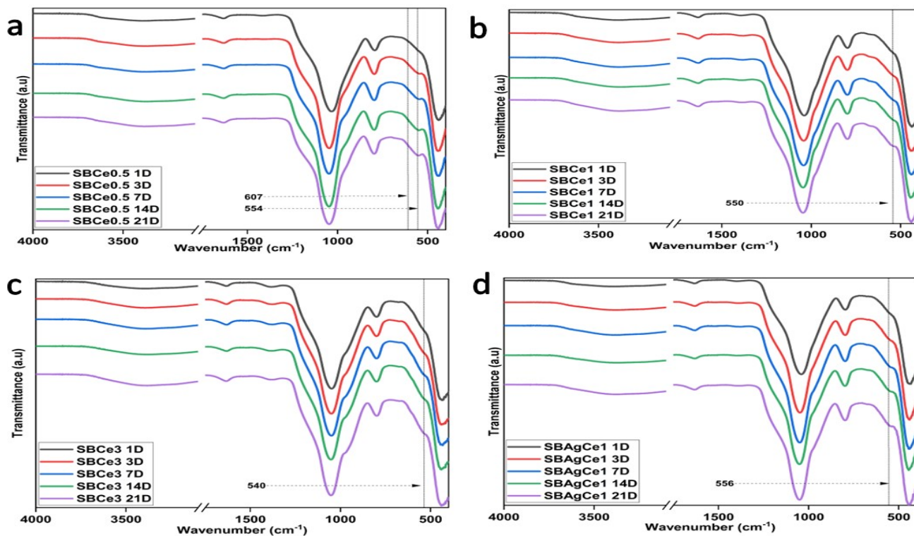
Supplementary Figure 1. FTIR spectra of Incubated doped BBGs for 1,3,7,14 and 21 days (a) SBCe0.5, (b) SBCe1, (c)SBCe3 and (d)SBAgCe1
