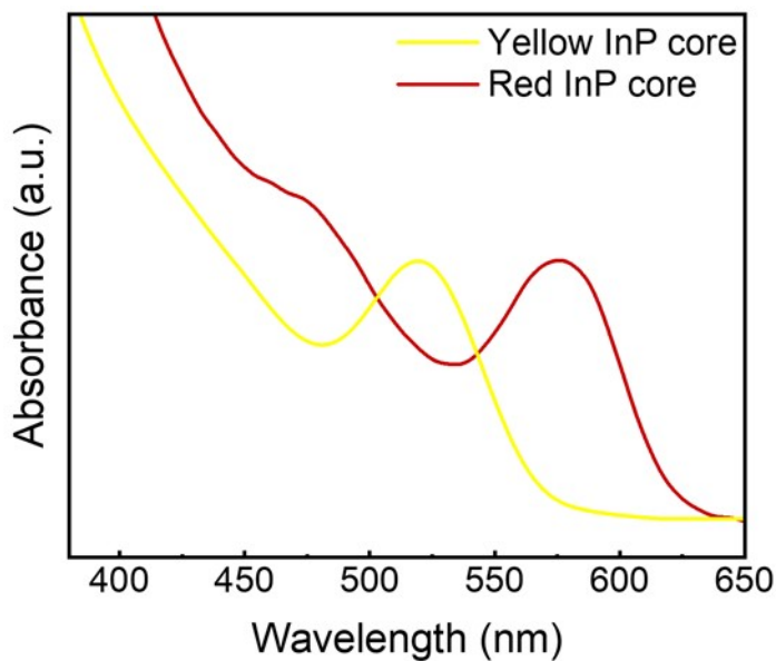
Figure S1. UV-visible absorption spectra of InP cores of yellow and red QDs.
