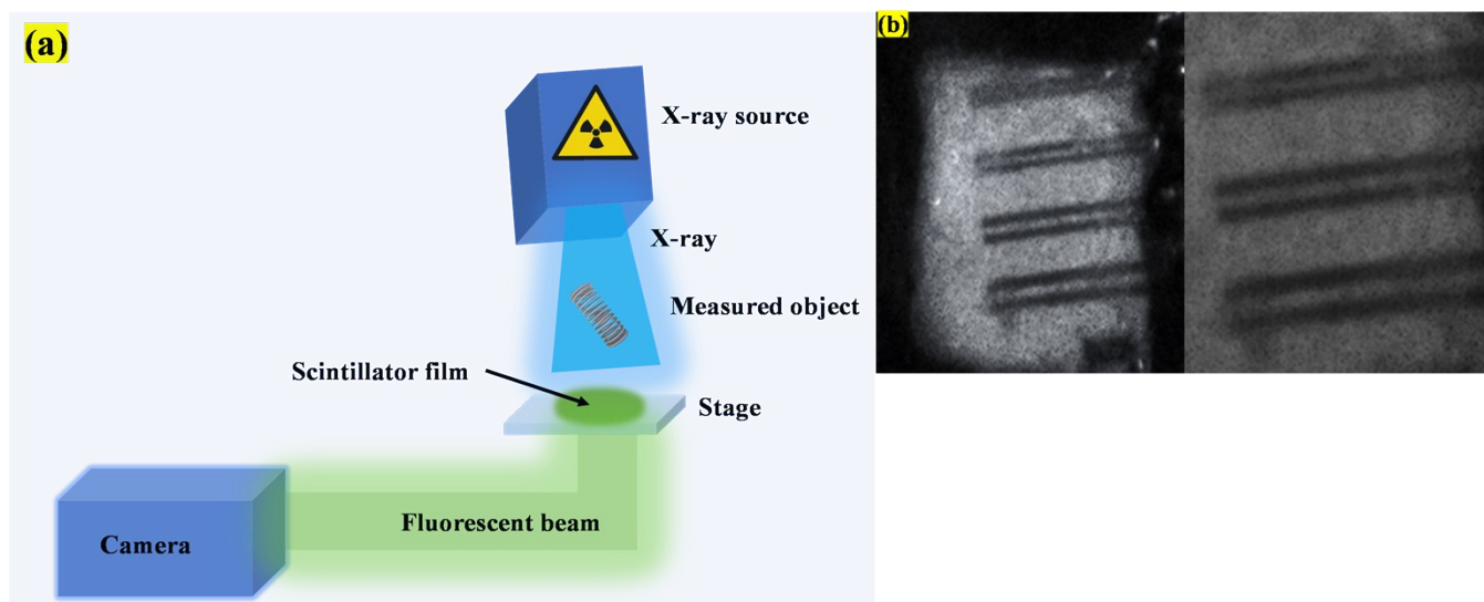
Fig. 10 (a) X-ray radiography setup consisting of X-ray source, object, CCD camera, and the composite screen (b) image formed by a duplex wire with a resolution of 100 microns.
