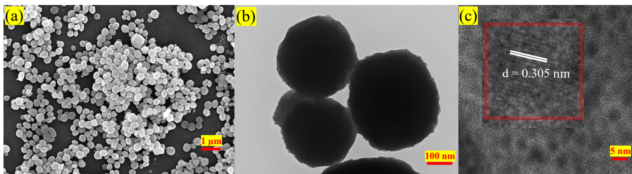
Fig. 2 (a) FE-SEM, (b) TEM (c) HRTEM images of the NBF: Gd, Tb nanoparticles.
