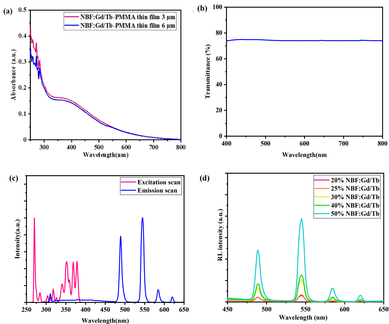
Fig. 8 (a) Absorption spectra of PMMA-NBF film of thickness 3 and 6 \mu\text{m} ; (b) transmission spectra of PMMA-NBF film (c) excitation and PL spectra of PMMA-NBF film (d) XEOL spectra of PMMA-NBF with different loading percentages.
