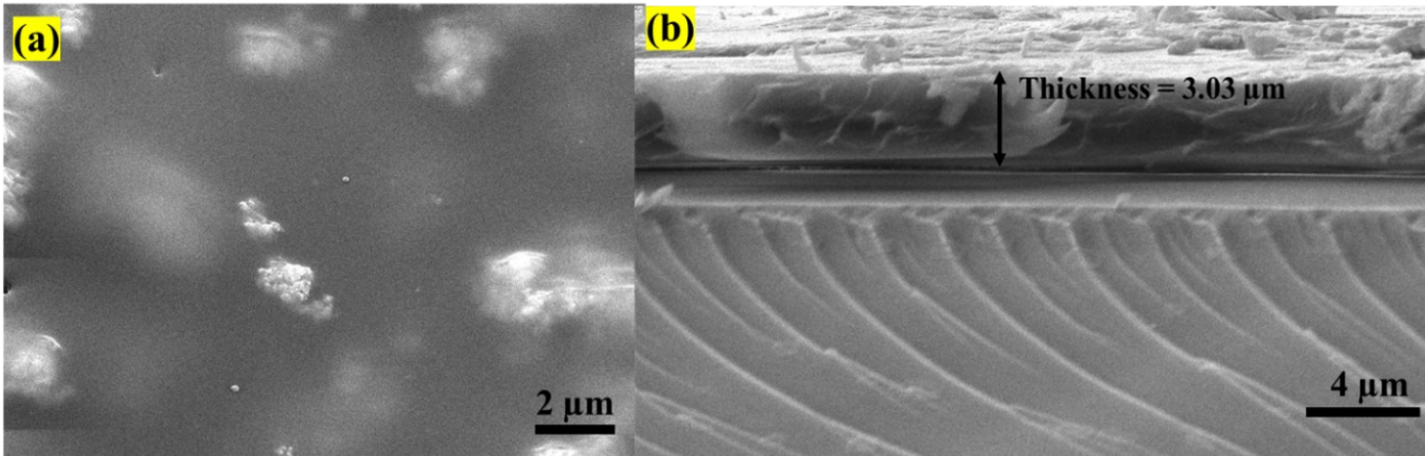
Fig. 7 (a) FESEM image of PMMA-NBF film (b) Cross-sectional FE-SEM image of a PMMA-NBF thin film.
