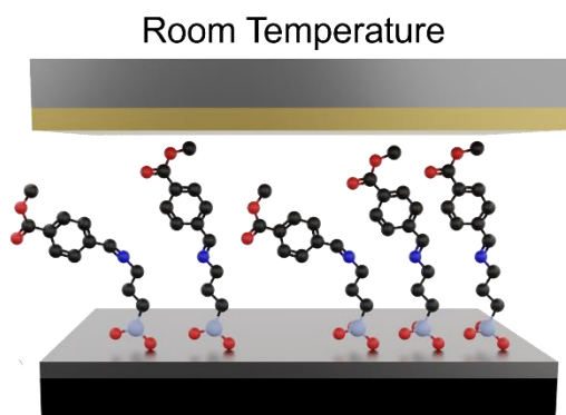
Fig S1. Illustrations of different molecular configurations of SAMs at room temperature (a) and at low temperature (b) due to entropic effects.
