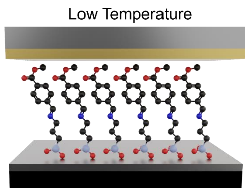
Fig S1. Illustrations of different molecular configurations of SAMs at room temperature (a) and at low temperature (b) due to entropic effects.
