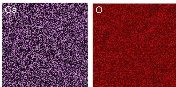
Figure S2. SEM-EDX mapping of Ga 2 O 3 film at a scale of 100 μm × 100 μm.
