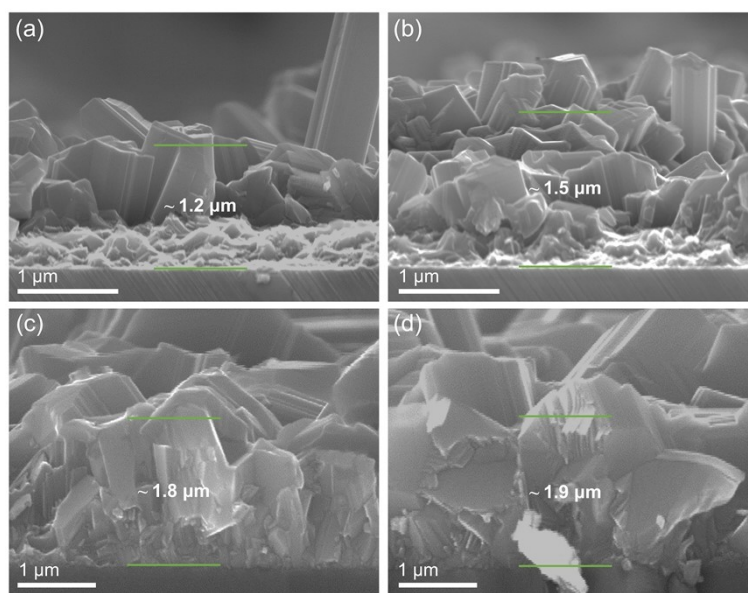
Figure S1. Cross-sectional SEM images of Ga 2 O 3 films prepared at different heating rates during thermal oxidation. (a) 20 °C/min, (b) 10 °C/min, (c) 5 °C/min, and (d) 2 °C/min.
